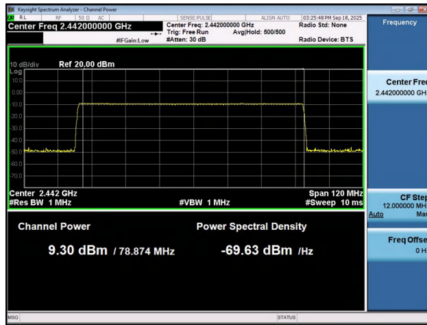
NTNV-DH5-Ant1-Hop-PASS
