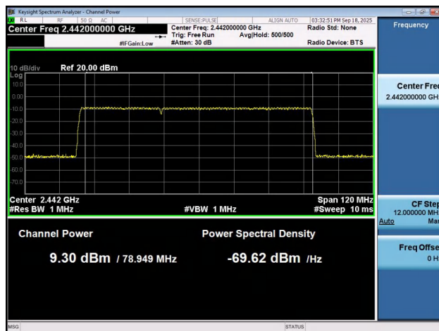
NTNV-3DH5-Ant1-Hop-PASS
