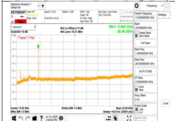
LPI 802.11ax 160MHz Chain0 6345MHz Range2
