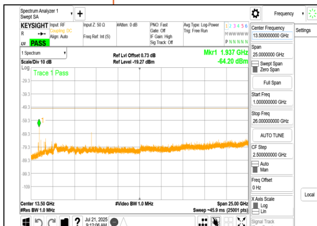
LPI 802.11ax 160MHz Chain1 6345MHz Range2
