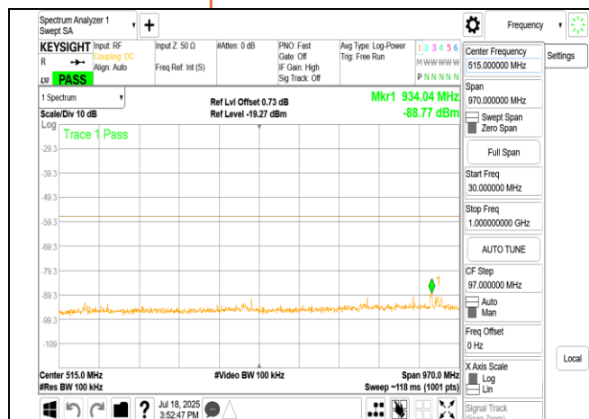
LPI 802.11ax 20MHz Chain0 6415MHz Range1
