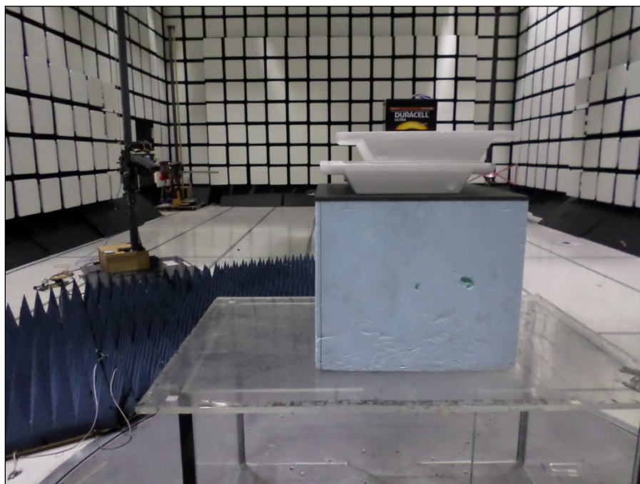
Photograph 8. Radiated Emissions, Above 1 GHz, Rear
