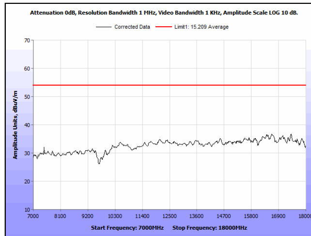
Plot 12. Radiated Emissions, 7 GHz – 18 GHz, Horizontal, Average
