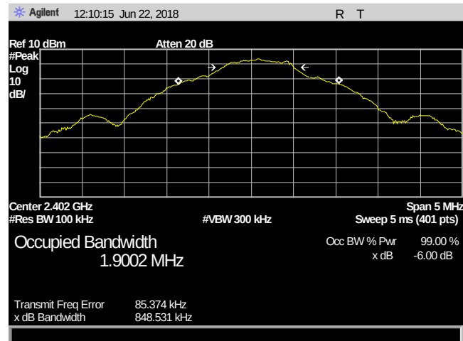
Plot 24. 6 dB Occupied Bandwidth, 2402
