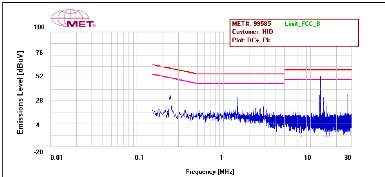
Plot 1. Conducted Emissions, DC+
