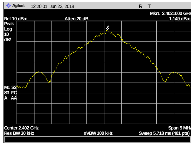
Plot 27. Power Density, 2402
