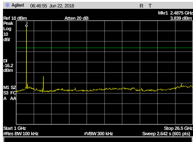
Plot 20. Conducted Spurious Emissions, 2480, 1 – 26.5 GHz
