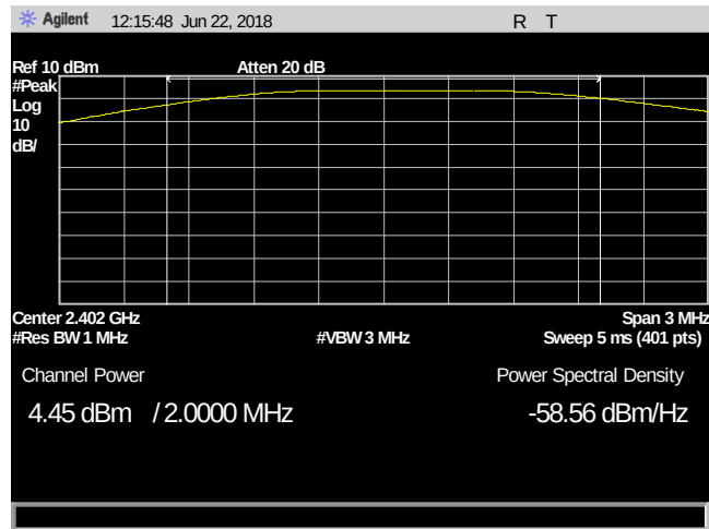
Plot 3. Peak Power Output, 2402
