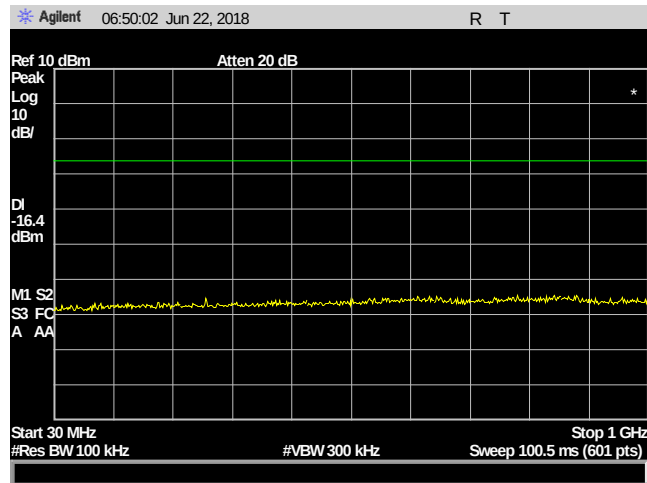
Plot 19. Conducted Spurious Emissions, 2442, 30 MHz – 1 GHz
