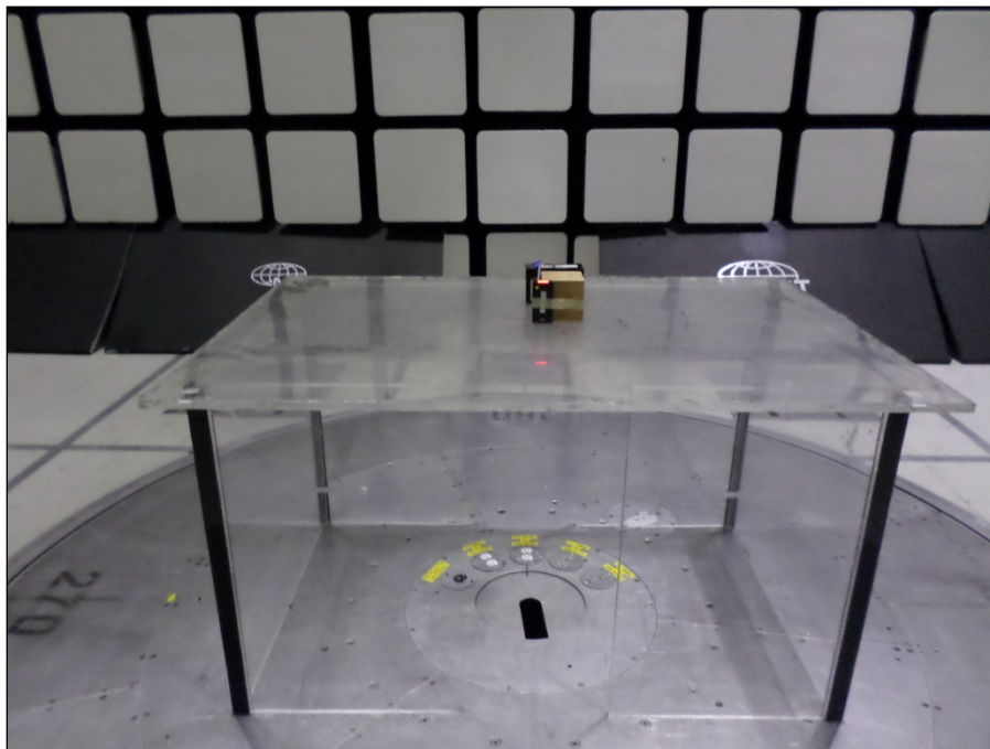
Photograph 4. Radiated Emissions, Below 1 GHz, Front
