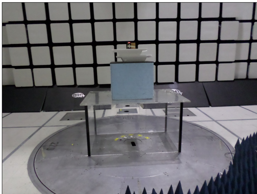
Photograph 7. Radiated Emissions, Above 1 GHz, Front
