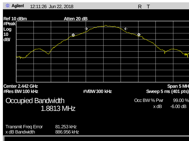
Plot 25. 6 dB Occupied Bandwidth, 2442
