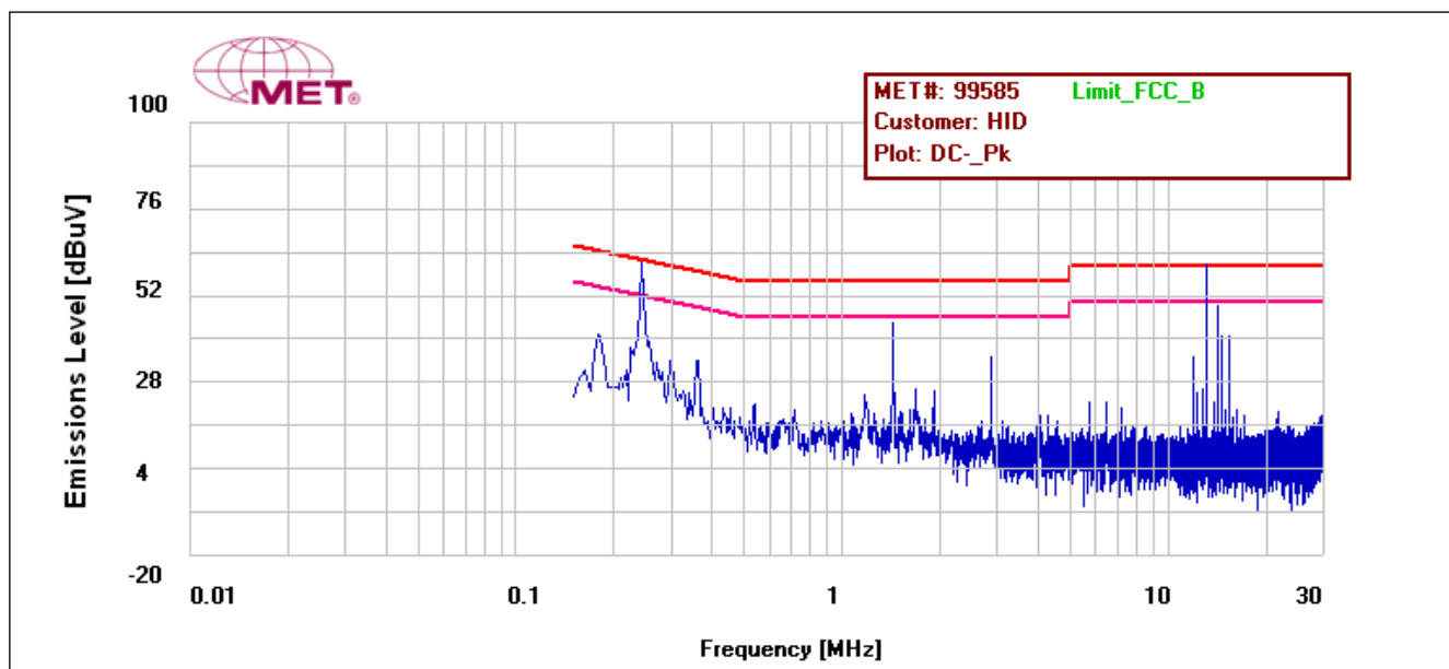
Plot 2. Conducted Emissions, DC-
