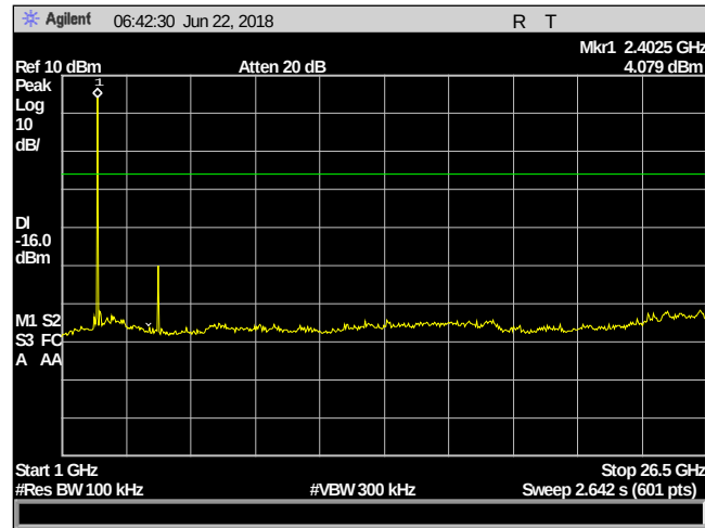
Plot 16. Conducted Spurious Emissions, 2402, 1 – 26.5 GHz
