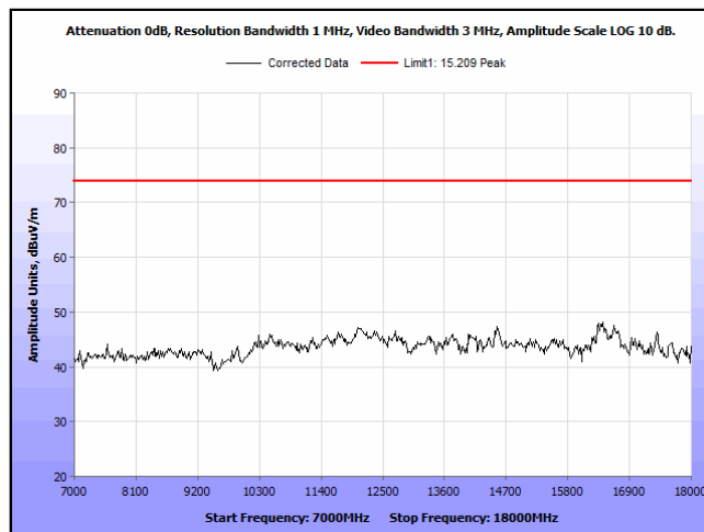
Plot 15. Radiated Emissions, 7 GHz – 18 GHz, Vertical, Peak
