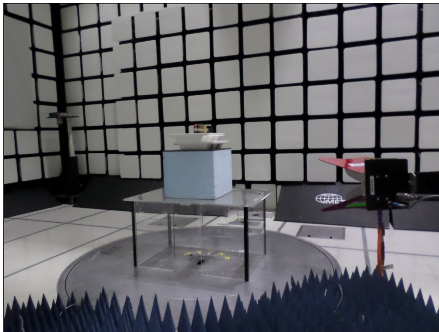
Photograph 6. Radiated Emissions, Above 1 GHz, Antenna
