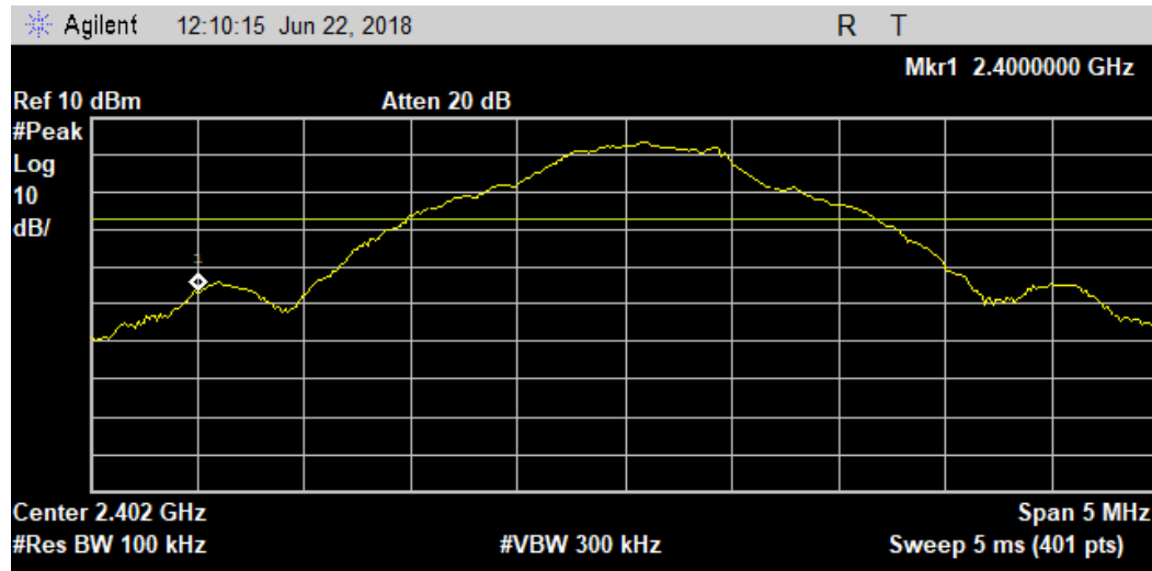
Plot 22. Conducted Spurious Emissions, 2402, Bandedge
