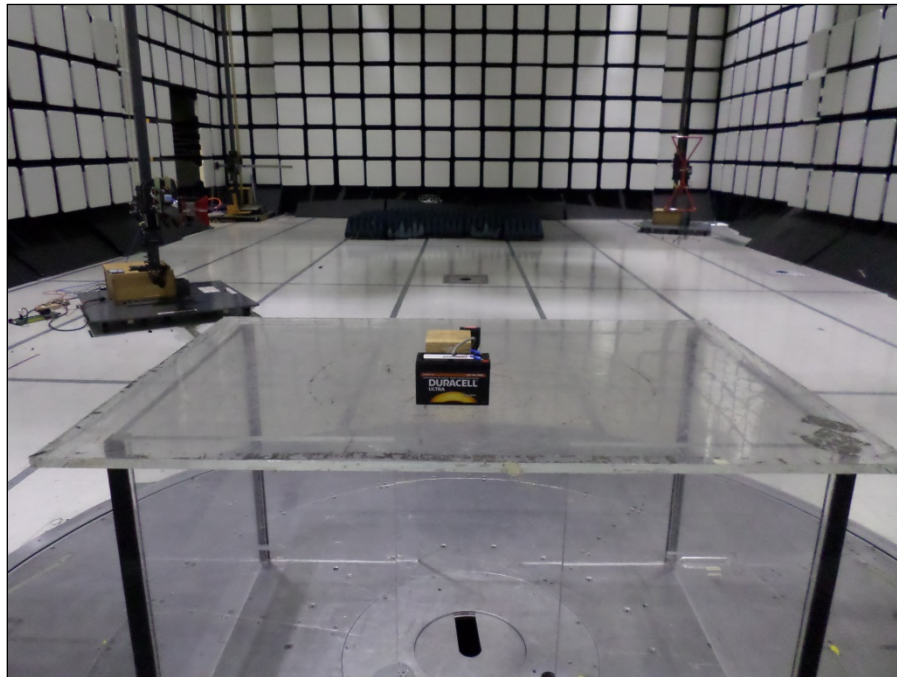
Photograph 5. Radiated Emissions, Below 1 GHz, Rear
