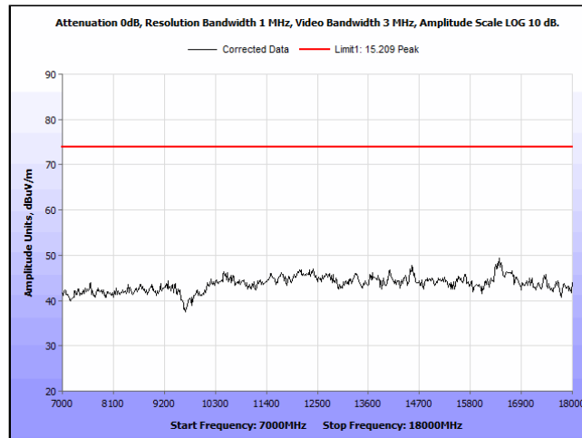
Plot 13. Radiated Emissions, 7 GHz – 18 GHz, Horizontal, Peak
