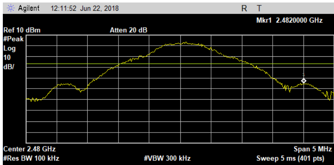
Plot 23. Conducted Spurious Emissions, 2480, Bandedge
