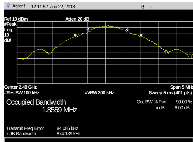
Plot 26. 6 dB Occupied Bandwidth, 2480
