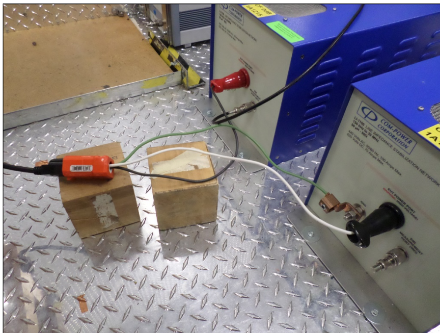
Photograph 2. Conducted Emissions, LISN Setup
