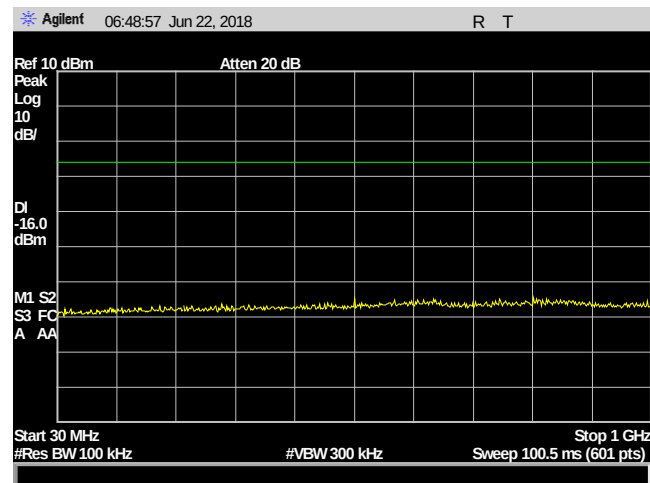
Plot 17. Conducted Spurious Emissions, 2402, 30 MHz – 1 GHz
