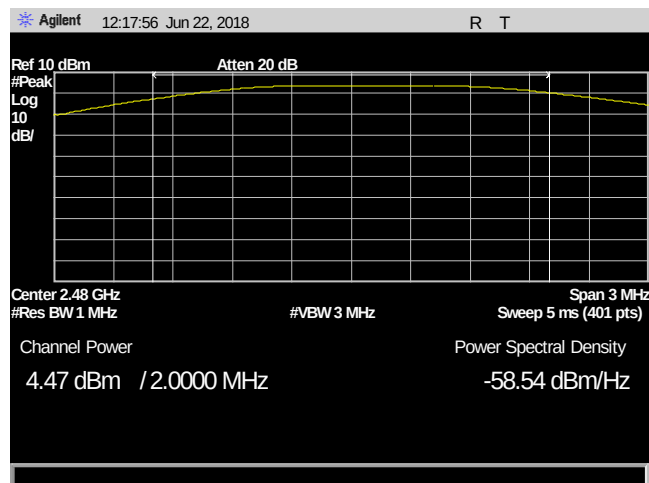
Plot 5. Peak Power Output, 2480
