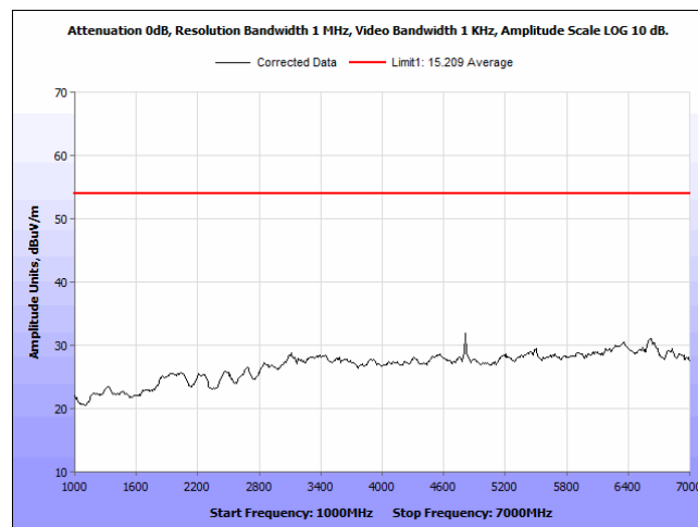
Plot 8. Radiated Emissions, 1 GHz – 7 GHz, Horizontal, Average
