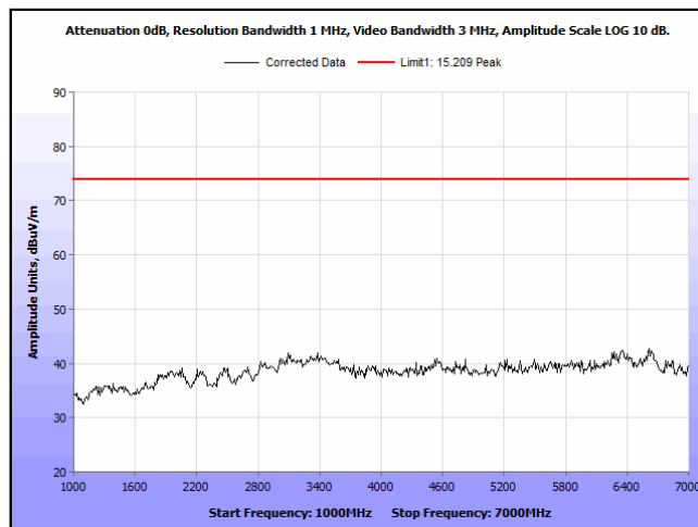
Plot 9. Radiated Emissions, 1 GHz – 7 GHz, Horizontal, Peak
