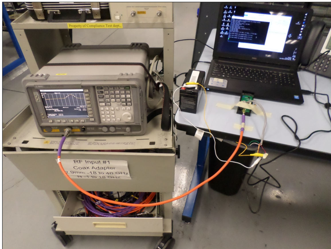
Photograph 9. Conducted Testing Setup
