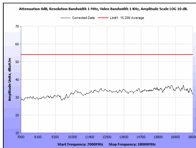
Plot 14. Radiated Emissions, 7 GHz – 18 GHz, Vertical, Average
