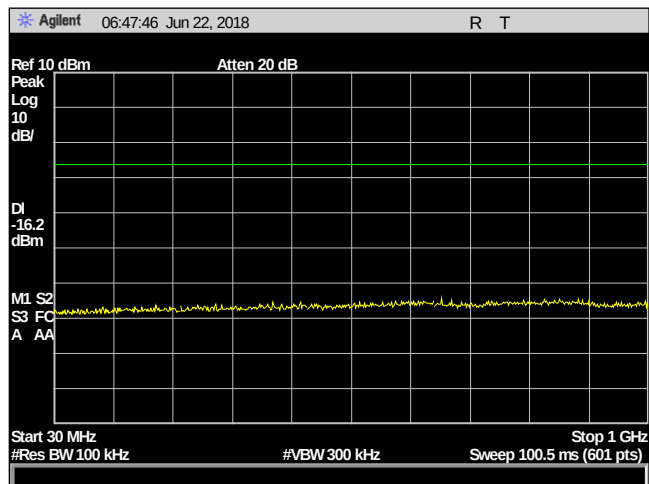
Plot 21. Conducted Spurious Emissions, 2480, 30 MHz – 1 GHz
