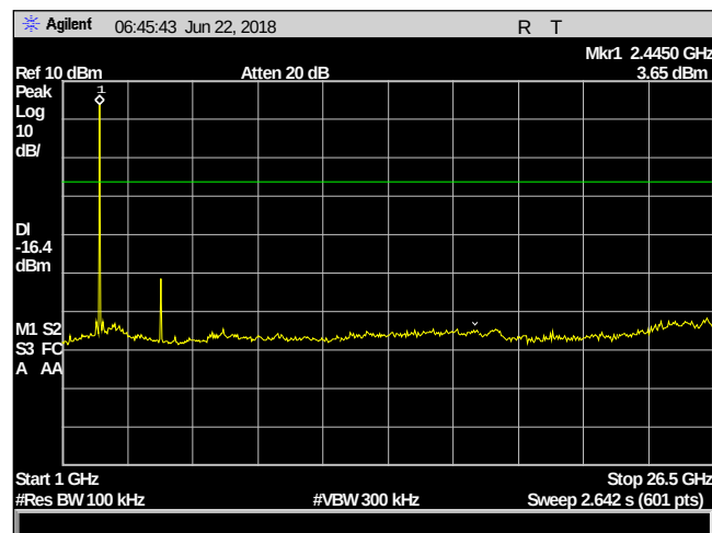
Plot 18. Conducted Spurious Emissions, 2442, 1 – 26.5 GHz
