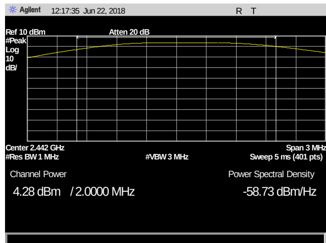
Plot 4. Peak Power Output, 2442
