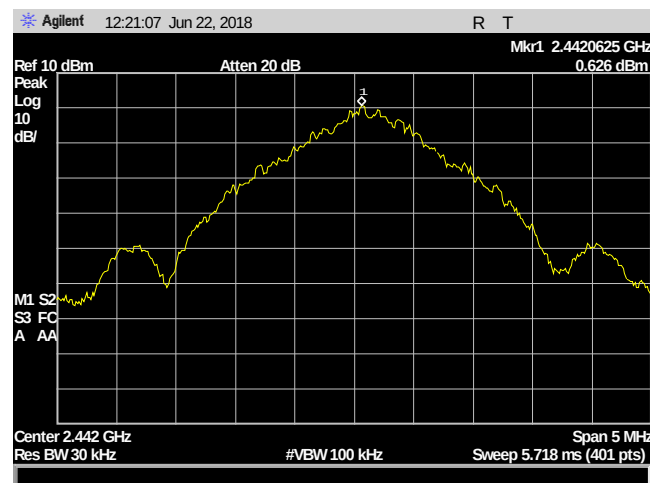
Plot 28. Power Density, 2442
