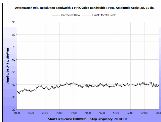
Plot 11. Radiated Emissions, 1 GHz – 7 GHz, Vertical, Peak
