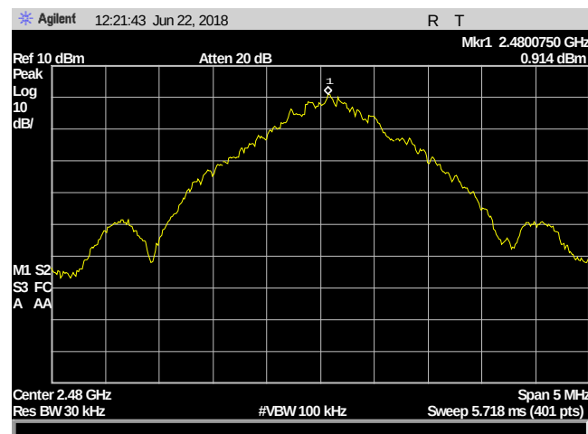
Plot 29. Power Density, 2480
