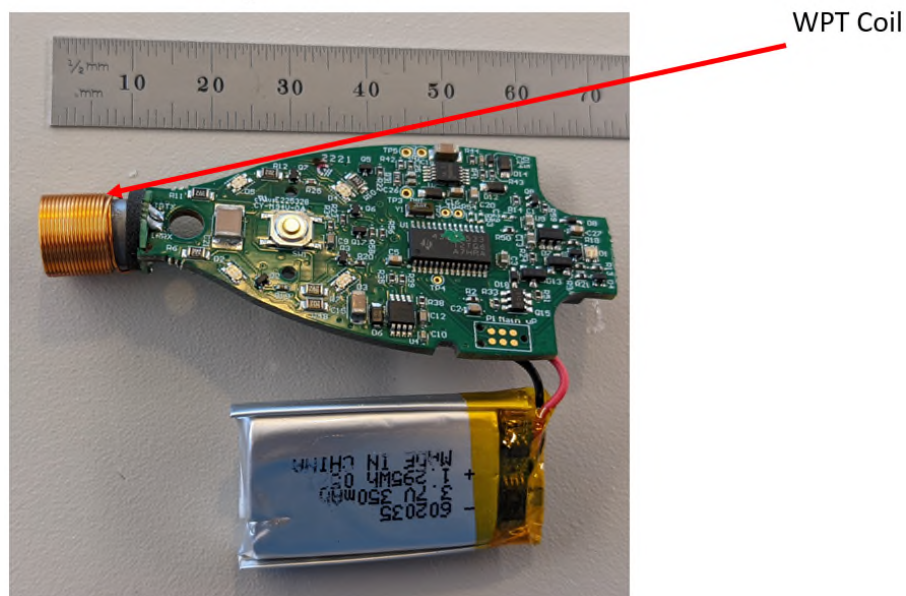
Photo 1.4-1 – Top View of the PCB
