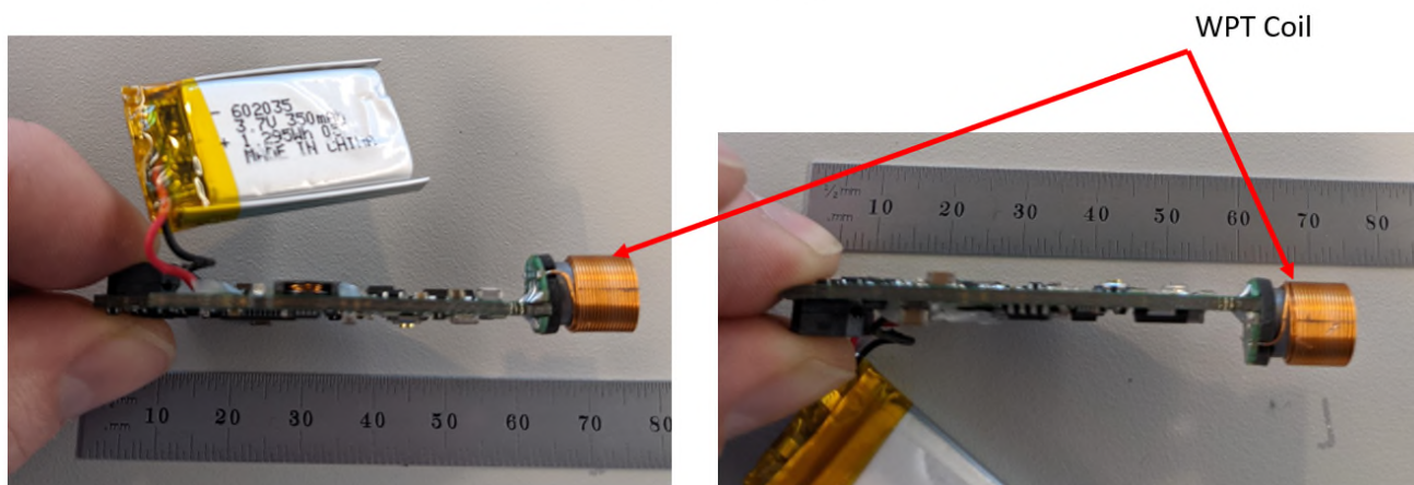
Photo 1.4-4 – Side Views of the PCB
