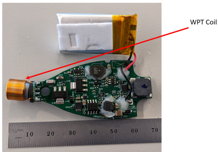
Photo 1.4-2 – Bottom View of the PCB
