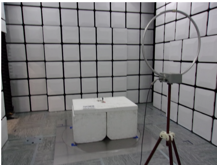
Photo 2.1-1 – Front View of the Test Setup up to 1 GHz
