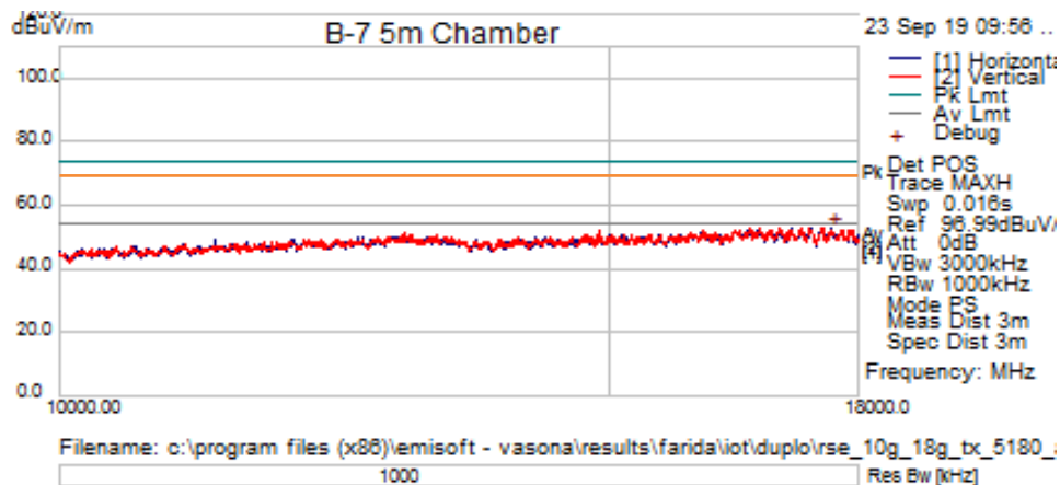
Title: TX Spurious Emissions from 10GHz-18GHz – Ch36 (5180 MHz)
