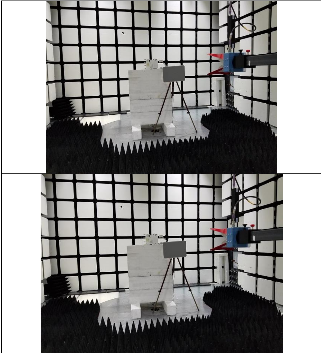
Title: Radiated Spurious Emissions 1GHz-18GHz – Test Setup
