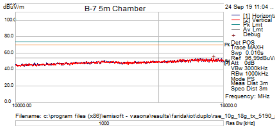
Title: TX Spurious Emissions from 10GHz-18GHz – Ch38 (5190 MHz)
