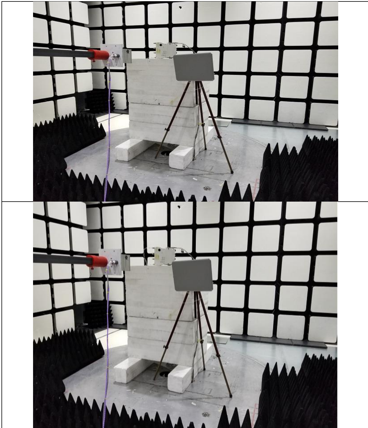
Title: Radiated Spurious Emissions 18GHz-40GHz – Test Setup
