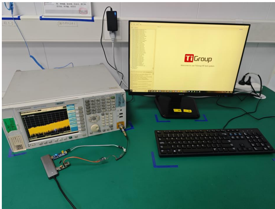
Conducted Test-Left Ear
