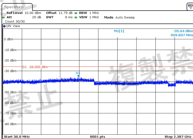
NTNV-2.4G_MIMO_10M-Ant1-2466-30~2387-PASS
