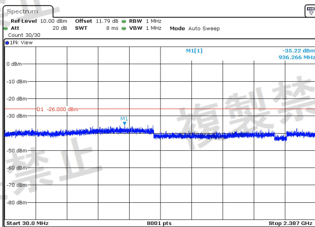
NTNV-2.4G_MIMO_20M-Ant1-2466-30~2387-PASS
