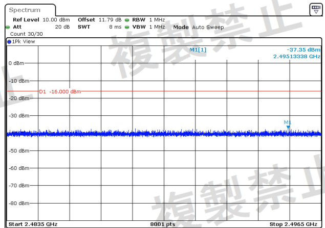
NTNV-2.4G_MIMO_20M-Ant2-2411-2483.5~2496.5-PASS
