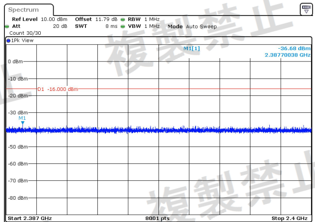
NTNV-2.4G_MIMO_20M-Ant2-2444-2387~2400-PASS
