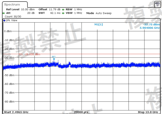
NTNV-2.4G_MIMO_20M-Ant2-2444-30~2387-PASS
