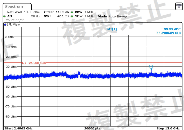
NTNV-2.4G_MIMO_20M-Ant2-2466-2496.5~13000-PASS
