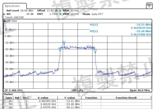
NTNV-2.4G_MIMO_10M-Ant2-2466-PASS
