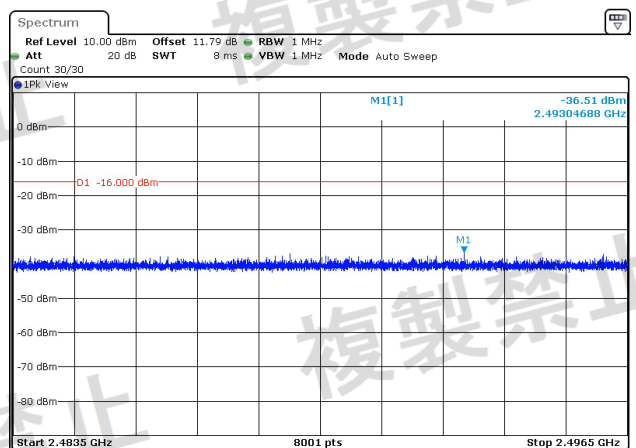
NTNV-2.4G_MIMO_10M-Ant2-2411-2483.5~2496.5-PASS
