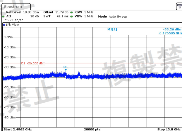
NTNV-2.4G_MIMO_10M-Ant1-2466-2496.5~13000-PASS
