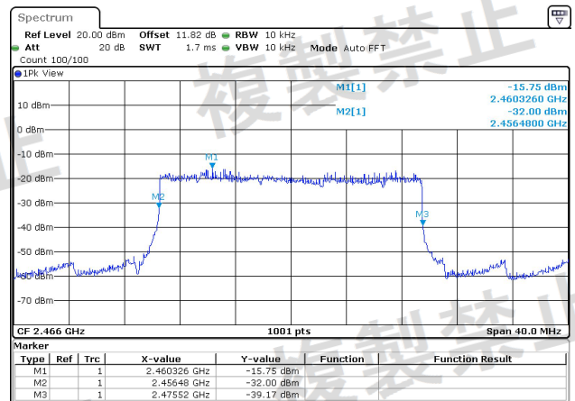
NTNV-2.4G_MIMO_20M-Ant2-2466-PASS
