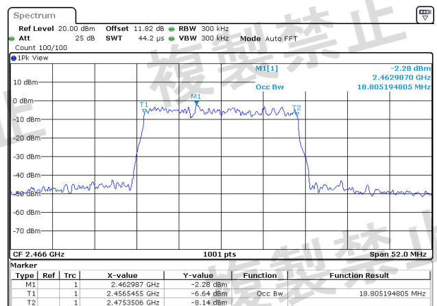
NTNV-2.4G_MIMO_20M-Ant2-2466-PASS
