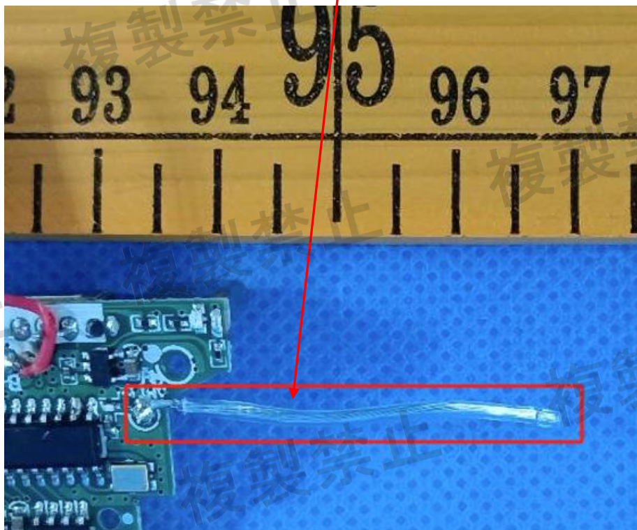
wireless antenna
