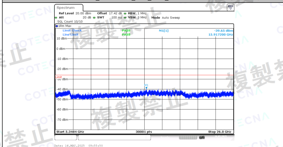
NTLV_11N40SISO_Ant1_5270_5350~5348.4
