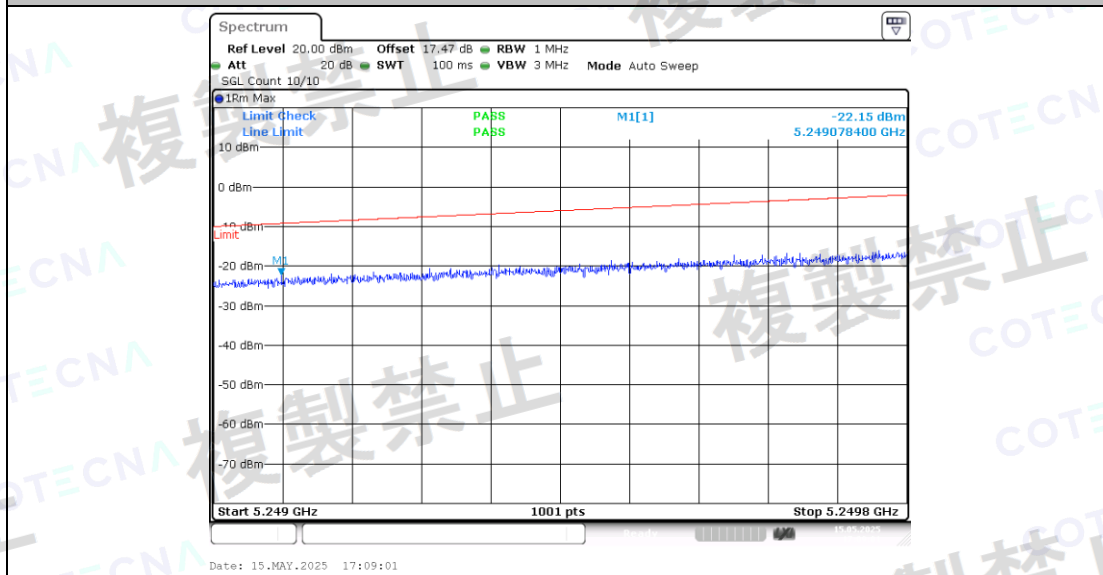
NTLV_11N20SISO_Ant1_5260_5249.8~5250
