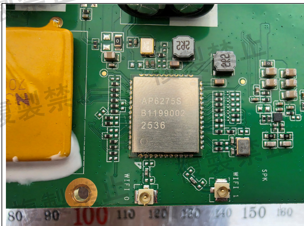
< Wifi module >
