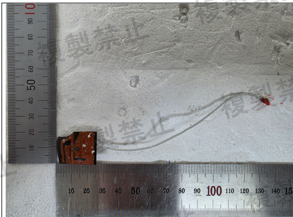
< Wifi Antenna 1 >
