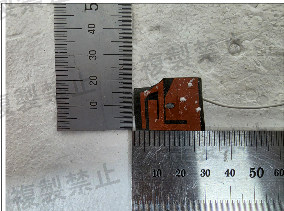
< Wifi Antenna 1 >
