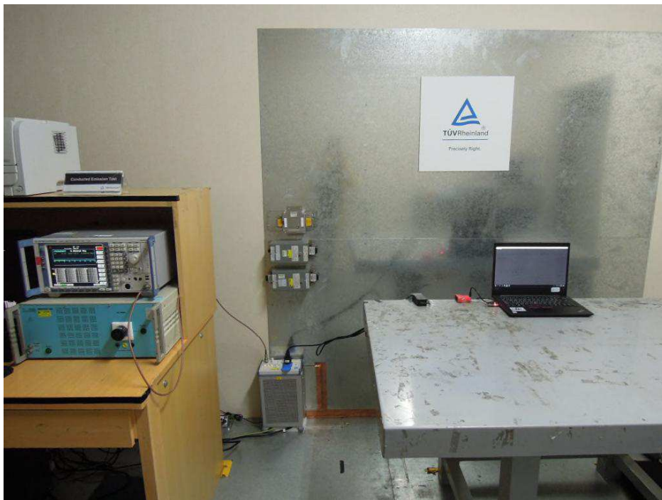
Photograph 9: Set-up for Mains Conducted testing (Front View)
