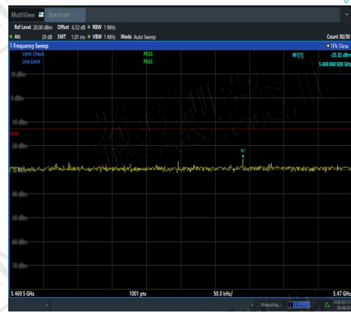
NTVN-11AC80MIMO-Ant2-5530-5469.5~5470-P ASS
