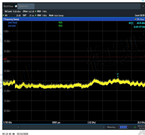
NTVN-11AX20SISO-Ant1-5700-5765~26000-PA SS
