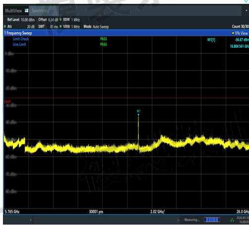
NTNV-11AX20SISO-Ant2-5600-5765~26000-PA
