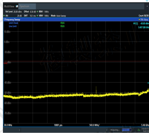
NTNV-11AC40SISO-Ant1-5550-30~5460-PASS
