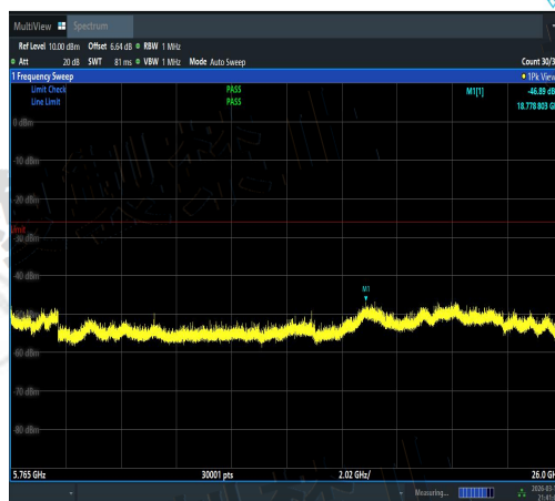
NTNV-11AX20MIMO-Ant3-5600-5765~26000-PA
