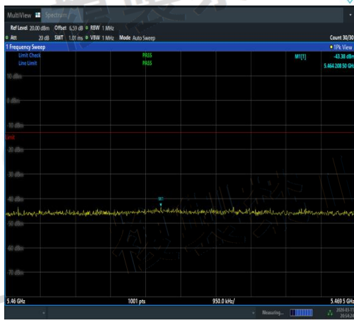
NTNV-11AC80MIMO-Ant2-5610-5460~5469.5-PASS
