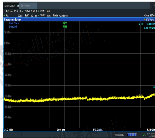
NTVN-11AC40MIMO-Ant2-5510-30~5460-PASS
