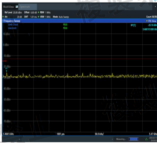
NTVN-11AC80MIMO-Ant1-5530-5469.5~5470-P ASS
