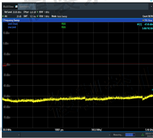
NTNV-11AC40MIMO-Ant2-5710-30~5460-PASS
