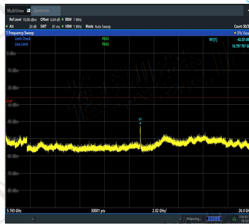
NTNV-11AX20SISO-Ant3-5600-5765~26000-PA
