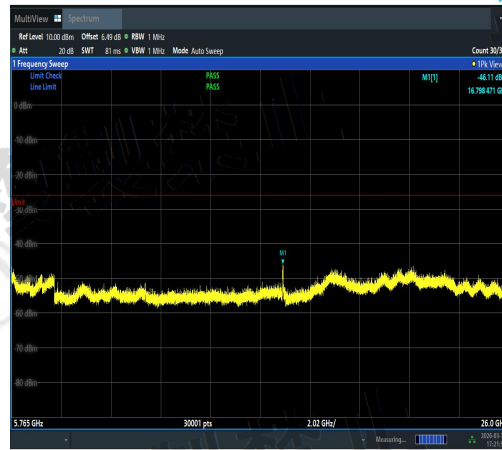
NTNV-11AX20SISO-Ant1-5600-5765~26000-PA
