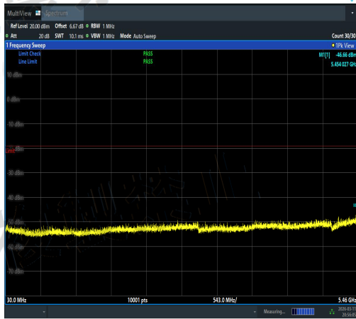
NTNV-11AC80MIMO-Ant3-5610-30~5460-PASS
