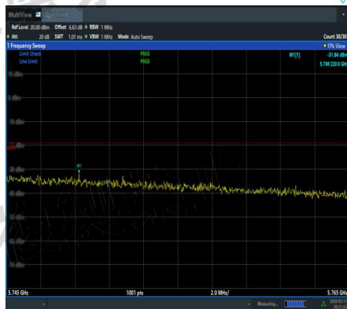
NTNV-11AC20MIMO-Ant3-5720-5745~5765-PAS
