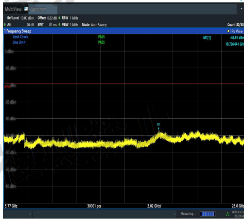
NTNV-11AC40MIMO-Ant3-5670-5770~26000-PA SS
