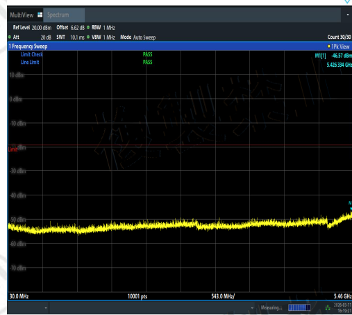
NTVN-11AC40SISO-Ant2-5670-30~5460-PASS
