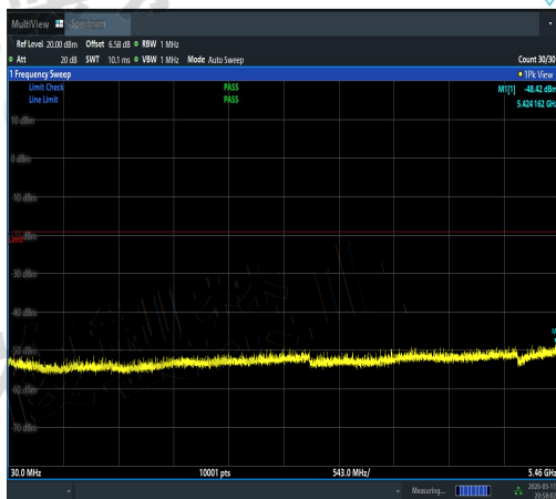
NTVN-11AC80MIMO-Ant1-5690-30~5460-PASS
