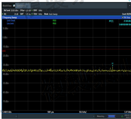
NTVN-11AC80MIMO-Ant1-5530-5469.5~5470-P ASS
