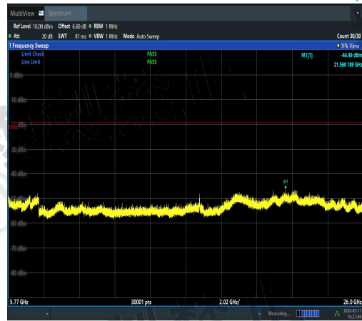
NTVN-11AC40SISO-Ant3-5550-5770~26000-PA SS
