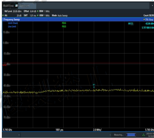
NTNV-11AX20SISO-Ant3-5600-5745~5765-PAS
