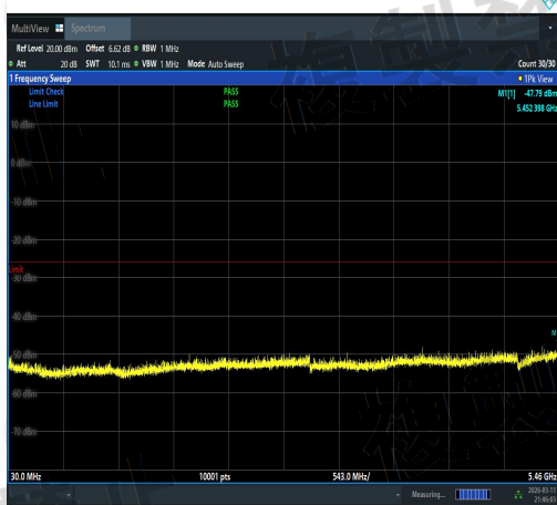
NTNV-11AX20MIMO-Ant3-5700-30~5460-PASS
