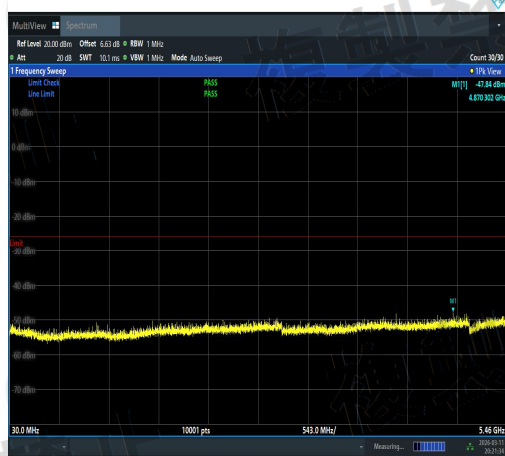
NTNV-11AC20MIMO-Ant3-5720-30~5460-PASS
