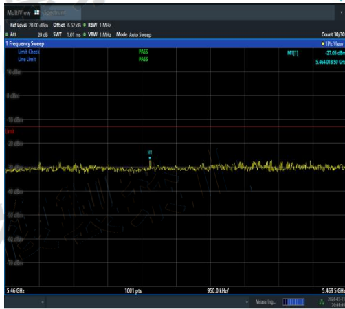
NTVN-11AC80MIMO-Ant2-5530-5460~5469.5-P ASS
