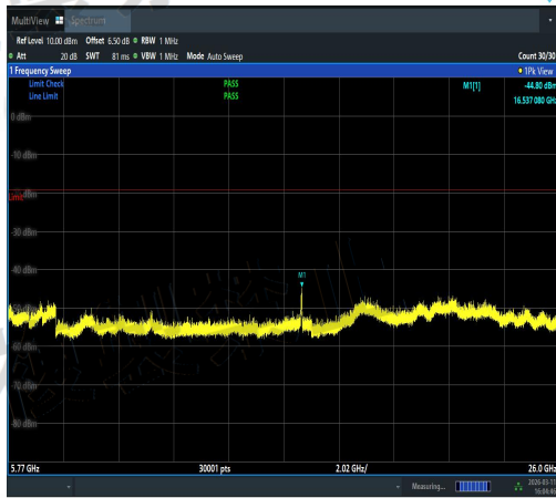
NTNV-11AC40SISO-Ant1-5510-5770~26000-PA SS
