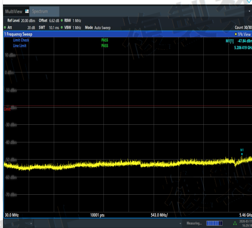
NTVN-11AC40SISO-Ant3-5670-30~5460-PASS
