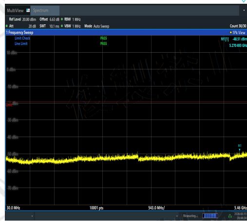
NTNV-11AC40MIMO-Ant3-5710-30~5460-PASS
