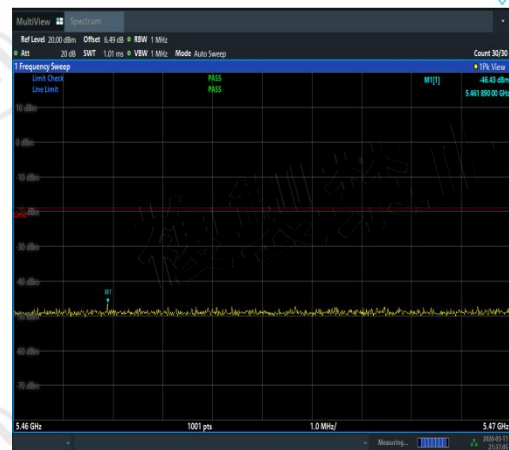
NTVN-11AX20MIMO-Ant1-5600-5460~5470-PASS
