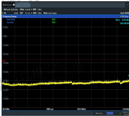
NTVN-11AC20MIMO-Ant1-5700-30~5460-PASS
