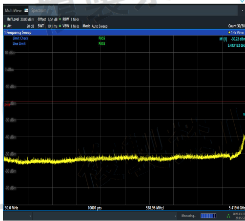
NTNV-11AC160MIMO-Ant2-5570-30~5419.6-PA SS
