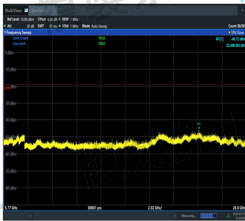
NTNV-11AC40SISO-Ant3-5510-5770~26000-PA SS
