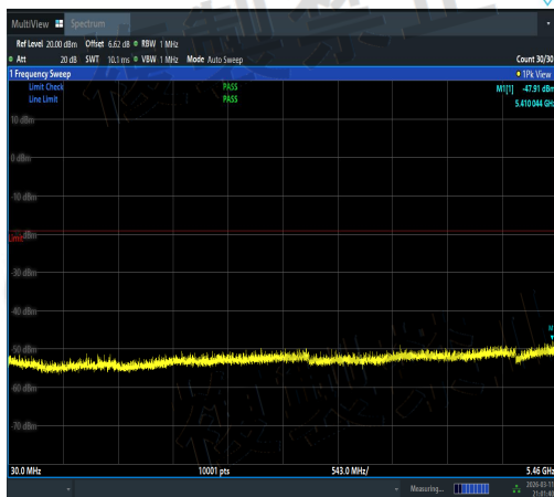
NTVN-11AC80MIMO-Ant3-5690-30~5460-PASS
