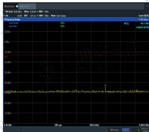
NTVN-11AC80MIMO-Ant1-5690-5460~5469.5-PASS
