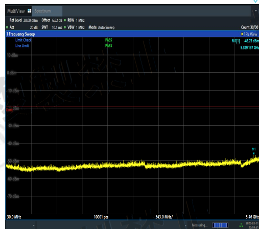
NTVN-11AC80MIMO-Ant2-5690-30~5460-PASS
