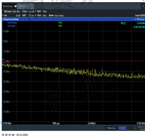
NTNV-11AX20SISO-Ant1-5720-5745~5765-See
