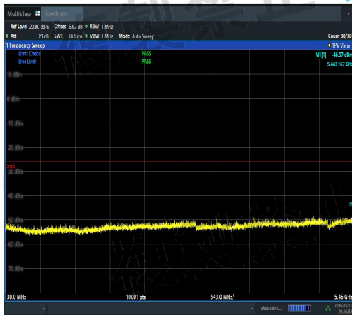
NTVN-11AC20MIMO-Ant3-5700-30~5460-PASS
