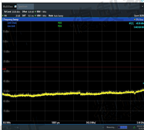
NTVN-11AX20SISO-Ant3-5600-30~5460-PASS
