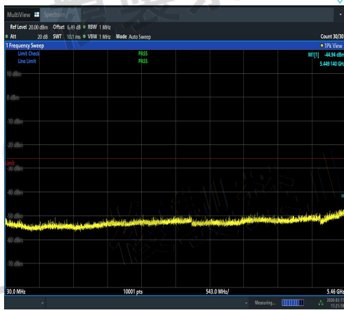
NTVN-11AX20SISO-Ant1-5600-30~5460-PASS
