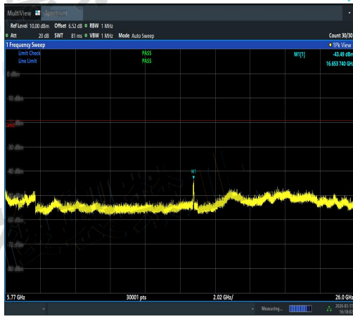
NTVN-11AC40SISO-Ant2-5550-5770~26000-PA SS
