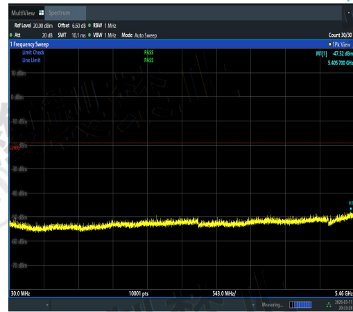
NTVN-11AC40MIMO-Ant3-5550-30~5460-PASS
