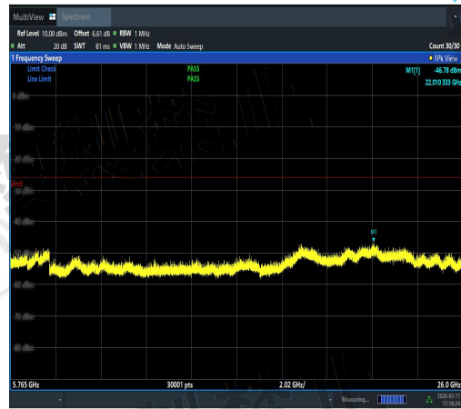
NTVN-11AX20SISO-Ant3-5500-5765~26000-PA SS
