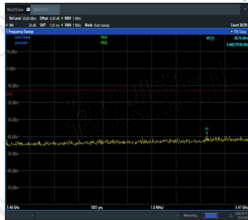
NTVN-11AC40MIMO-Ant1-5510-5460~5470-PASS
