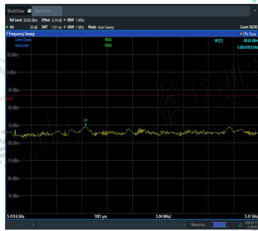
NTNV-11AC160MIMO-Ant3-5570-30~5419.6-PA SS
