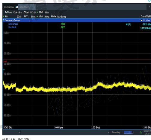
NTNV-11AC20MIMO-Ant2-5720-5765~26000-PA
