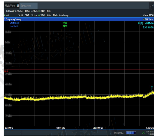
NTVN-11AX20MIMO-Ant2-5600-30~5460-PASS
