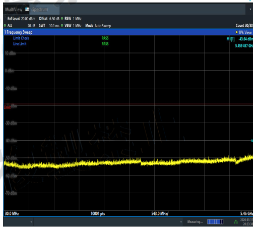
NTVN-11AC40MIMO-Ant1-5510-30~5460-PASS
