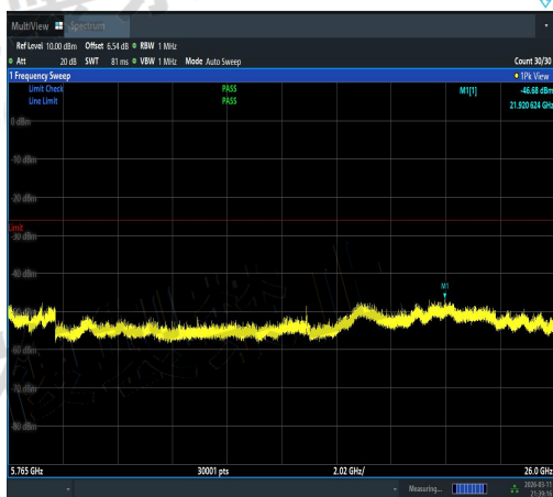
NTNV-11AX20MIMO-Ant2-5600-5765~26000-PA
