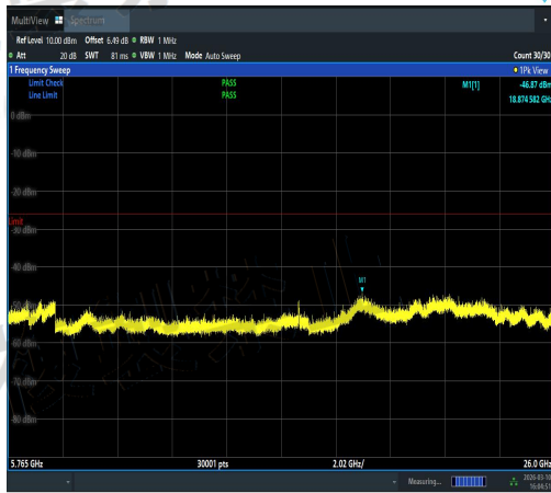
NTVN-11AX20SISO-Ant2-5500-5765~26000-PA SS
