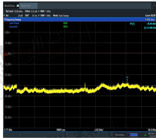
NTNV-11AC40SISO-Ant2-5510-5770~26000-PA SS
