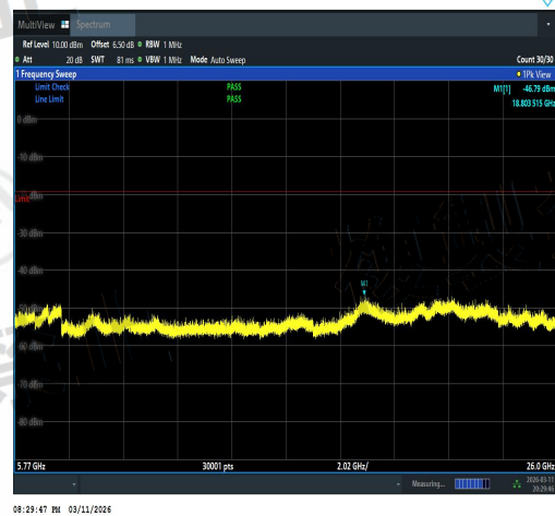
NTVN-11AC40MIMO-Ant1-5550-5770~26000-PA
