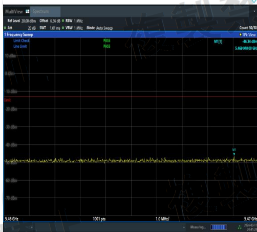
NTNV-11AC40MIMO-Ant1-5710-5460~5470-PAS
