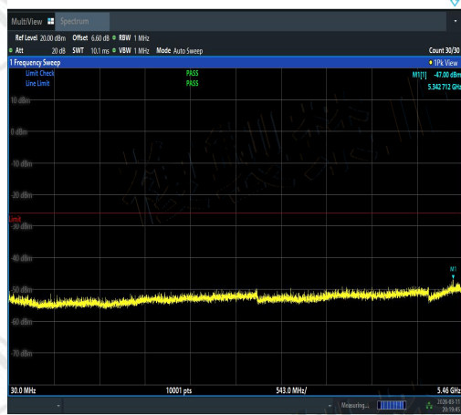
NTNV-11AC20MIMO-Ant2-5720-30~5460-PASS
