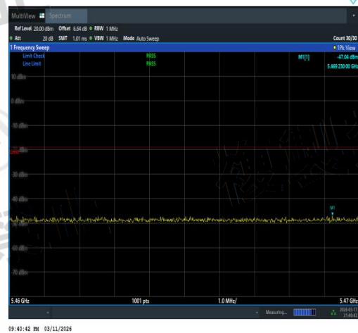
NTVN-11AX20MIMO-Ant3-5600-5460~5470-PASS
