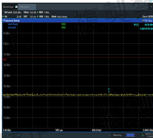
NTVN-11AC80MIMO-Ant2-5690-5460~5469.5-P
