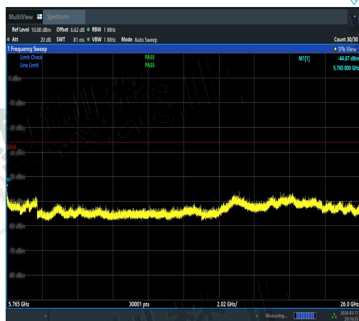
NTNV-11AC20MIMO-Ant3-5700-5765~26000-PA
