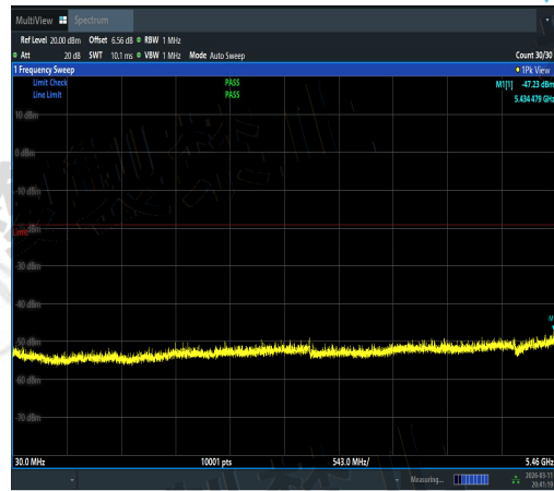
NTNV-11AC40MIMO-Ant1-5710-30~5460-PASS
