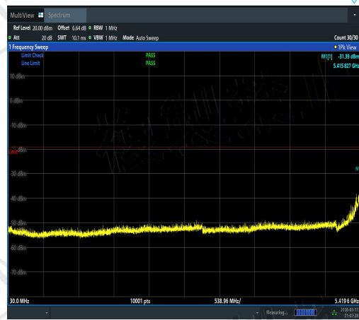
NTNV-11AC160MIMO-Ant3-5570-30~5419.6-PA SS
