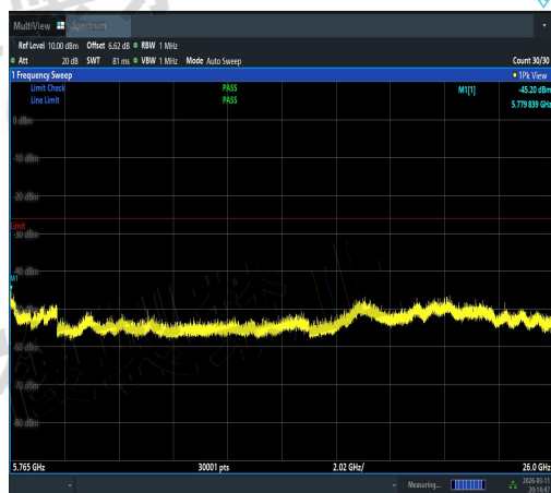
NTNV-11AC20MIMO-Ant2-5700-5765~26000-PA
