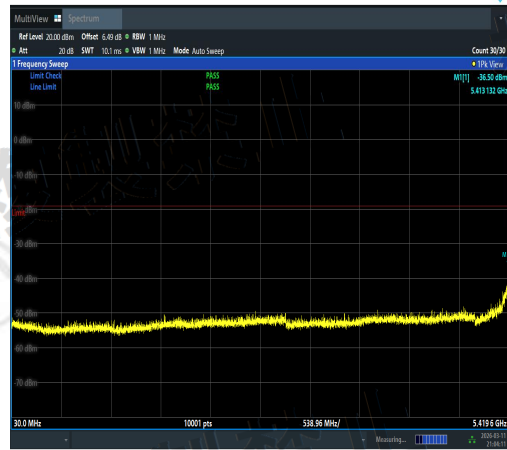
NTNV-11AC160MIMO-Ant1-5570-30~5419.6-PA SS
