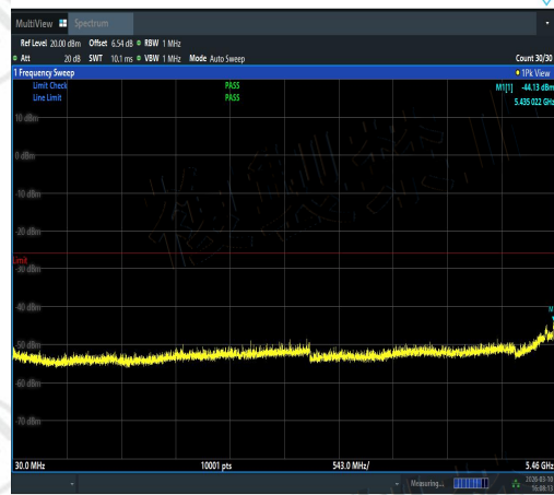
NTVN-11AX20SISO-Ant2-5600-30~5460-PASS
