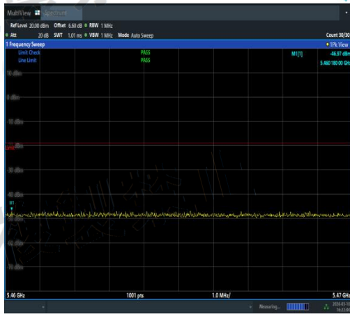
NTNV-11AX20SISO-Ant2-5720-5460~5470-PAS
