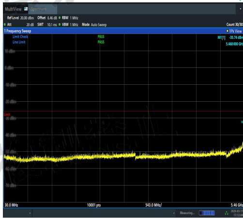
NTVN-11AX20SISO-Ant1-5500-30~5460-PASS
