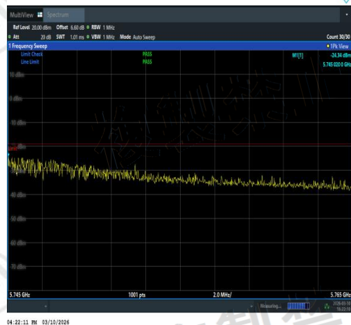
NTNV-11AX20SISO-Ant2-5720-5745~5765-See
