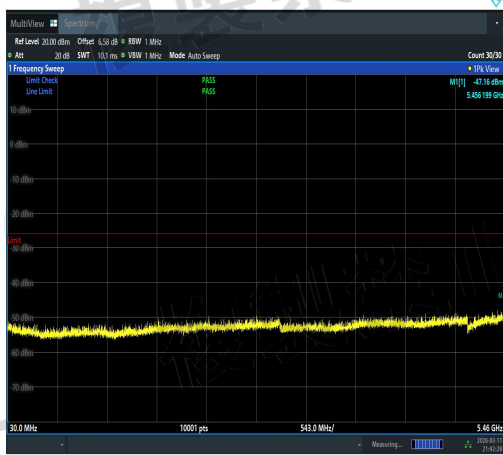
NTNV-11AX20MIMO-Ant1-5700-30~5460-PASS
