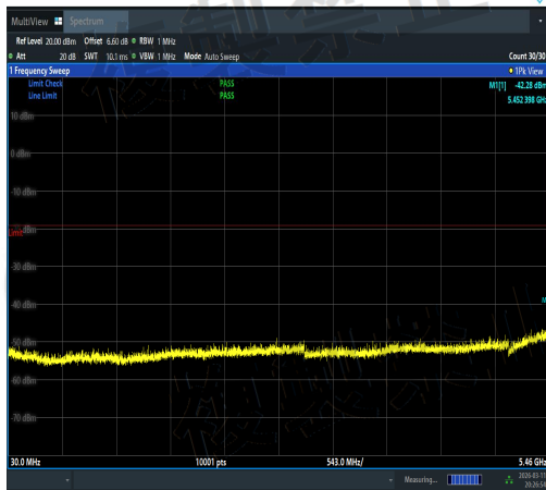
NTVN-11AC40MIMO-Ant3-5510-30~5460-PASS
