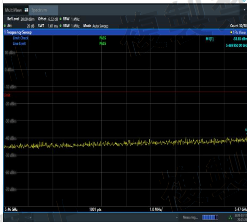
NTVN-11AC40MIMO-Ant2-5510-5460~5470-PASS
