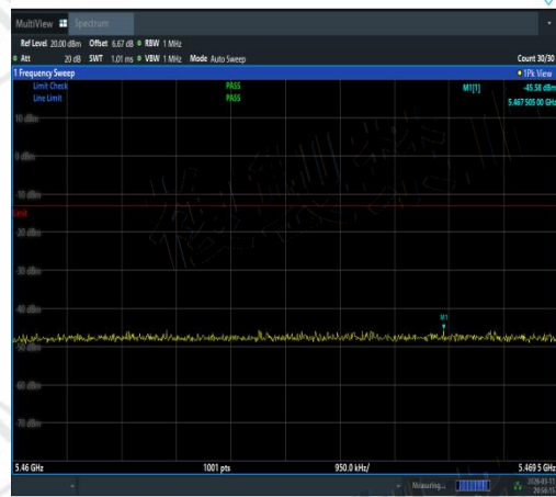
NTNV-11AC80MIMO-Ant3-5610-5460~5469.5-PASS
