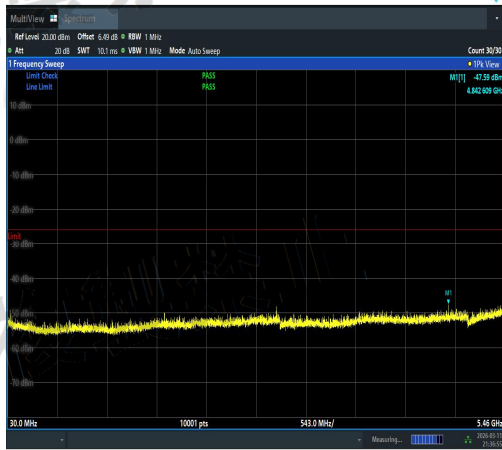
NTVN-11AX20MIMO-Ant1-5600-30~5460-PASS
