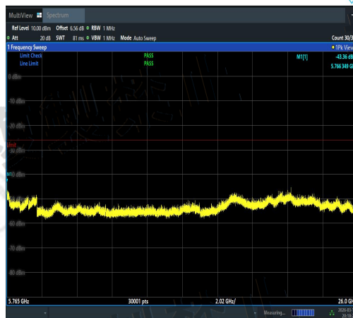
NTNV-11AC20MIMO-Ant1-5720-5765~26000-PA
