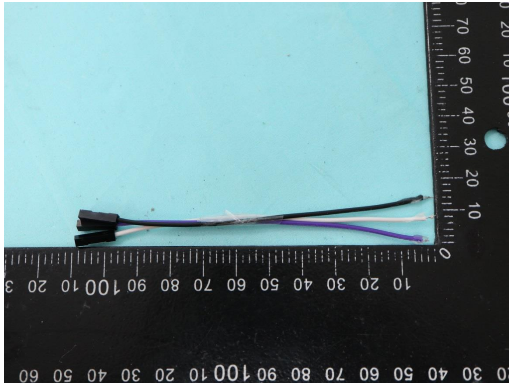
Fixture cable 杜邦線/ 彩色 cable 2.54mm female
