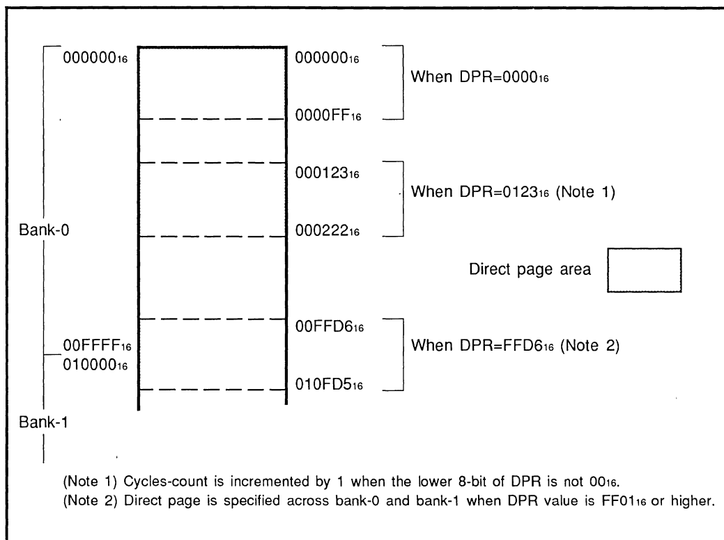
Fig. 2.2 Setting Direct Page by Direct Page Register
