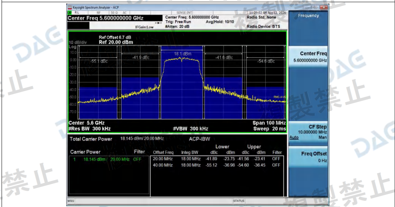
ACP_Measure_NVNT_ANT1_802_11a_5600_20M
