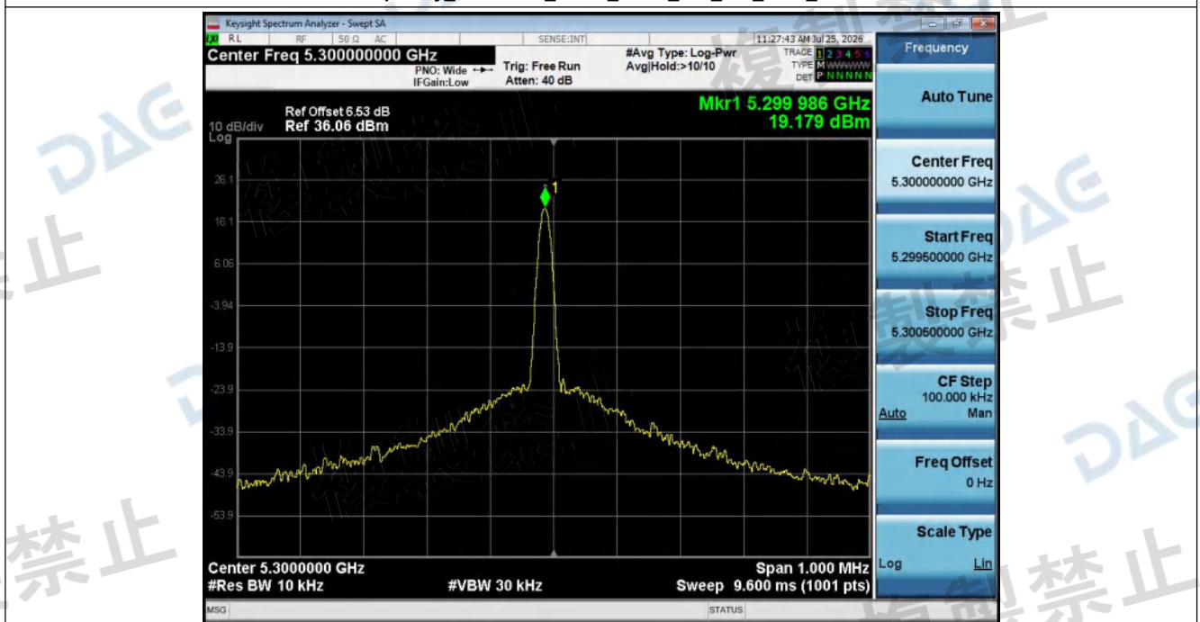
Frequency_Tolerance_NTLV_ANT1_802_11a_5300_20M
