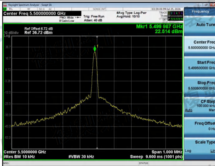
Frequency_Tolerance_NTLV_ANT1_802_11a_5500_20M
