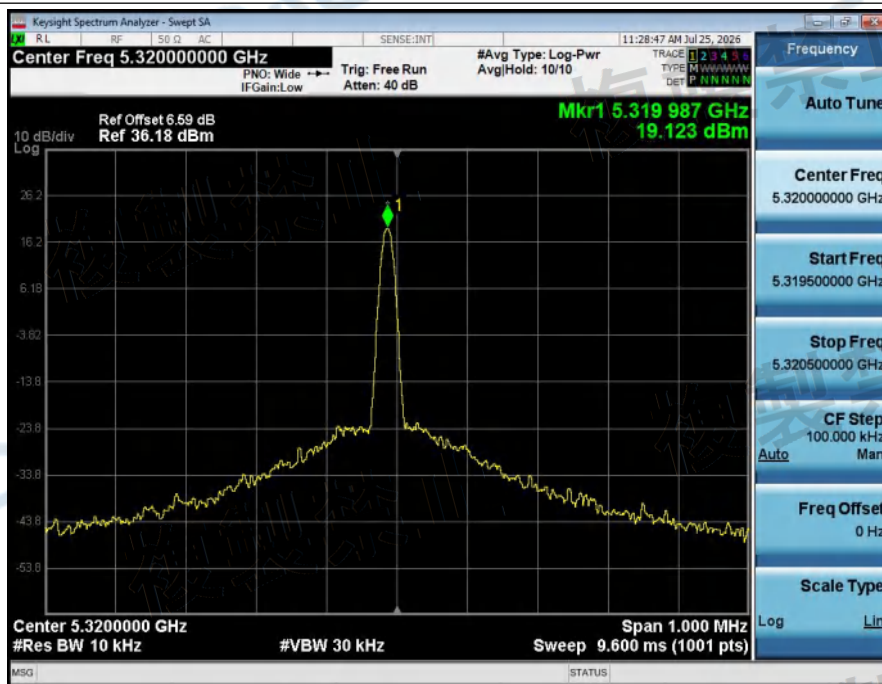
Frequency_Tolerance_NTHV_ANT1_802_11a_5320_20M
