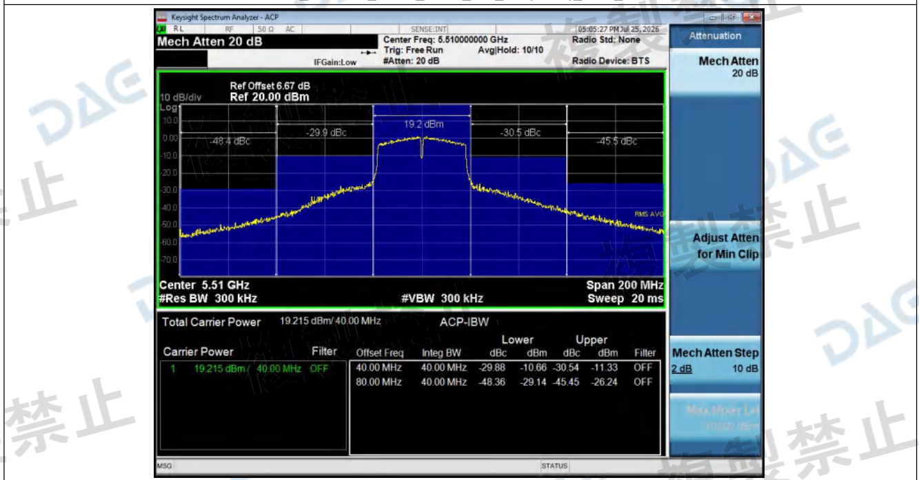
ACP_Measure_NVNT_ANT1_802_11n(HT40)_5510_40M
