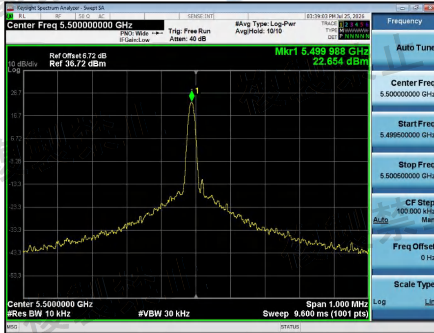
Frequency_Tolerance_NTLV_ANT1_802_11a_5500_20M
