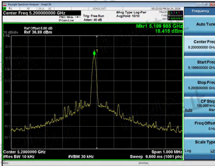
Frequency_Tolerance_NTHV_ANT1_802_11a_5200_20M
