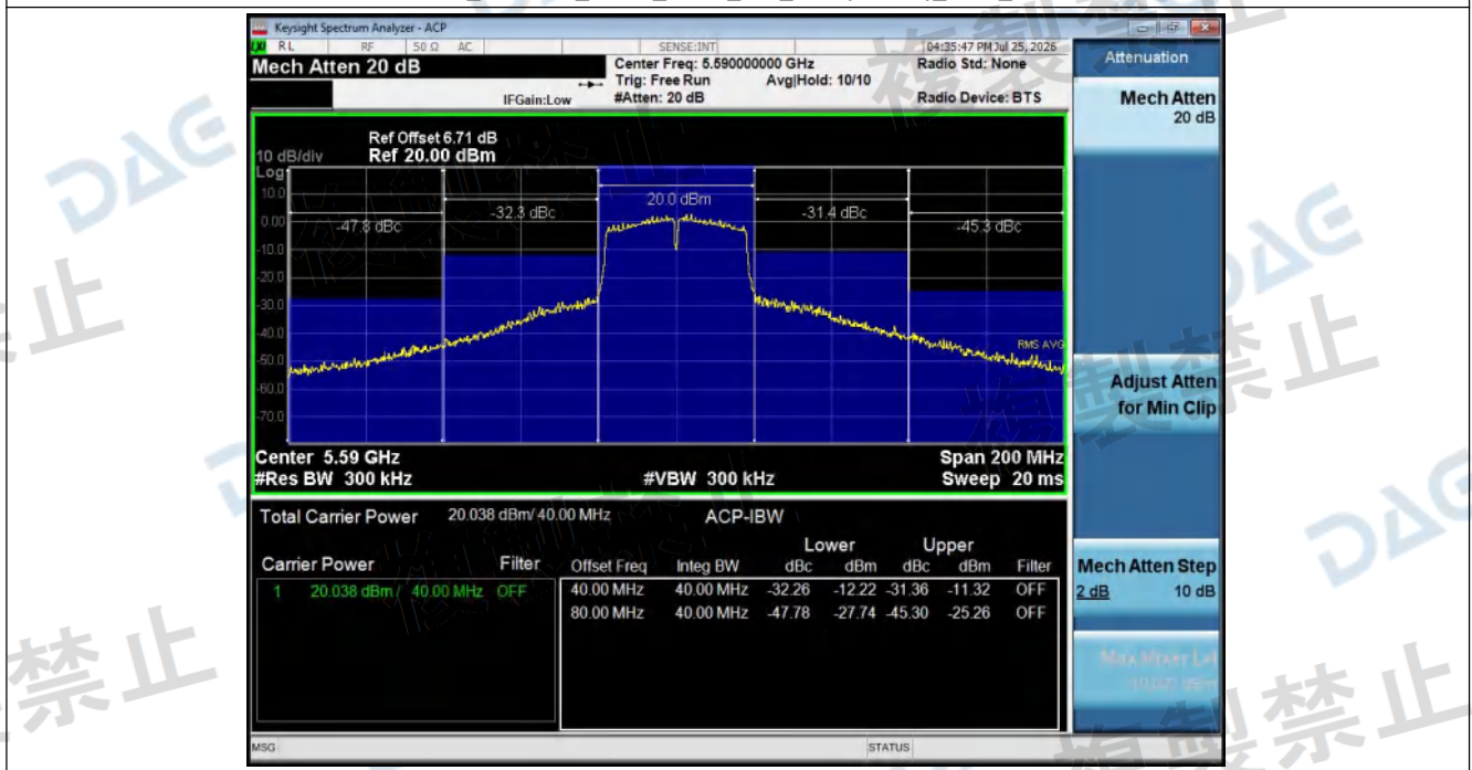
ACP_Measure_NVNT_ANT1_802_11ac(VHT40)_5590_40M
