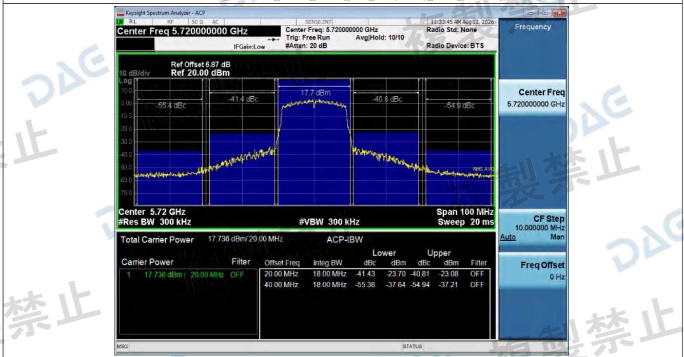
ACP_Measure_NVNT_ANT1_802_11n(HT20)_5720_20M
