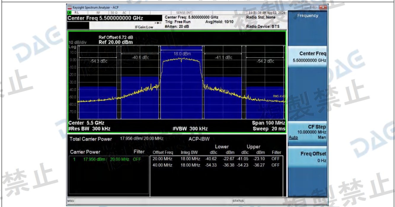
ACP_Measure_NVNT_ANT1_802_11n(HT20)_5500_20M
