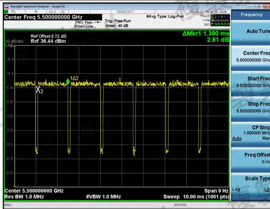
Burst_Length_NVNT_ANT1_802_11a_5500_20M
