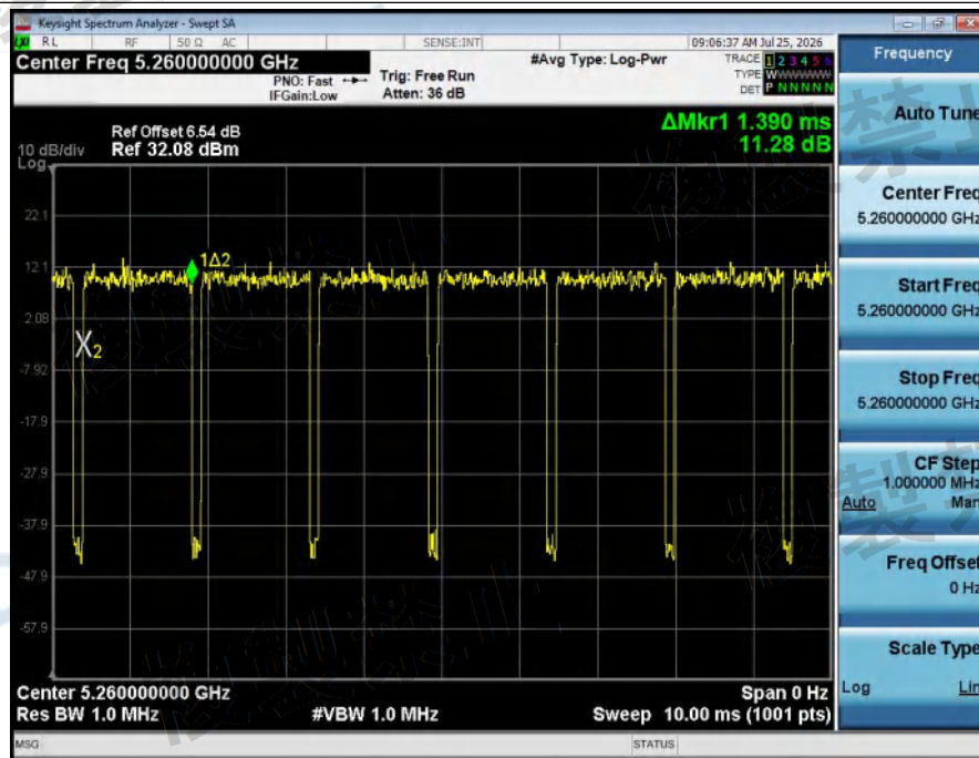
Burst_Length_NVNT_ANT1_802_11a_5260_20M
