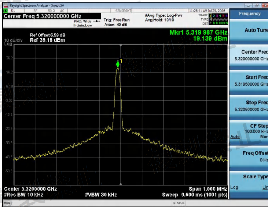
Frequency_Tolerance_NTLV_ANT1_802_11a_5320_20M
