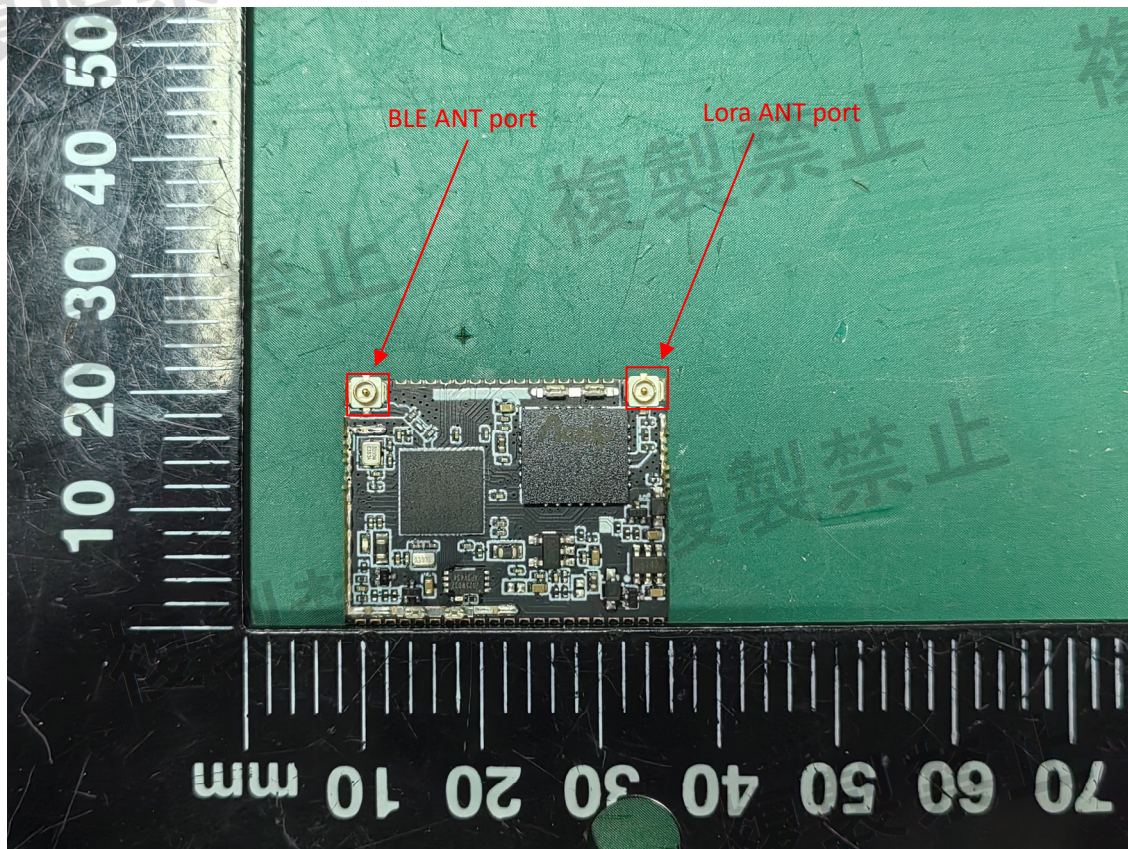
Antenna Port
