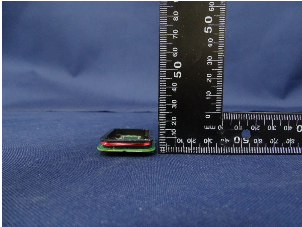
(5) EUT Photo - Trade Name: ELATEC, Model No.: TWN4 MultiTech 3 M
