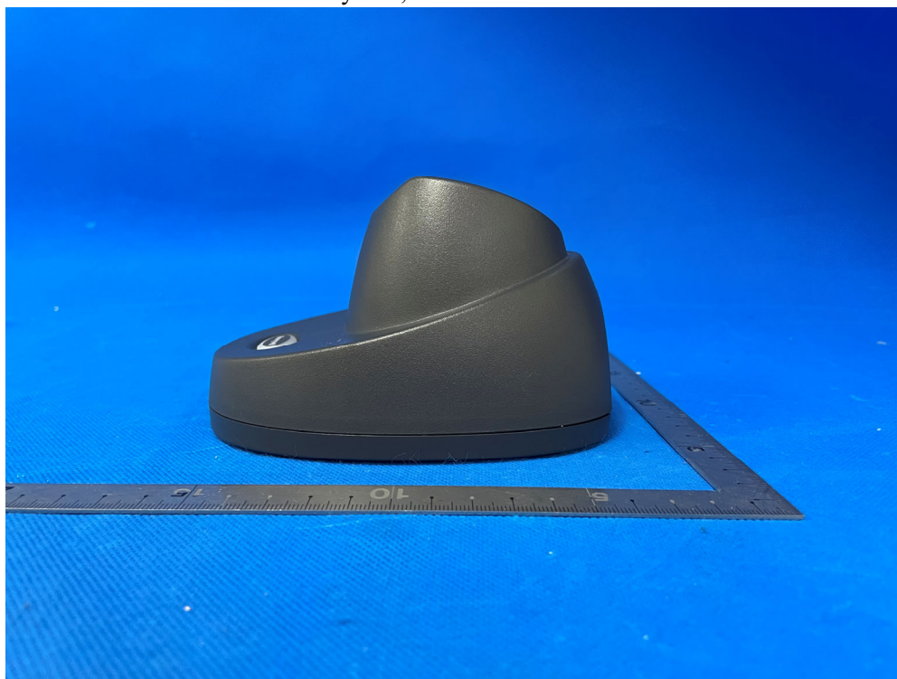
(5) EUT Photo - Trade Name: Honeywell, Model No.: CCB01-010BT
