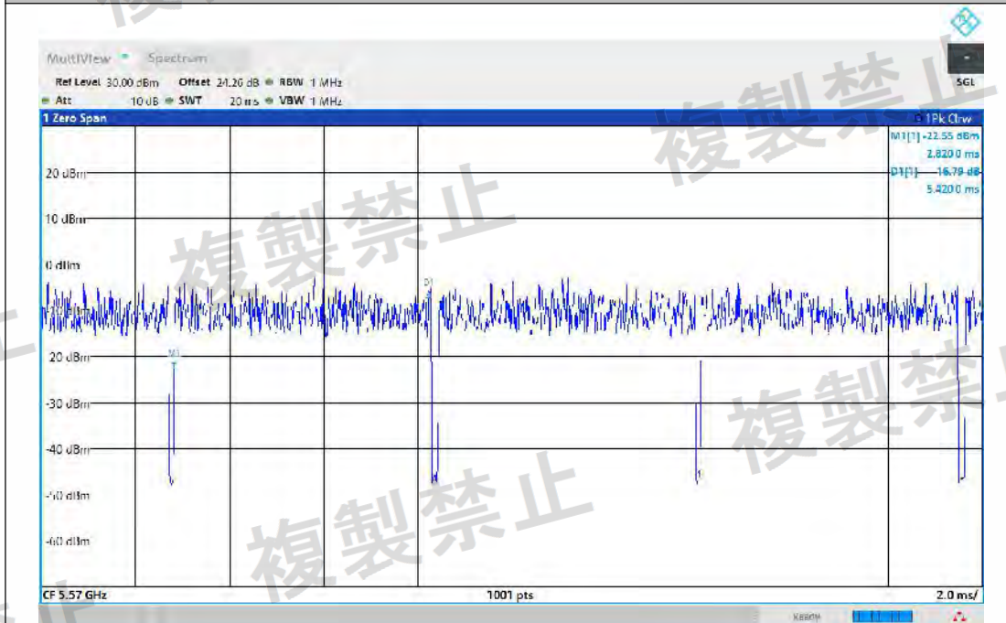
NTNV-11BE160MIMO-Ant2-5570-PASS
