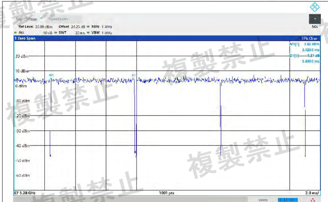
NTV-11BE20MIMO-Ant1-5280-PASS
