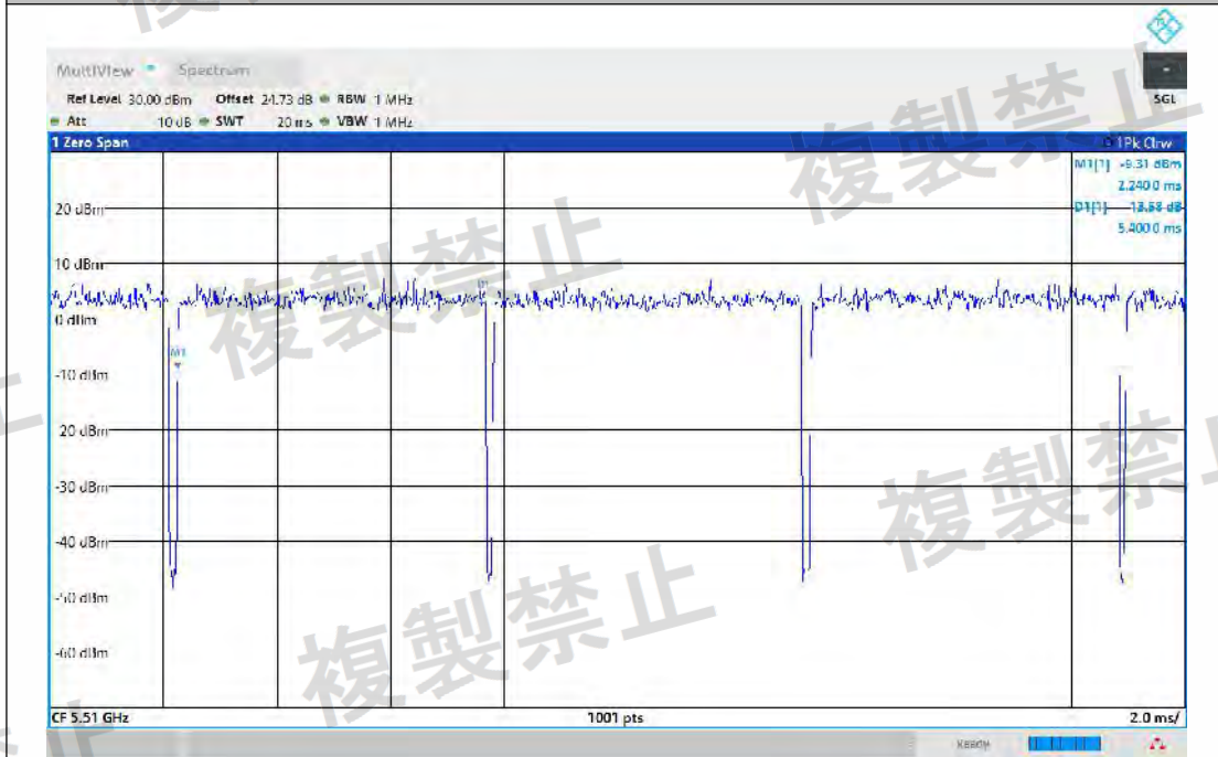
NTV-11AX40MIMO-Ant2-5510-PASS
