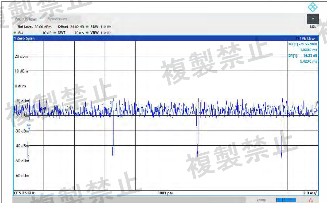
NTNV-11BE160MIMO-Ant1-5250-PASS
