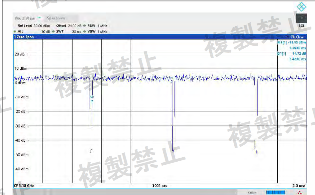
NTV-11AX20MIMO-Ant2-5180-PASS
