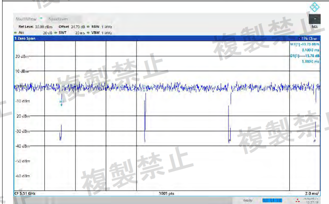
NTNV-11N40MIMO-Ant2-5510-PASS
