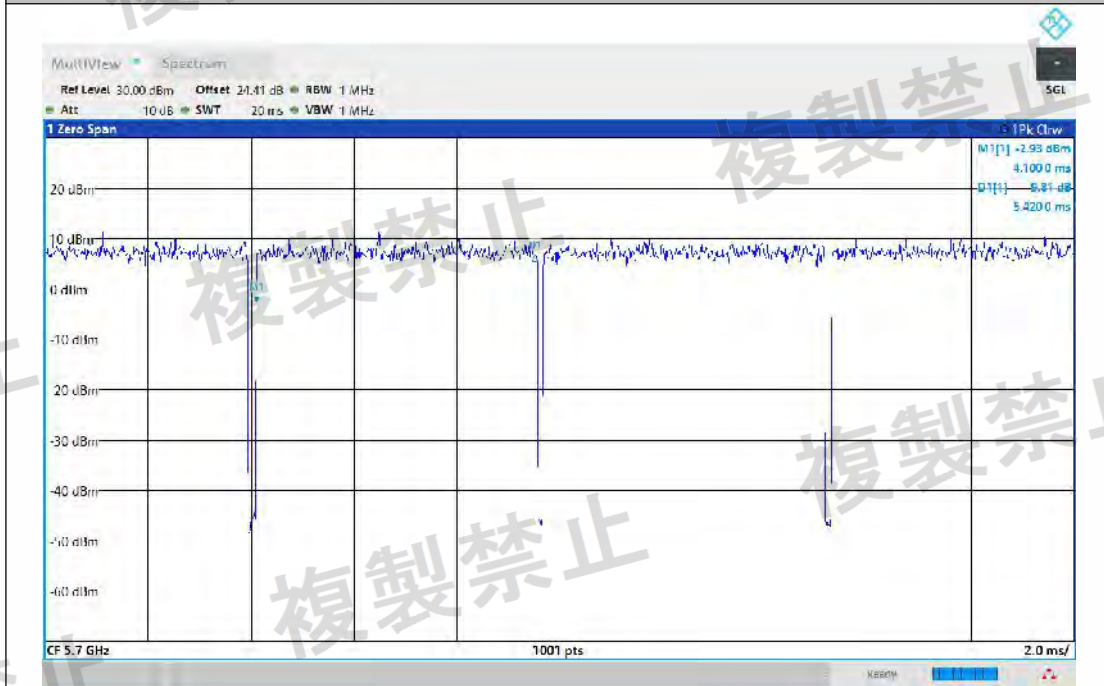
NTVN-11BE20MIMO-Ant2-5700-PASS
