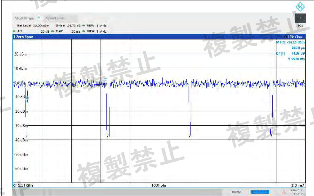
NTNV-11AC40MIMO-Ant2-5510-PASS
