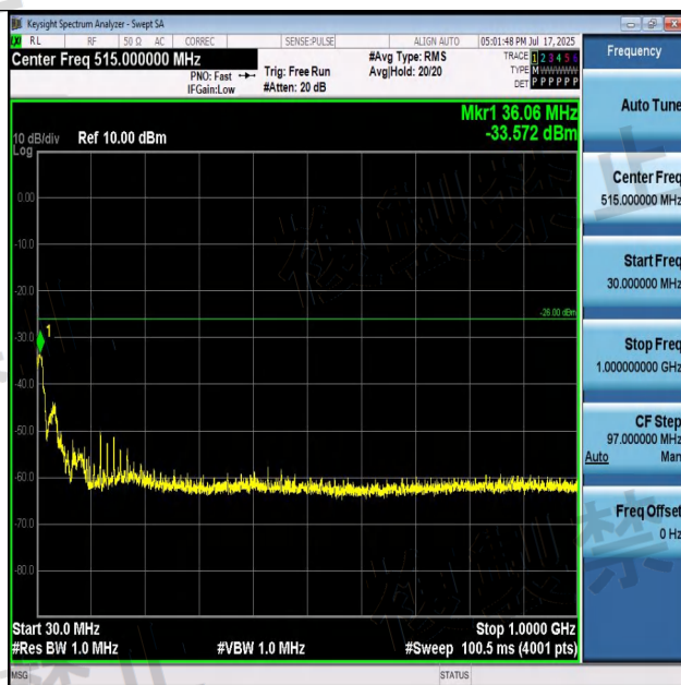
NTNV-BLE_1M-Ant1-2440-30~1000-PASS
