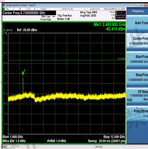
NTNV-BLE_1M-Ant1-2402-1000~12500-PASS
