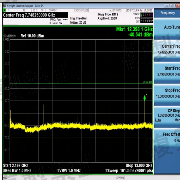
NTNV-BLE_1M-Ant1-2480-2496.5~13000-PASS
