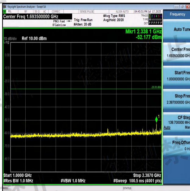
NTNV-BLE_1M-Ant1-2402-1000~2387-PASS
