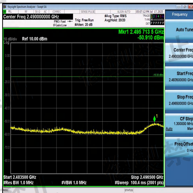
NTNV-BLE_1M-Ant1-2480-2483.5~2496.5-PASS
