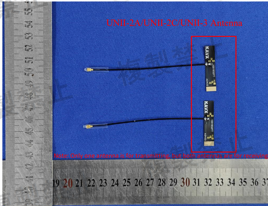
View of Product-9 (Antenna: 1001932FT)
