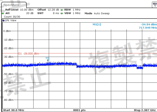
NTNV-BLE_125K-Ant1-2440-30~2387-PASS
