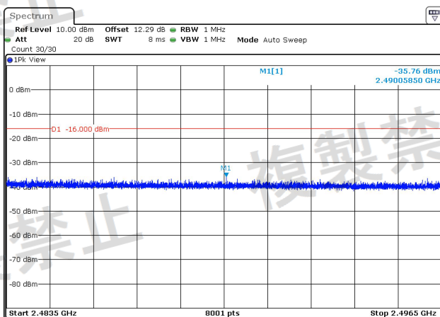
NTNV-BLE_125K-Ant1-2480-2483.5~2496.5-PASS
