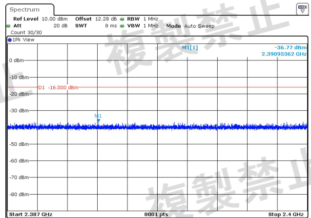
NTNV-BLE_125K-Ant1-2440-2387~2400-PASS
