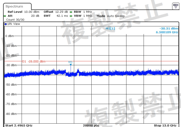
NTNV-BLE_125K-Ant1-2480-2496.5~13000-PASS
