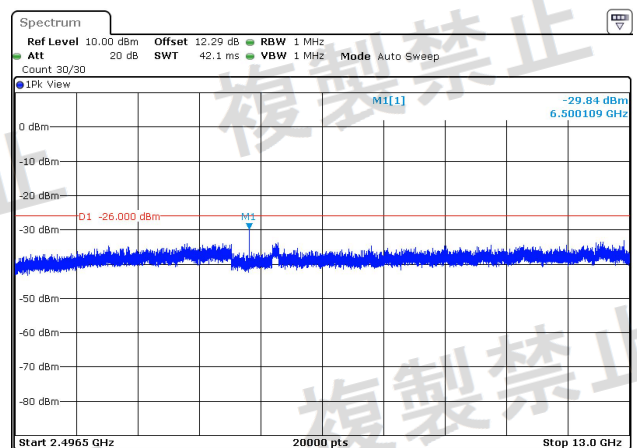
NTNV-BLE_500K-Ant1-2480-2496.5~13000-PASS
