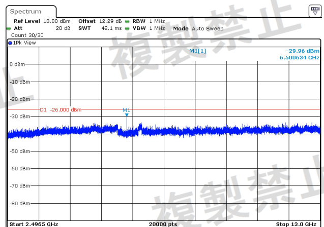
NTNV-BLE_1M-Ant1-2480-2496.5~13000-PASS
