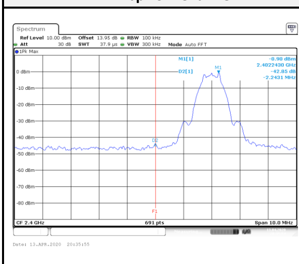
BLE-1Mbps Low Channel
