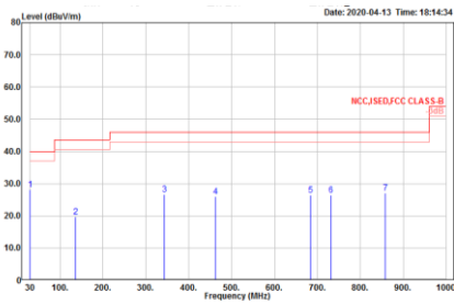
BLE Receiver Mode Horizontal (30 MHz – 1GHz)
