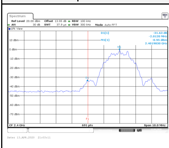
BLE-2Mbps Low Channel
