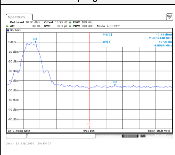
BLE-1Mbps High Channel
