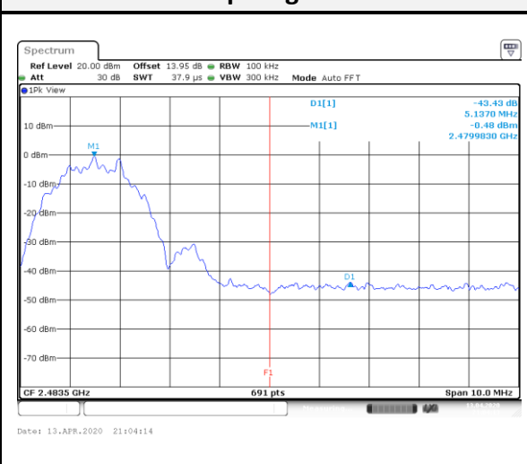
BLE-2Mbps High Channel
