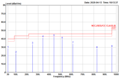
BLE Receiver Mode Vertical (30 MHz – 1GHz)
