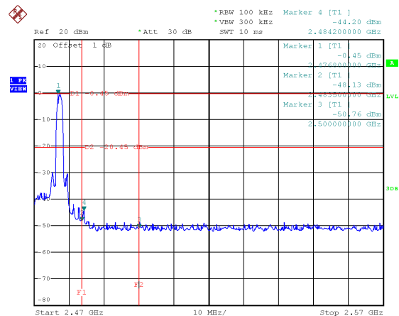
Bandedge- CH38 (Upper)
