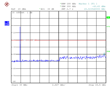
CH38 – 10th Harmonic of the fundamental frequency
