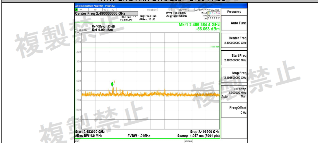
NTNV-2.4G-Ant1-2475-2483.5~2496.5-PASS
