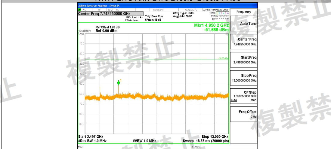
NTNV-2.4G-Ant1-2475-2496.5~13000-PASS
