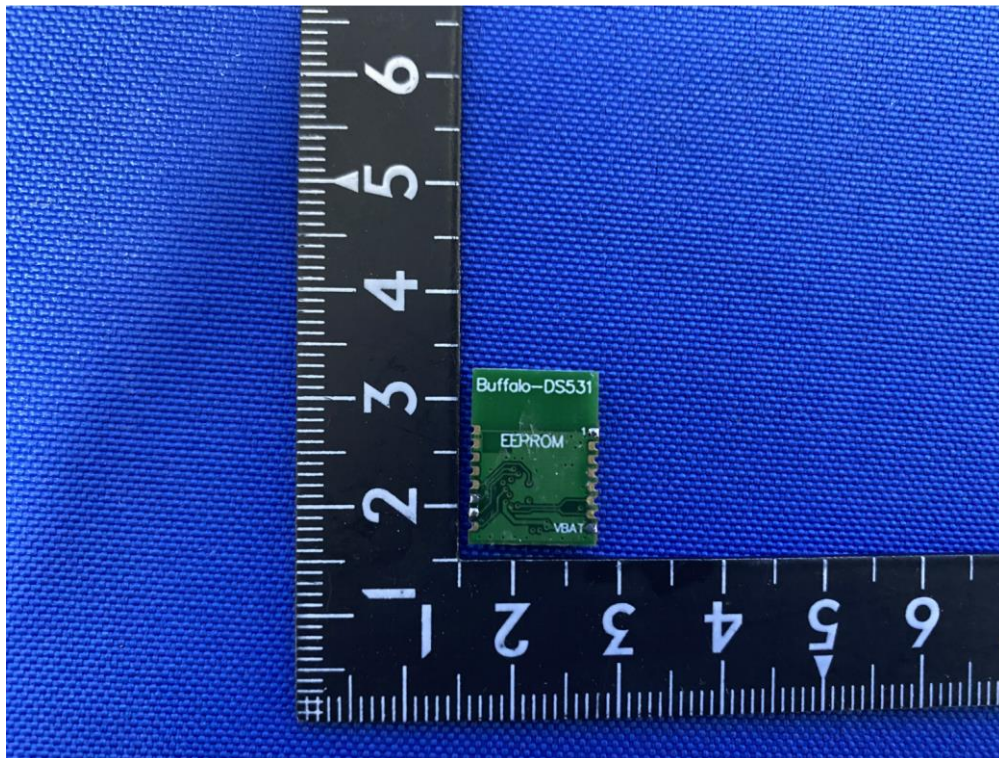
(2) EUT Photo (Buffalo-DS531-C)
