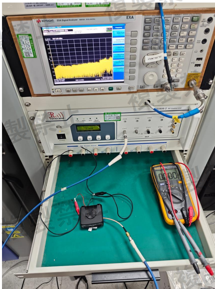
Antenna Terminal Test View
