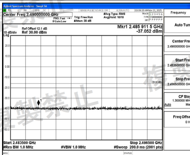
NTNV_2DH5_Ant1_2480_2496.5~13000
