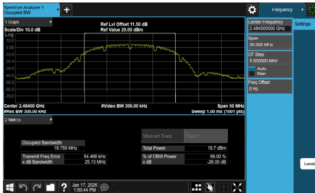
99% OBW
