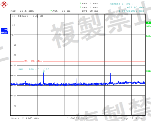
8DPSK_High_3DH1(2.4965GHz~12.5GHz)
