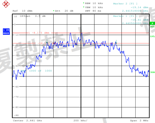
8DPSK_Middle Channel
