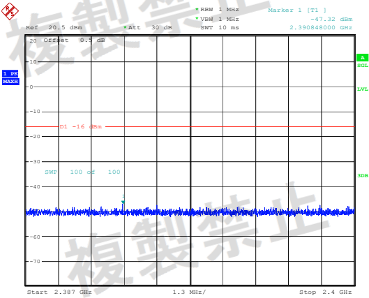
8DPSK_High_3DH1(2.387GHz~2.4GHz)
