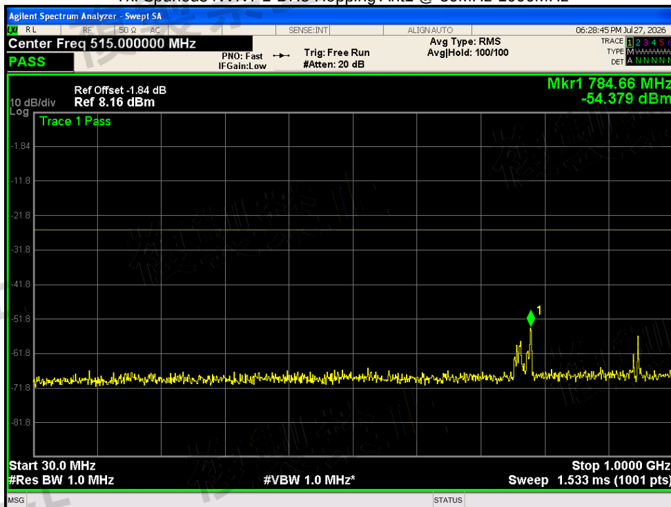
Tx. Spurious NVNT 1-DH5 Hopping Ant1 @ 30MHz-1000MHz
