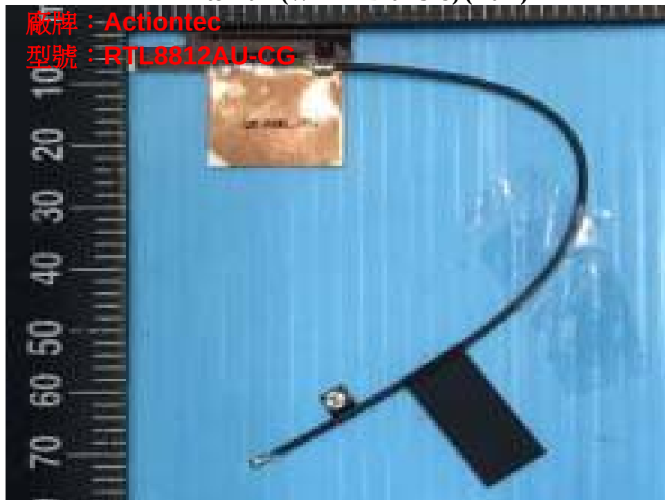
Tx Antenna 2 (WA-P-LB-02-379) (main)
