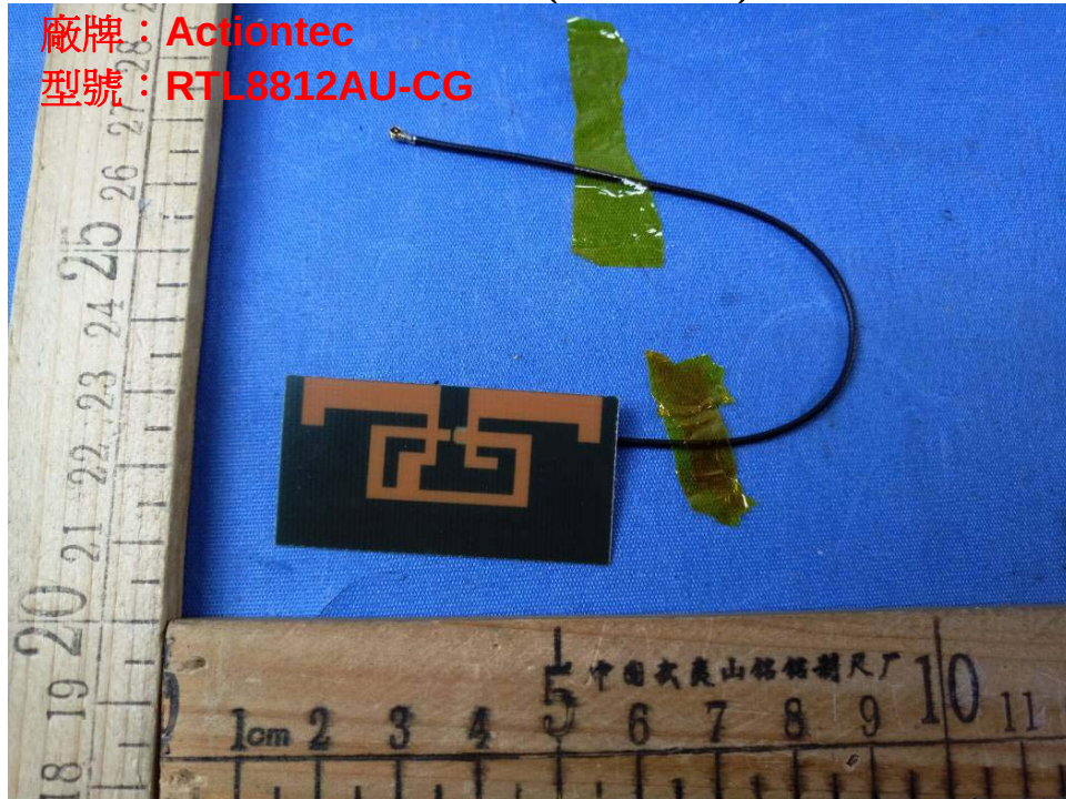
Tx Antenna 1 (main & aux)
