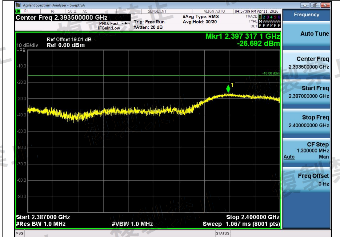
NTNV-11B-Ant1-2412-2387~2400-PASS
