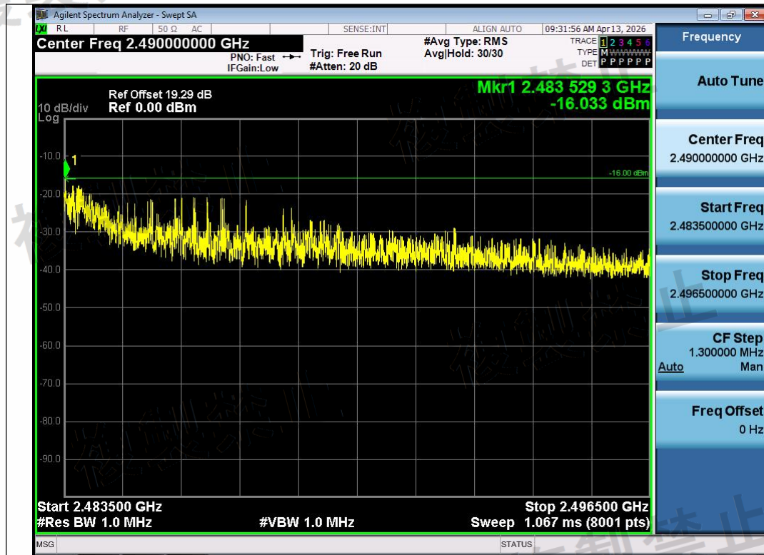
NTNV-11N20SISO-Ant1-2472-2483.5~2496.5-See table below
