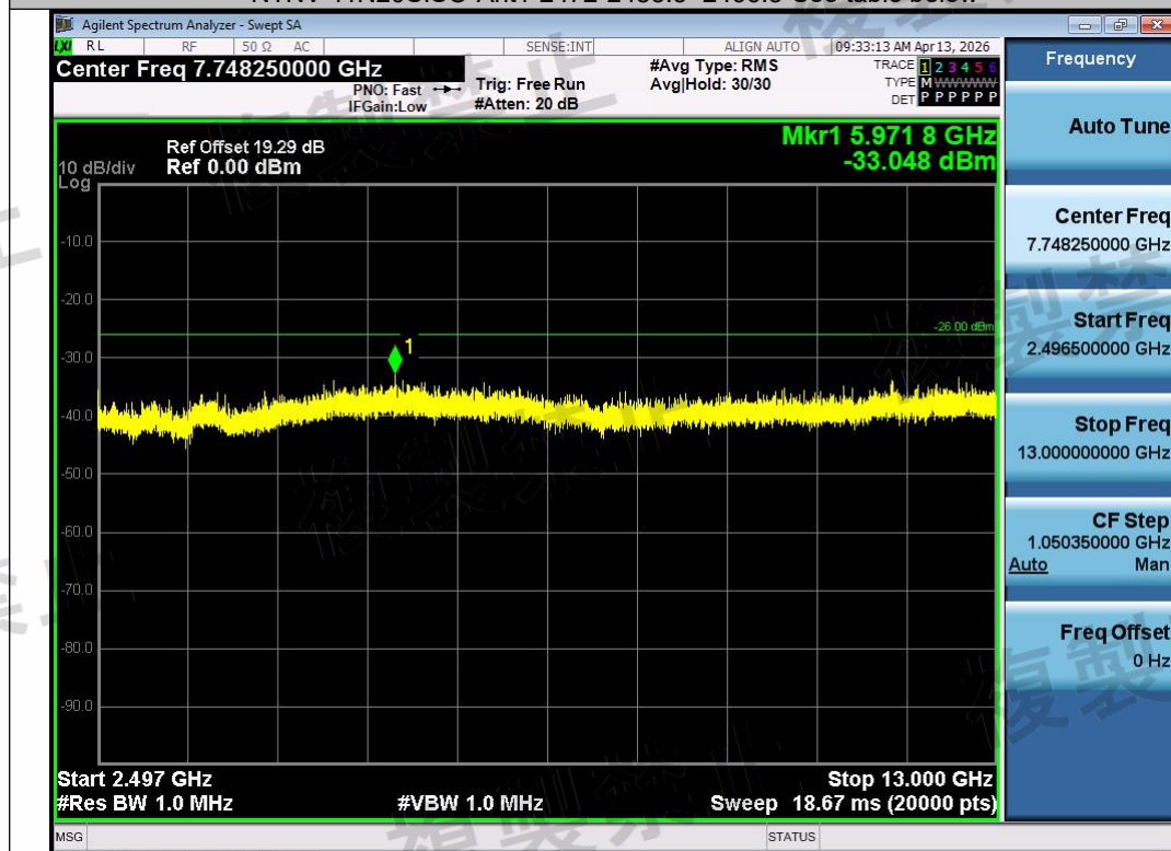
NTNV-11N20SISO-Ant1-2472-2496.5~13000-PASS
