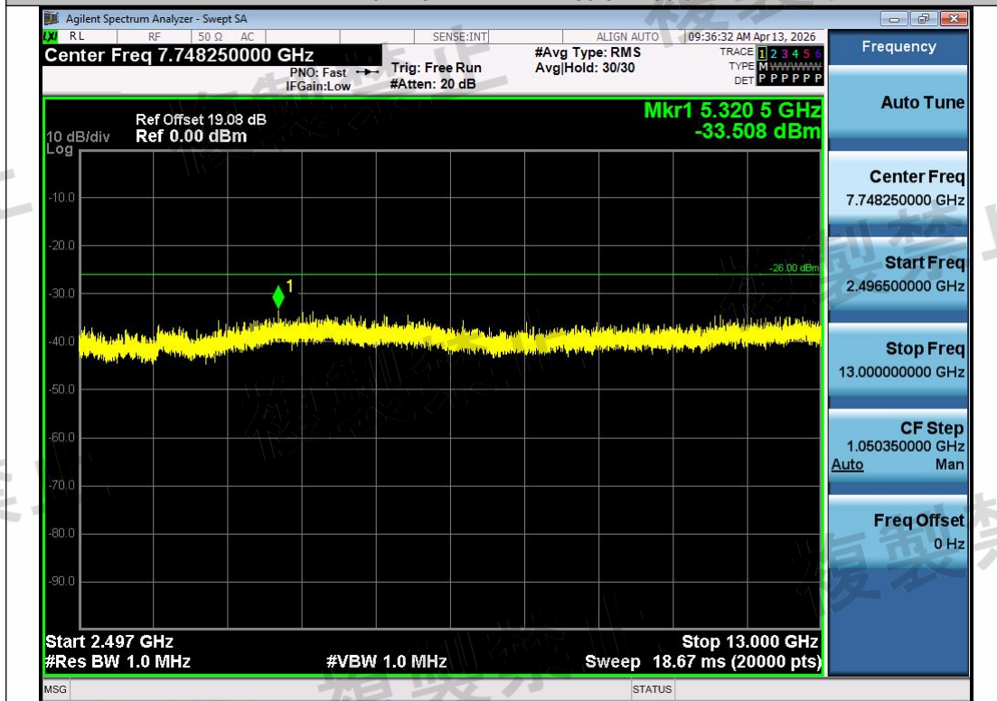
NTNV-11N40SISO-Ant1-2422-2496.5~13000-PASS
