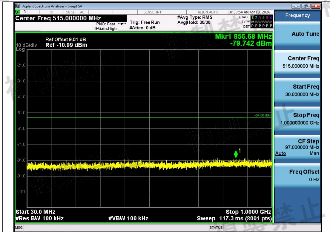
NTNV-11B-Ant1-2412-30~1000-PASS
