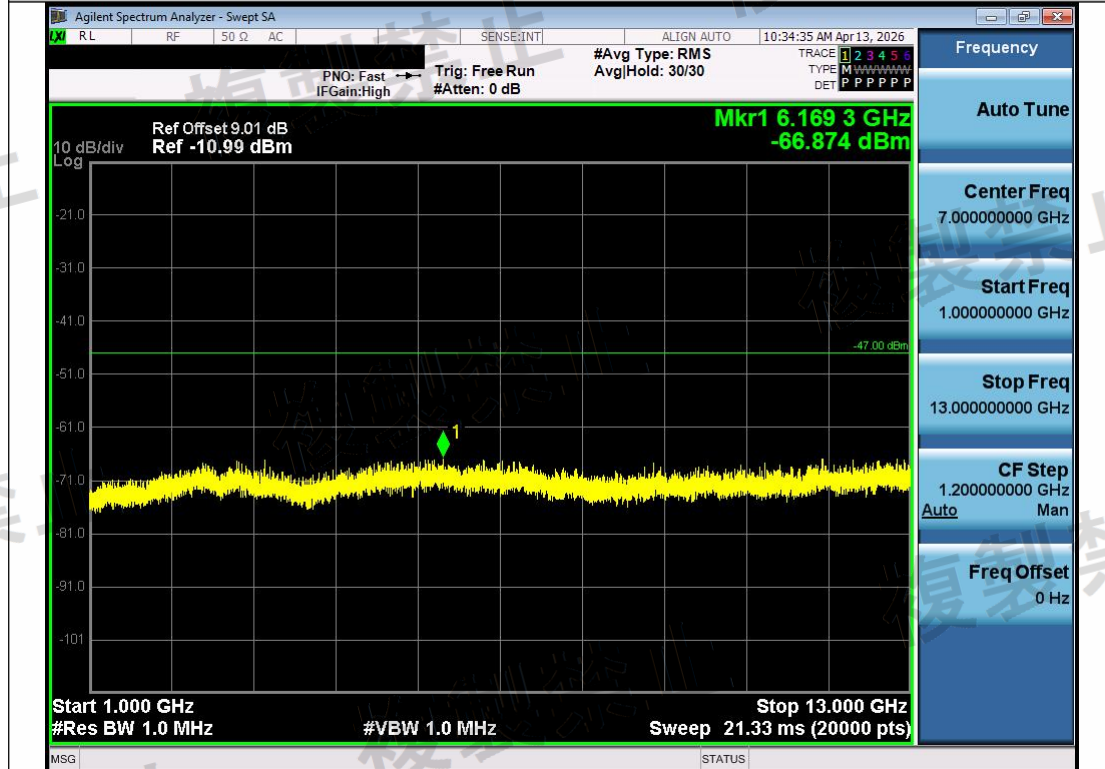
NTNV-11B-Ant1-2412-1000~13000-PASS
