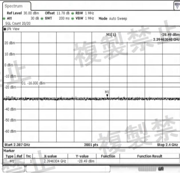
NTNV-11B-Ant1-2442-2387~2400-PASS
