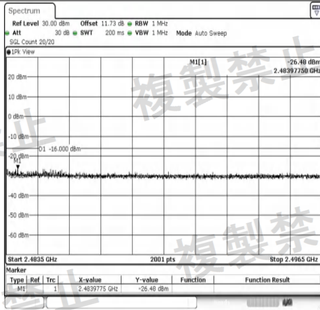
NTNV-11N20SISO-Ant1-2472-2483.5~2496.5-PASS
