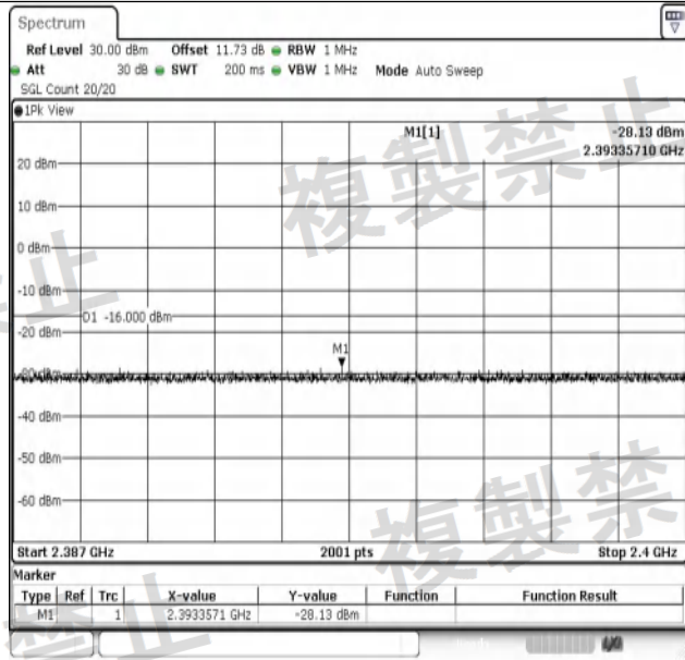
NTNV-11G-Ant1-2472-2387~2400-PASS
