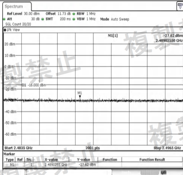
NTNV-11G-Ant1-2472-2483.5~2496.5-PASS
