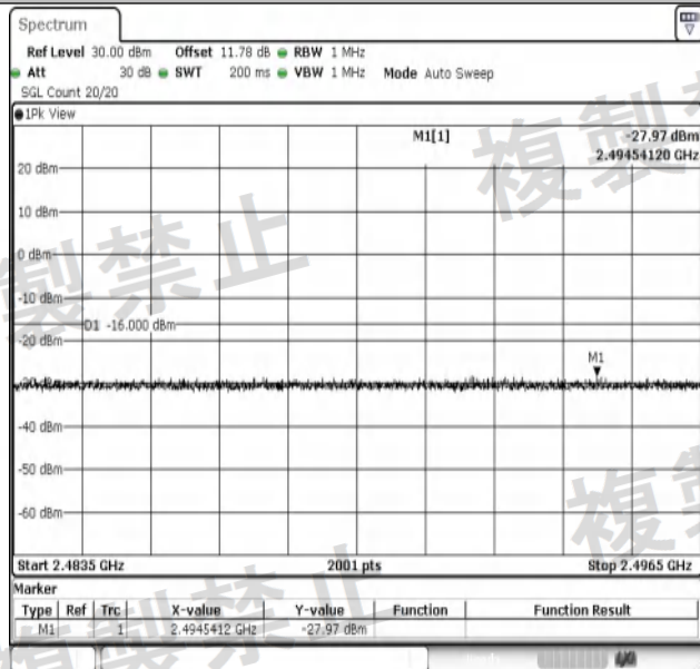
NTNV-11B-Ant1-2442-2483.5~2496.5-PASS
