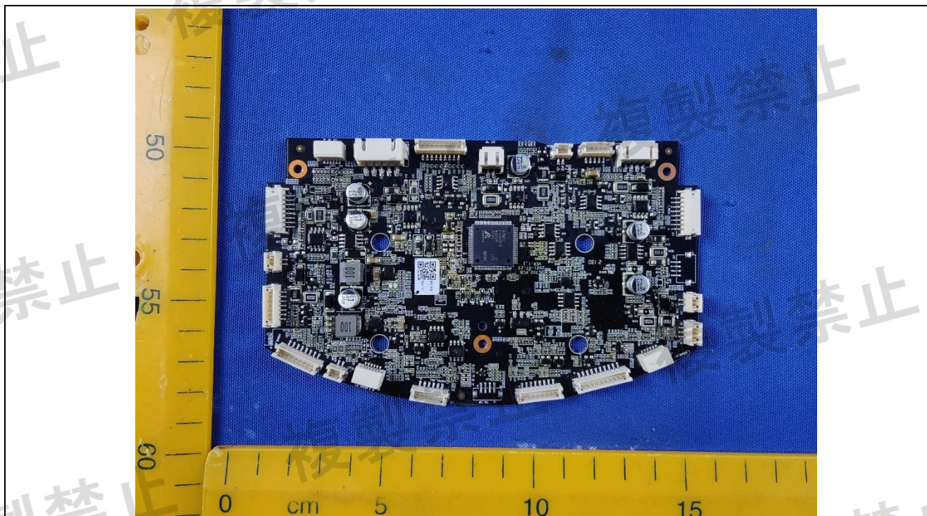
Details of: Main board
