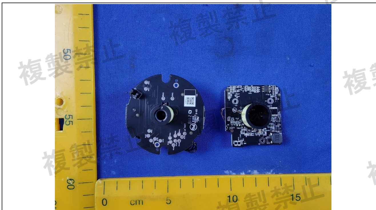
Details of: PCB view for Lidar module
