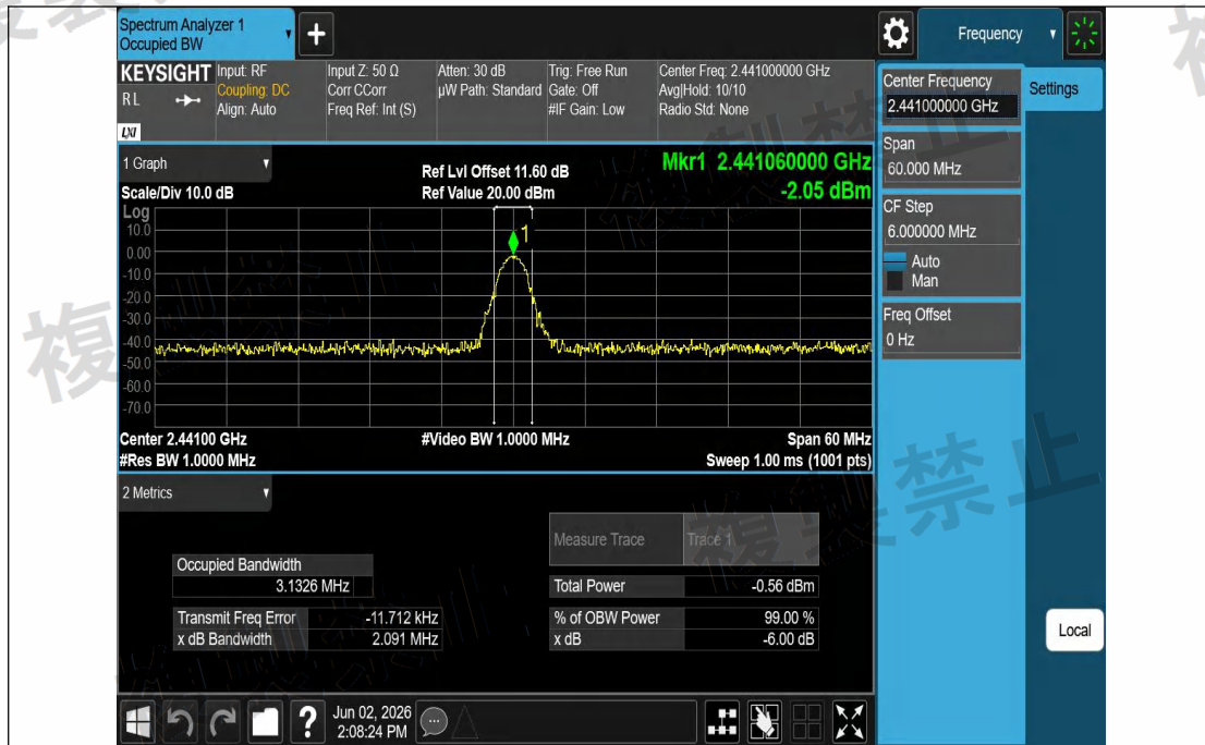
NTNV-2DH5-Ant1-2441-PASS
