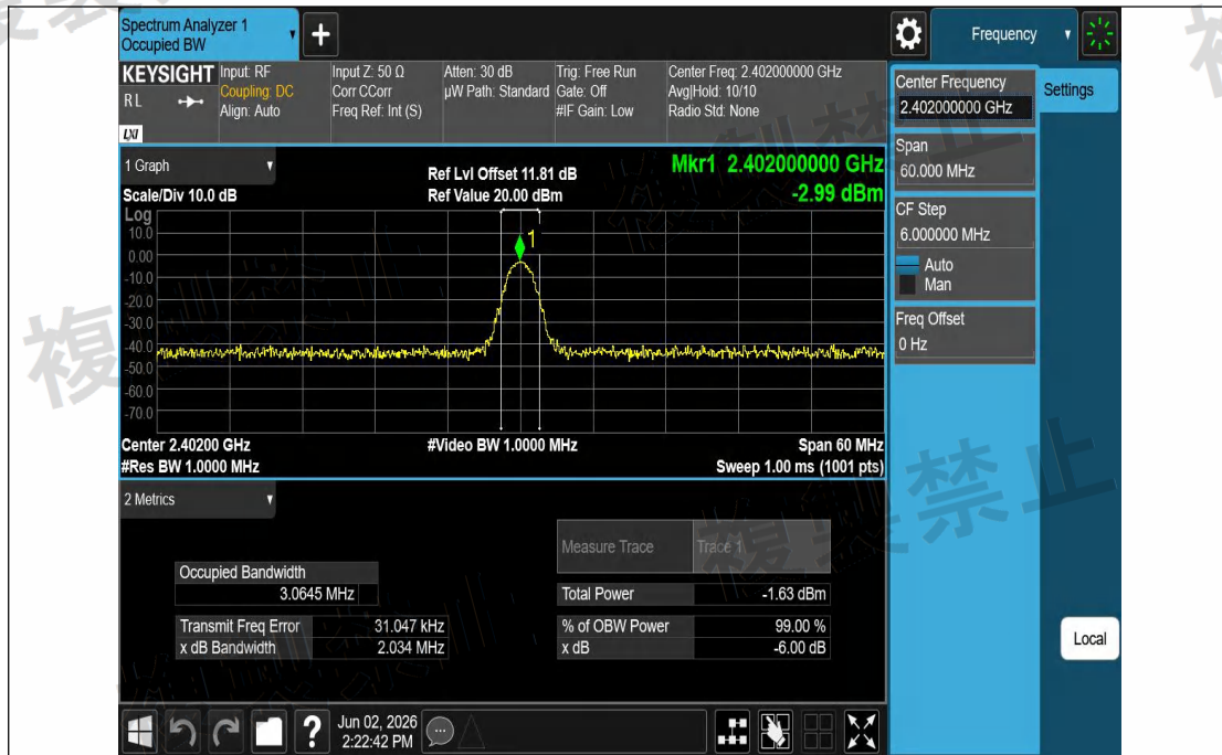
NTNV-3DH5-Ant1-2402-PASS
