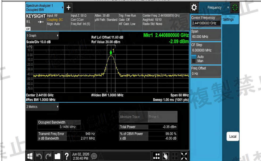
NTNV-3DH5-Ant1-2441-PASS
