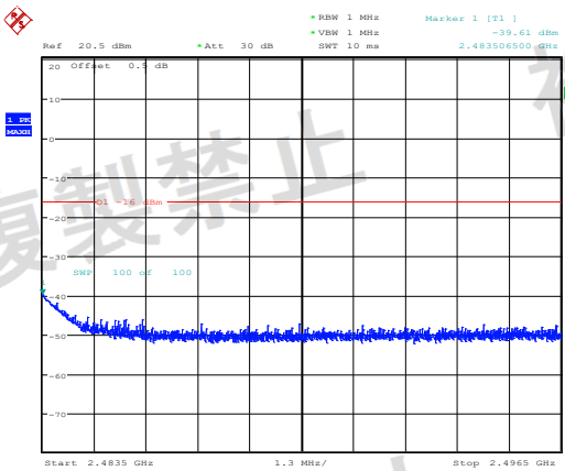
GFSK_High_DH1(2.4835GHz~2.4965GHz)
