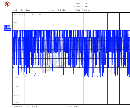
GFSK_Hopping_AFH_DH1
