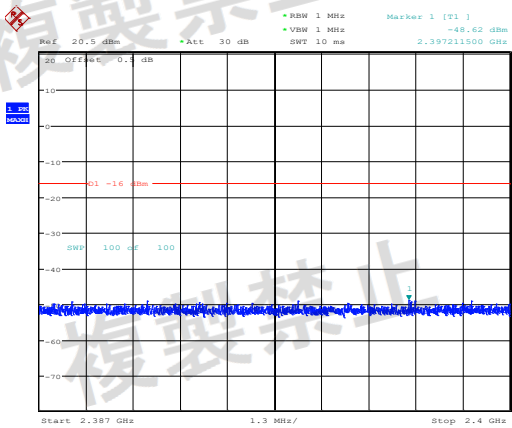
GFSK_High_DH1(2.387GHz~2.4GHz)
