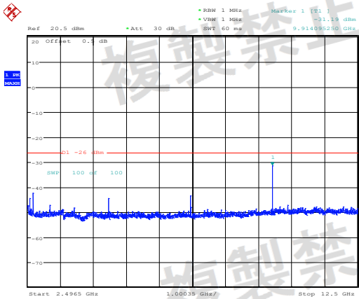
GFSK_High_DH1(2.4965GHz~12.5GHz)
