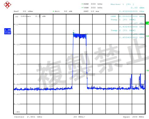
Spreading Bandwidth
