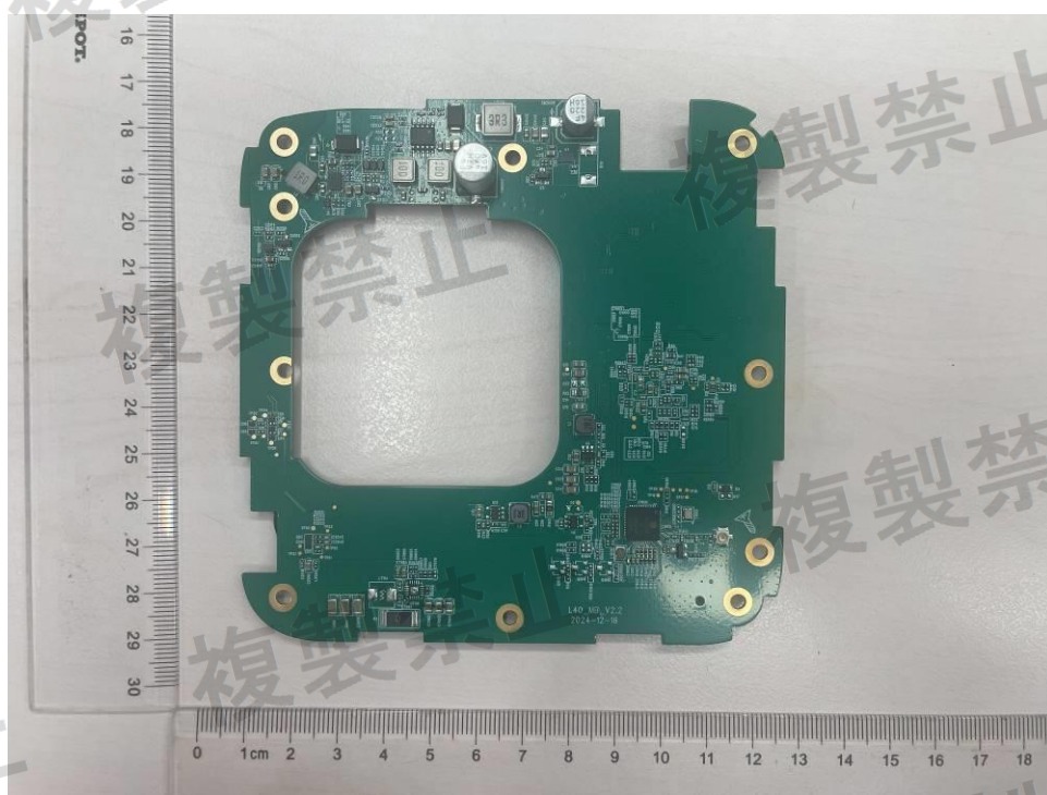
Figure 8: Bottom view of main board
