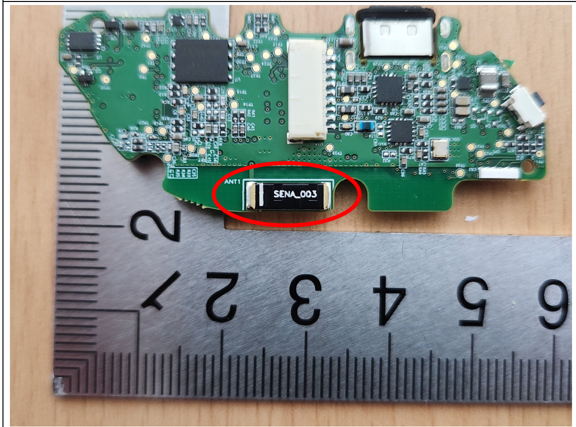
BT Antenna
