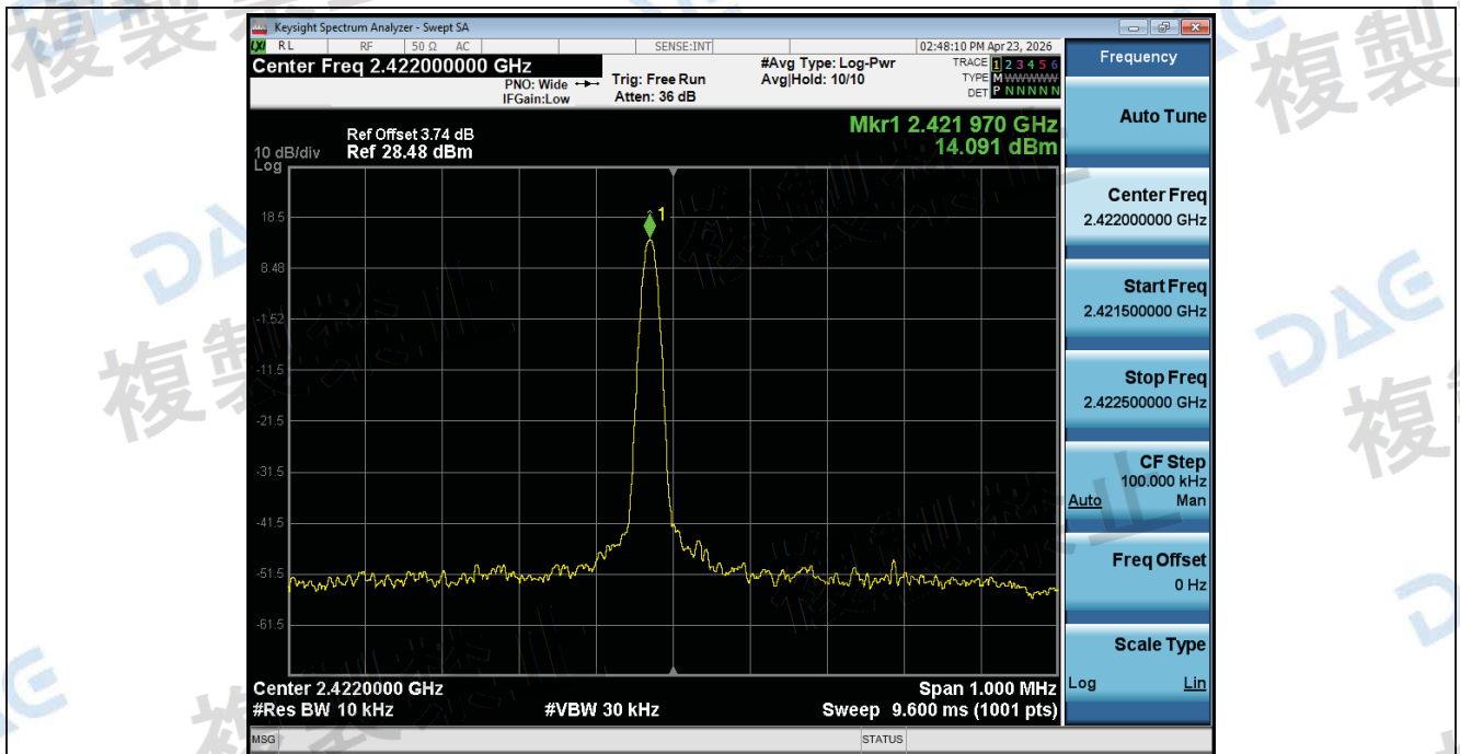
Frequency_Tolerance_NTLV_ANT1_802_11n(HT40)_2422
