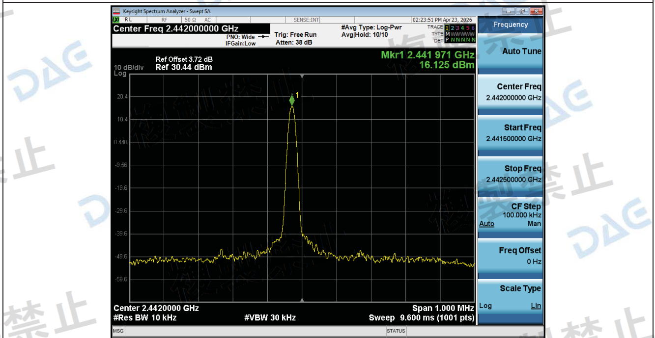
Frequency_Tolerance_NTHV_ANT1_802_11ax(HE20)_2442
