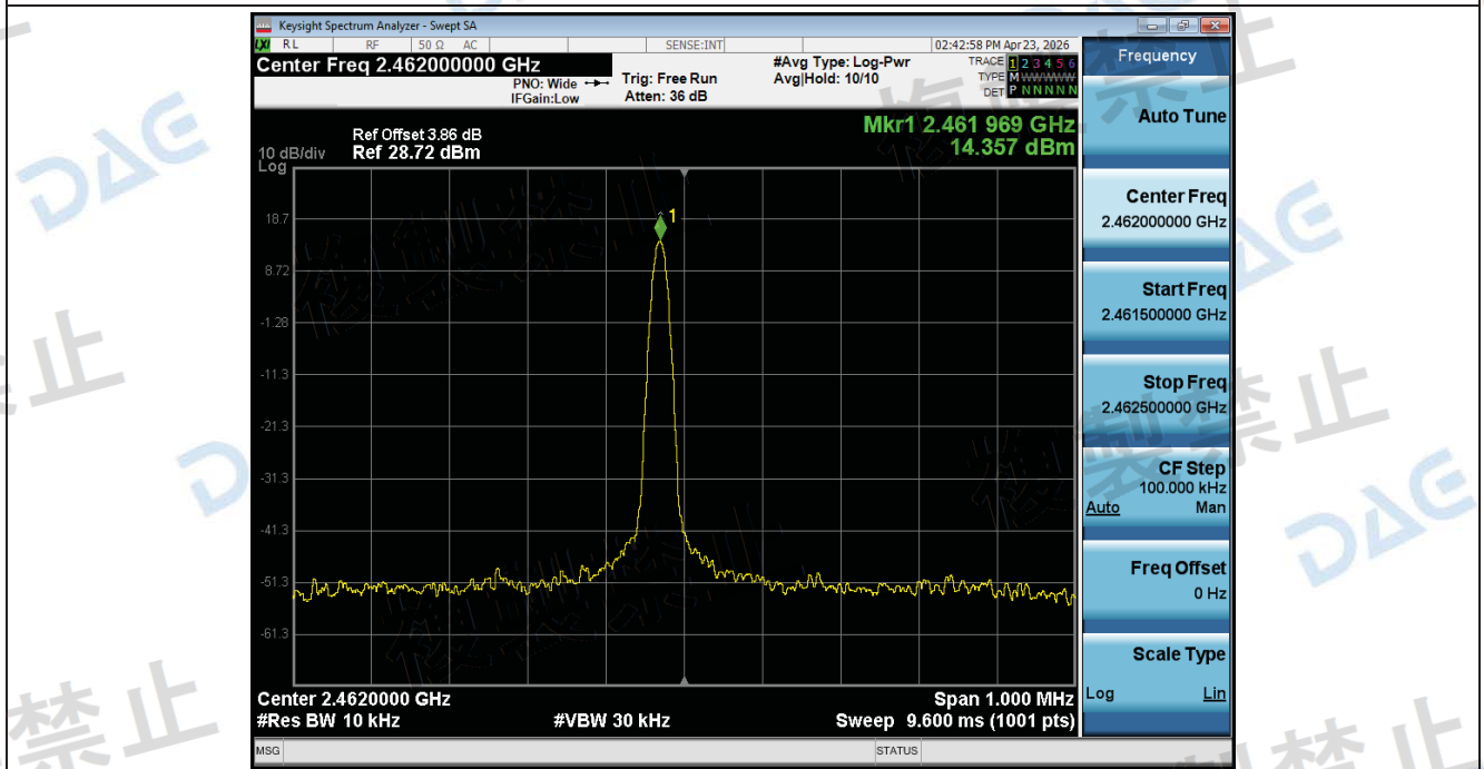
Frequency_Tolerance_NTHV_ANT1_802_11ax(HE40)_2462
