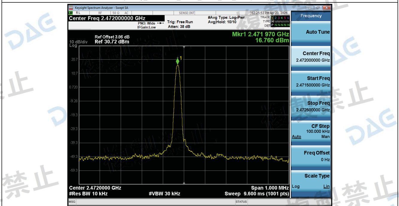
Frequency_Tolerance_NTLV_ANT1_802_11ax(HE20)_2472
