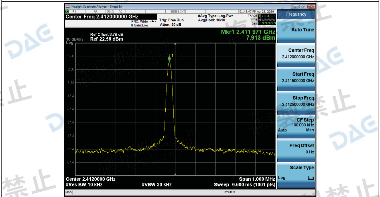
Frequency_Tolerance_NTHV_ANT1_802_11g_2412
