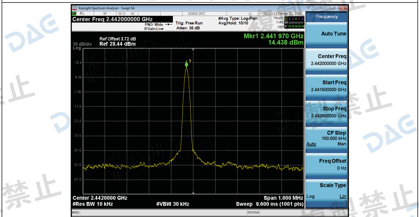
Frequency_Tolerance_NTLV_ANT1_802_11n(HT40)_2442
