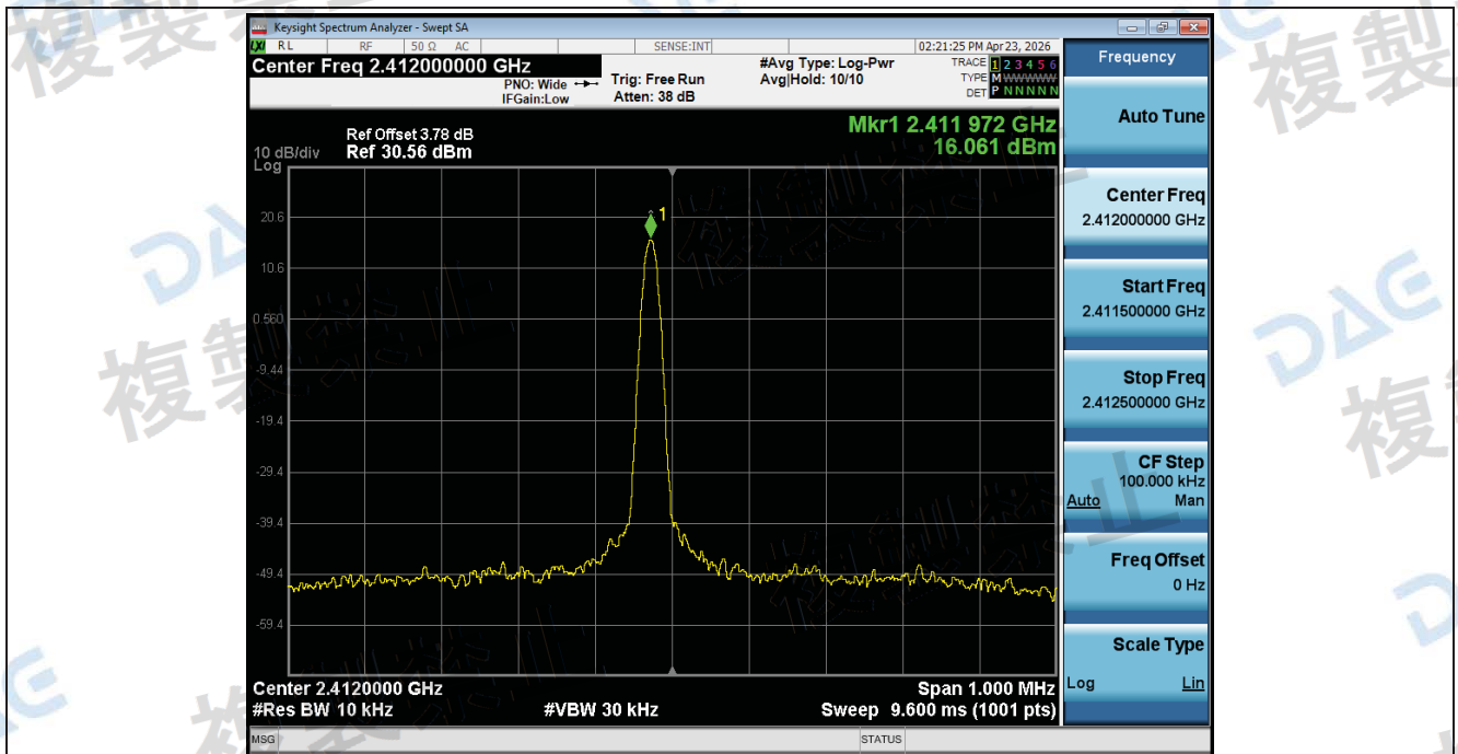
Frequency_Tolerance_NTHV_ANT1_802_11ax(HE20)_2412
