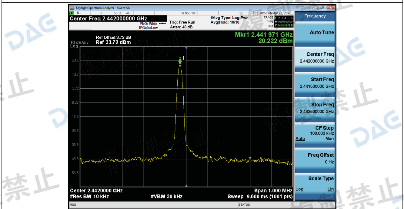
Frequency_Tolerance_NTLV_ANT1_802_11b_2442
