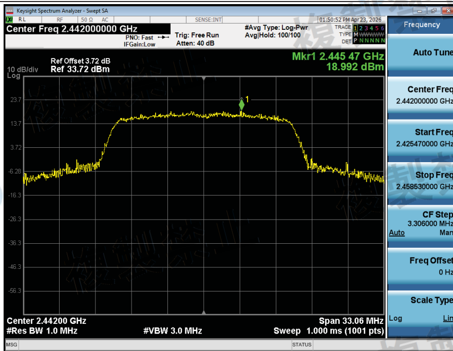
2_Antena_Power_NVNT_ANT1_802_11g_2442
