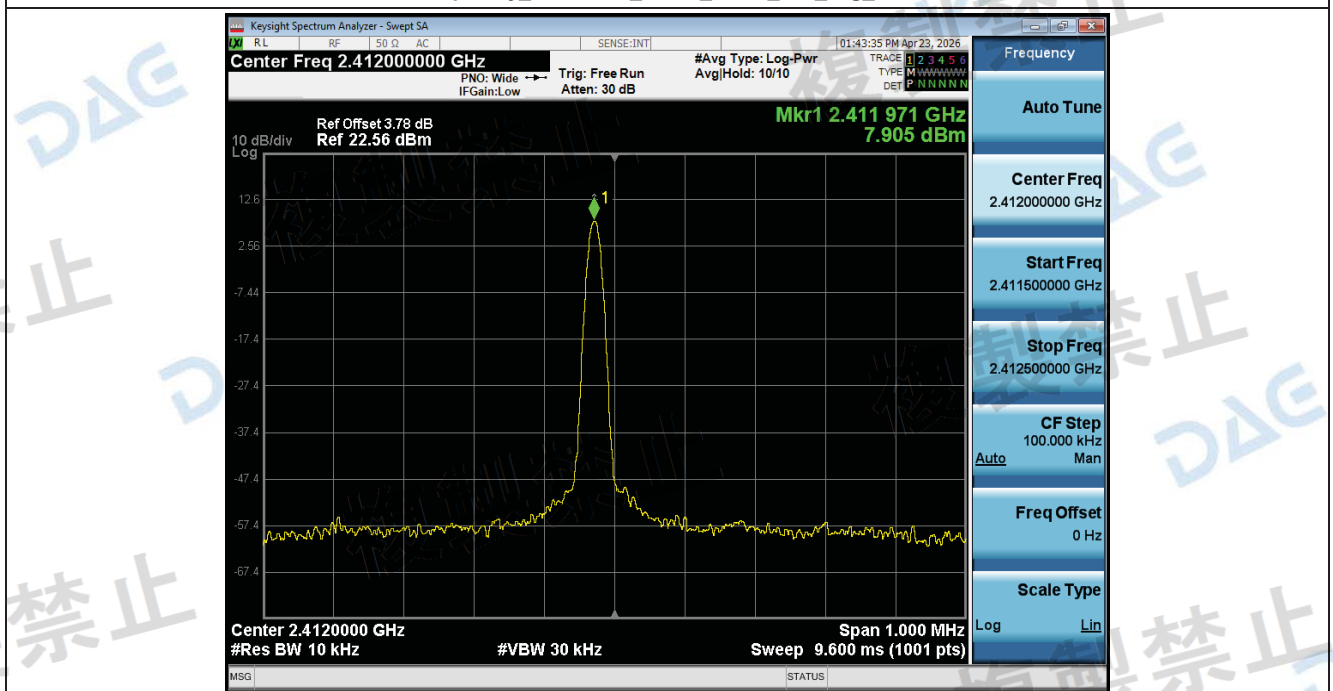
Frequency_Tolerance_NTLV_ANT1_802_11g_2412
