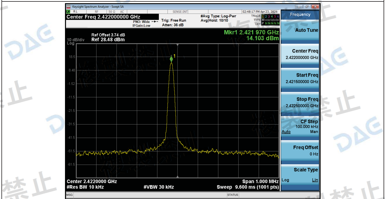
Frequency_Tolerance_NTHV_ANT1_802_11n(HT40)_2422
