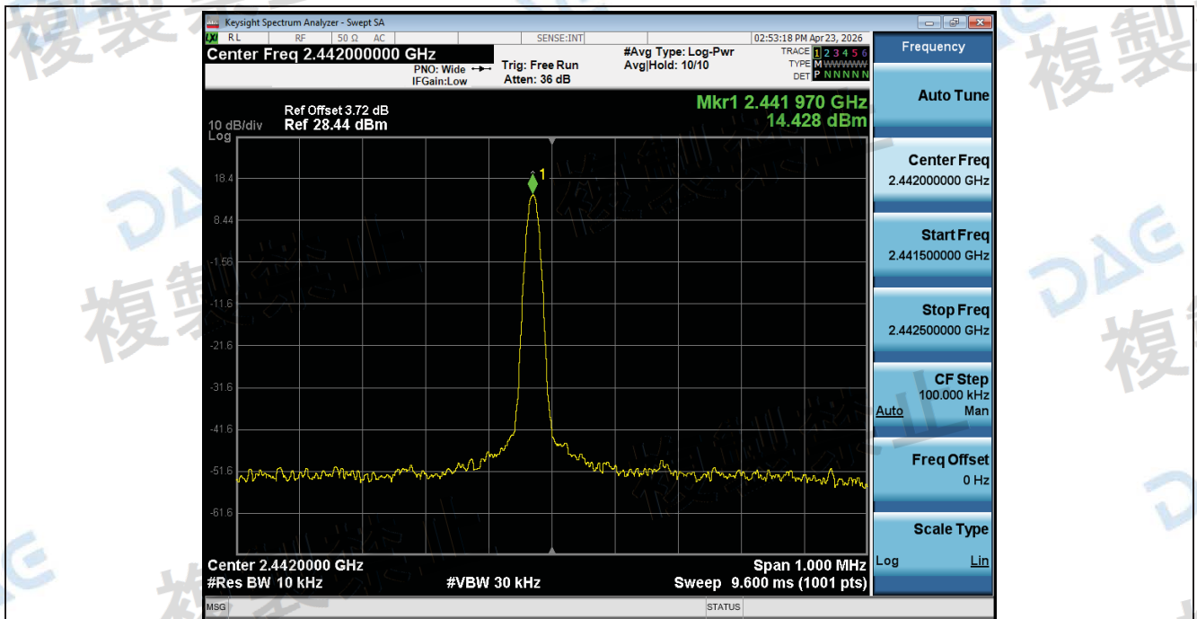
Frequency_Tolerance_NTHV_ANT1_802_11n(HT40)_2442
