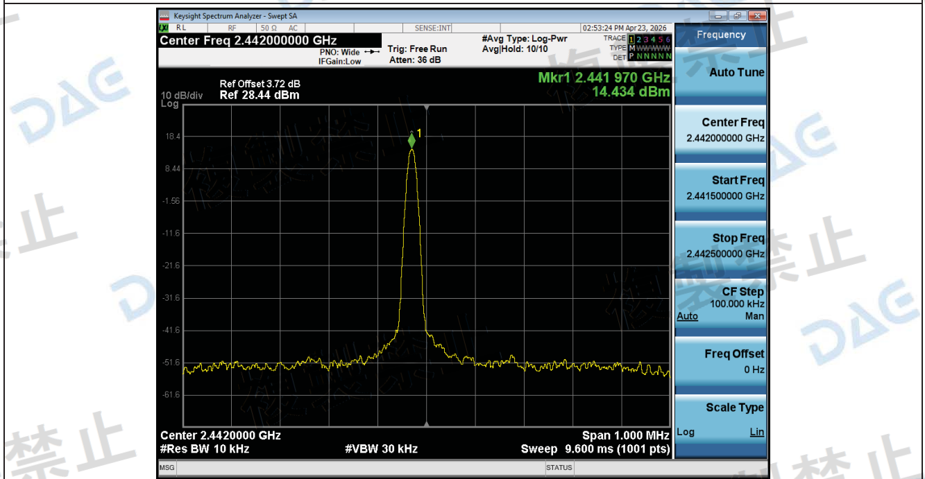
Frequency_Tolerance_NTHV_ANT1_802_11n(HT40)_2442
