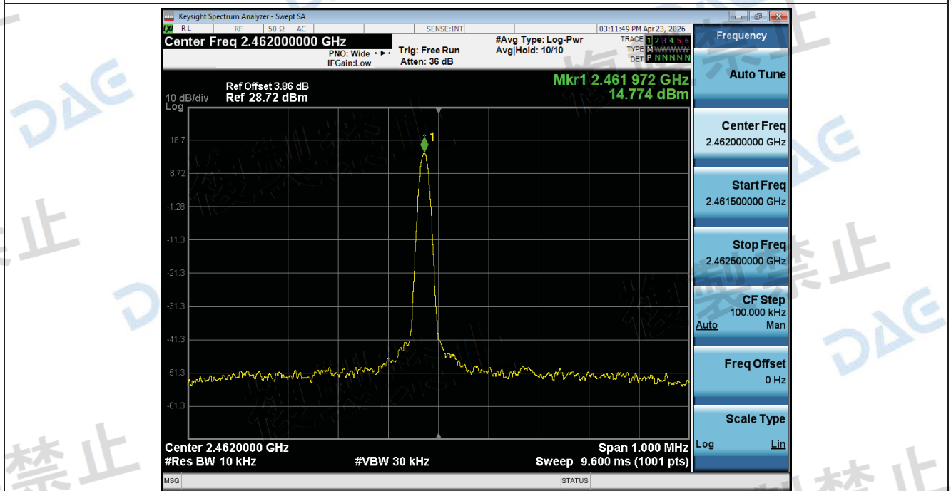
Frequency_Tolerance_NTHV_ANT1_802_11n(HT40)_2462
