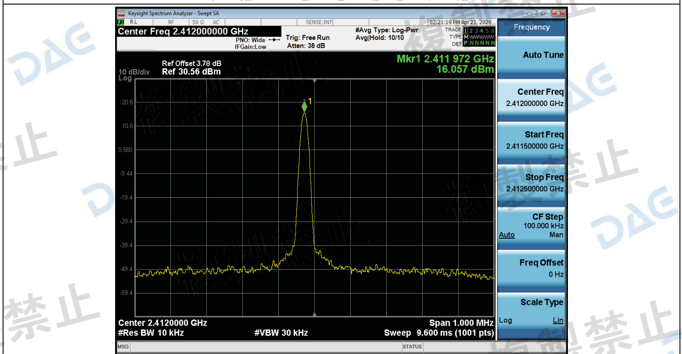
Frequency_Tolerance_NTLV_ANT1_802_11ax(HE20)_2412
