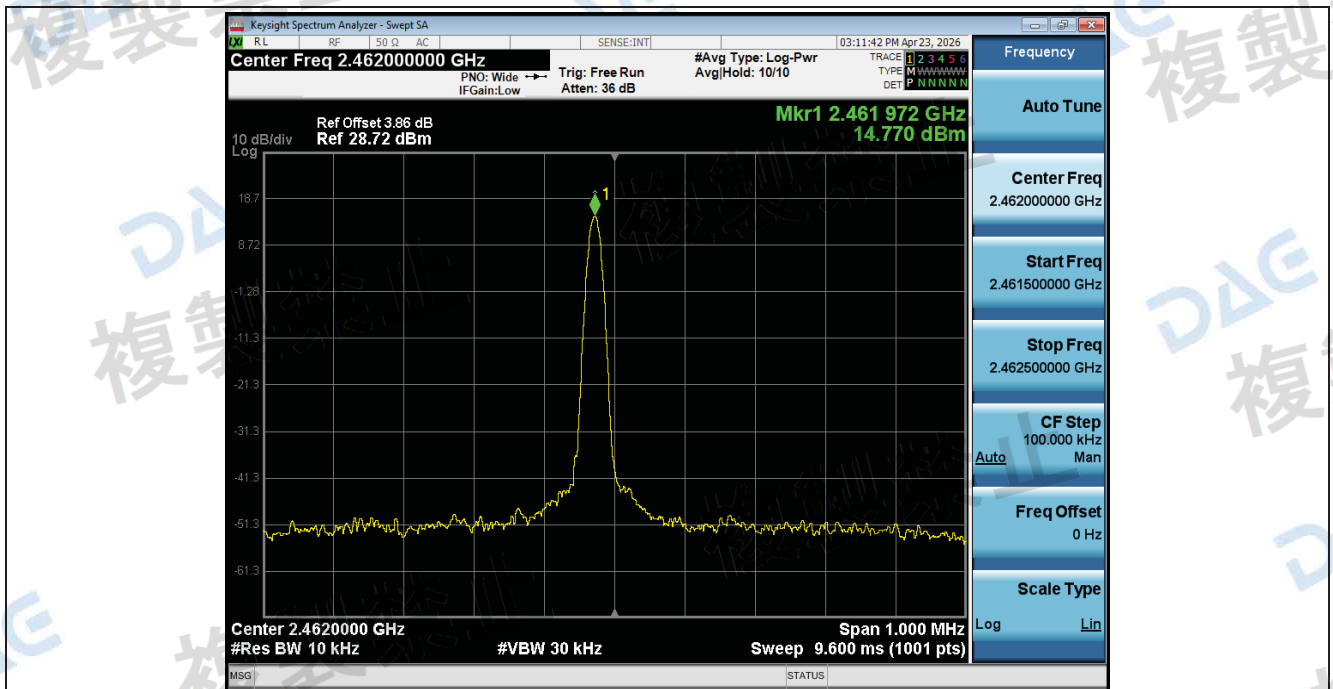
Frequency_Tolerance_NTLV_ANT1_802_11n(HT40)_2462
