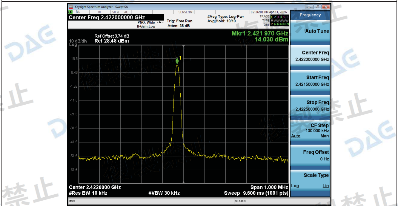
Frequency_Tolerance_NTHV_ANT1_802_11ax(HE40)_2422
