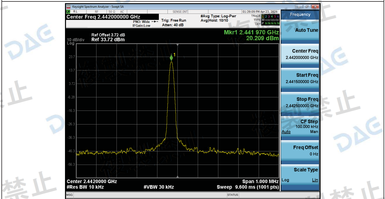
Frequency_Tolerance_NTHV_ANT1_802_11b_2442
