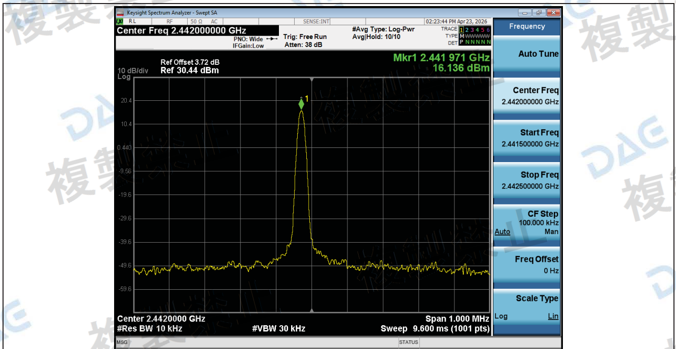
Frequency_Tolerance_NTLV_ANT1_802_11ax(HE20)_2442
