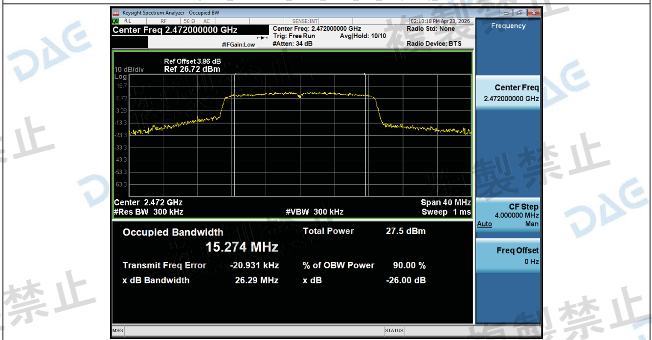
Spread_Bandwidth_NVNT_ANT1_802_11n(HT20)_2472
