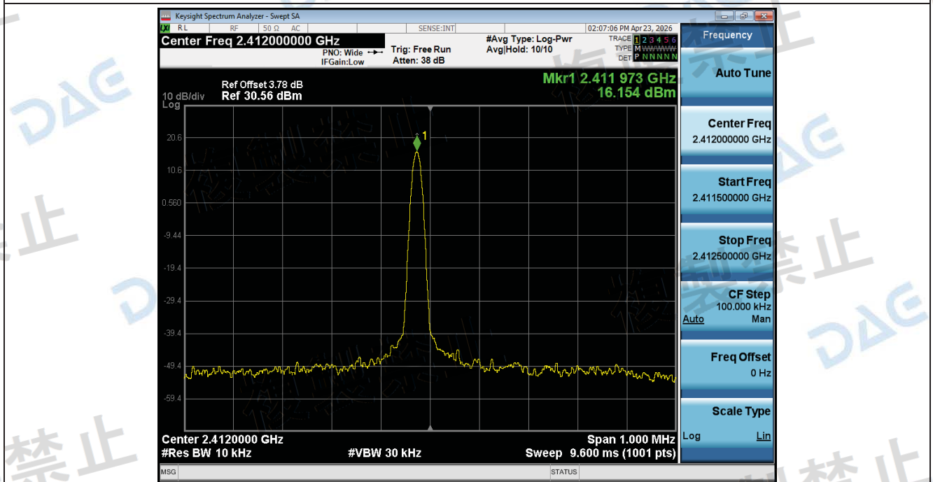
Frequency_Tolerance_NTHV_ANT1_802_11n(HT20)_2412
