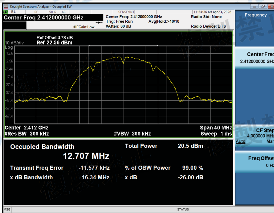
Occupied_Frequency_Bandwidth_NVNT_ANT1_802_11b_2412
