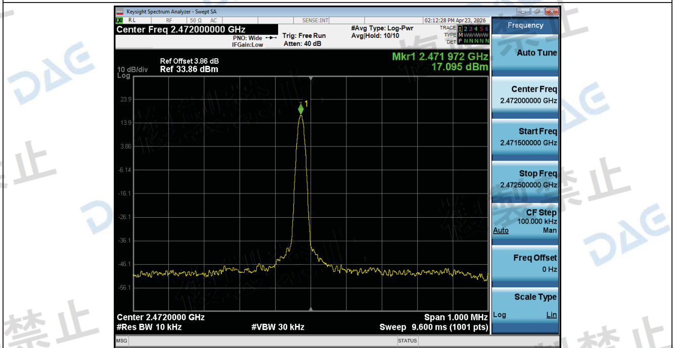
Frequency_Tolerance_NTHV_ANT1_802_11n(HT20)_2472
