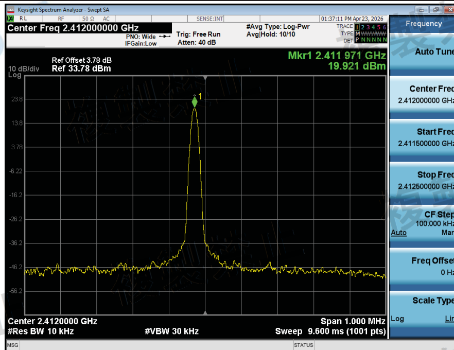
Frequency_Tolerance_NTHV_ANT1_802_11b_2412
