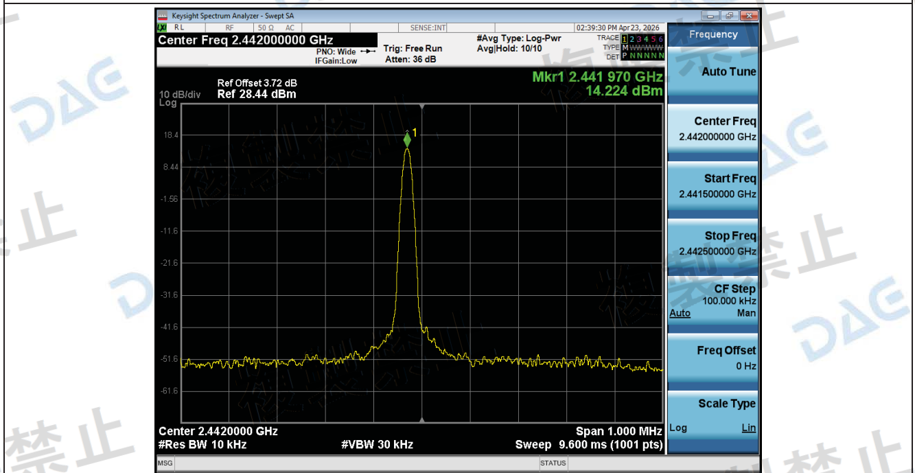
Frequency_Tolerance_NTHV_ANT1_802_11ax(HE40)_2442
