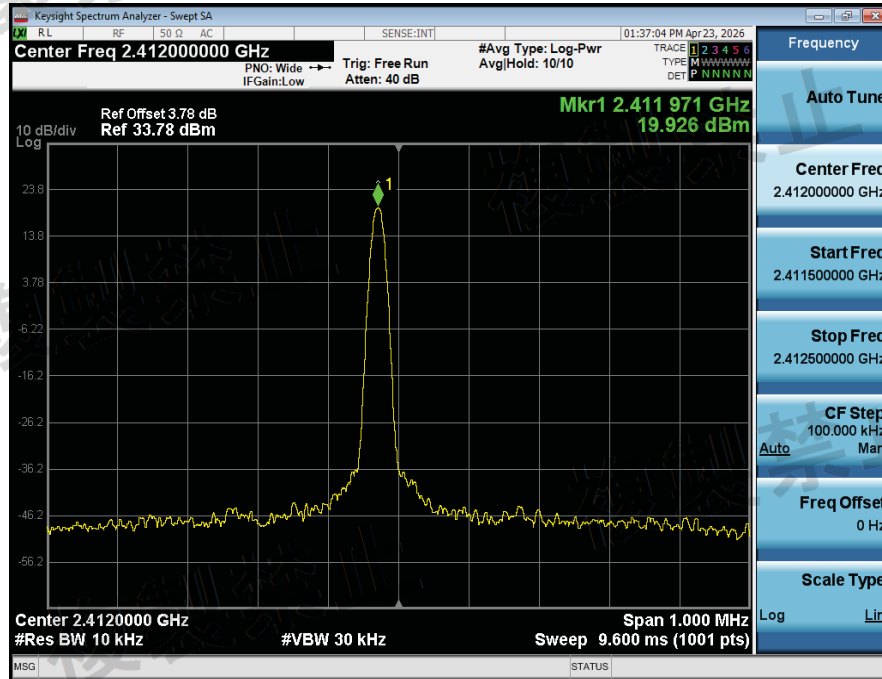
Frequency_Tolerance_NTLV_ANT1_802_11b_2412
