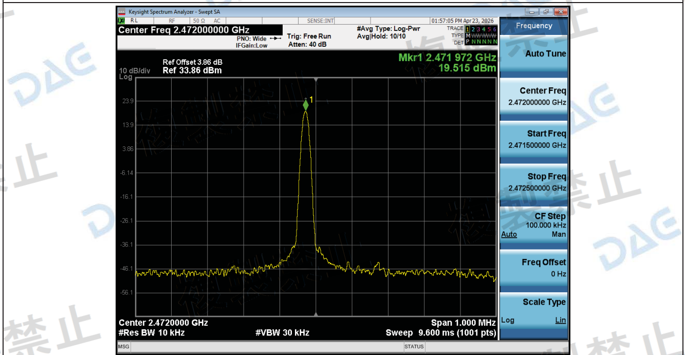
Frequency_Tolerance_NTHV_ANT1_802_11g_2472
