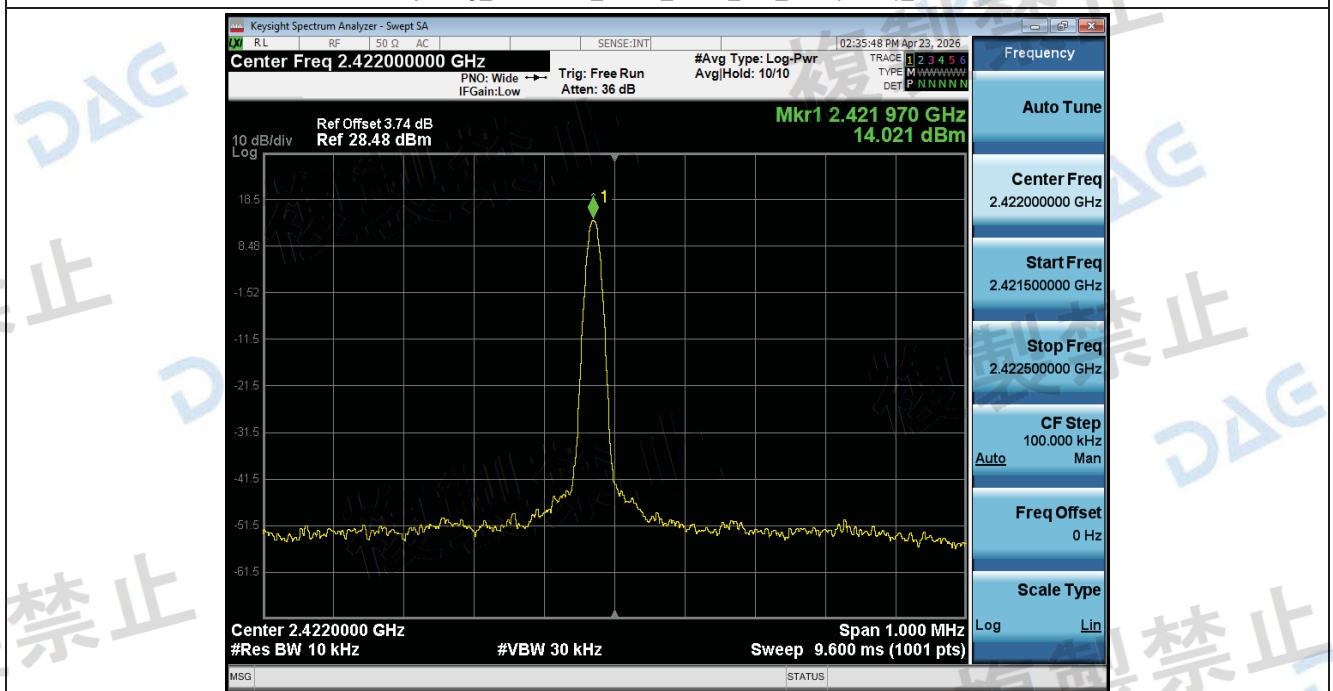
Frequency_Tolerance_NTLV_ANT1_802_11ax(HE40)_2422
