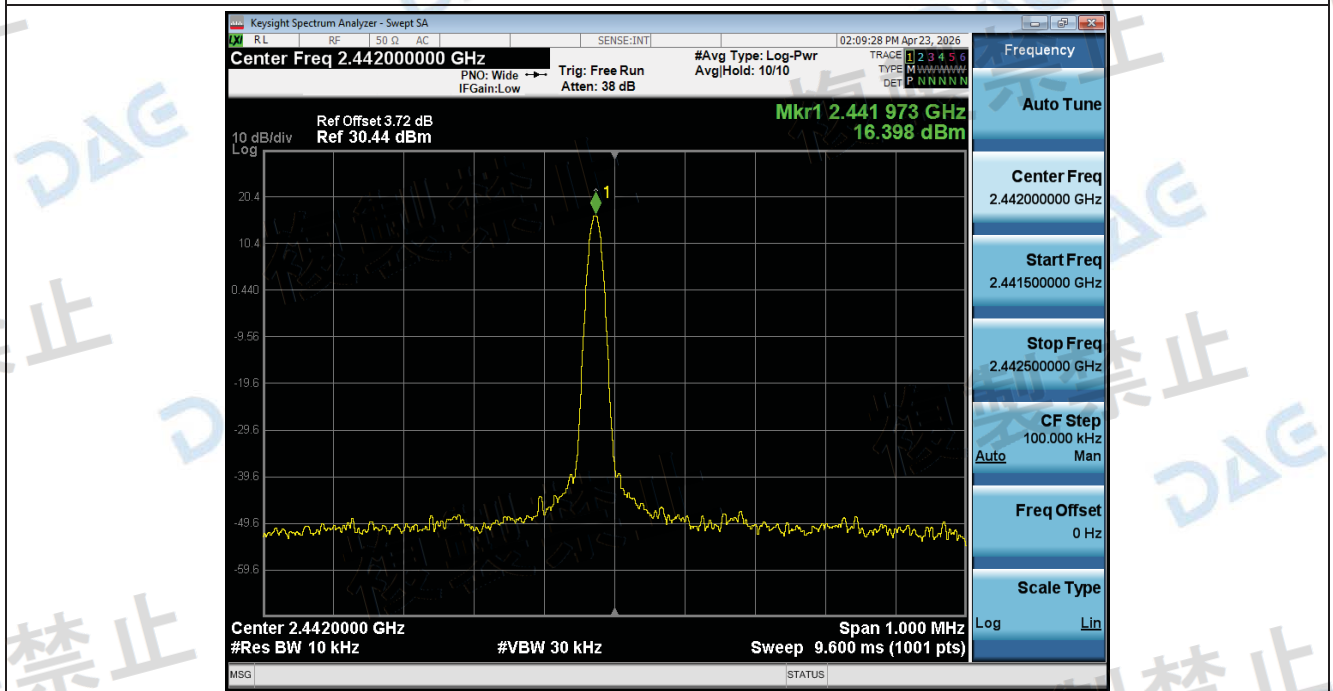
Frequency_Tolerance_NTHV_ANT1_802_11n(HT20)_2442
