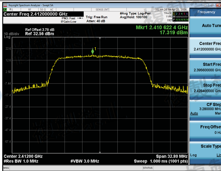
2_Antena_Power_NVNT_ANT1_802_11g_2412
