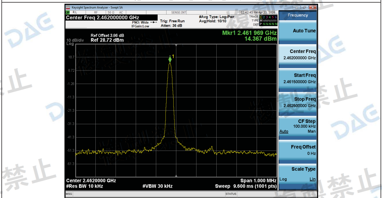
Frequency_Tolerance_NTLV_ANT1_802_11ax(HE40)_2462
