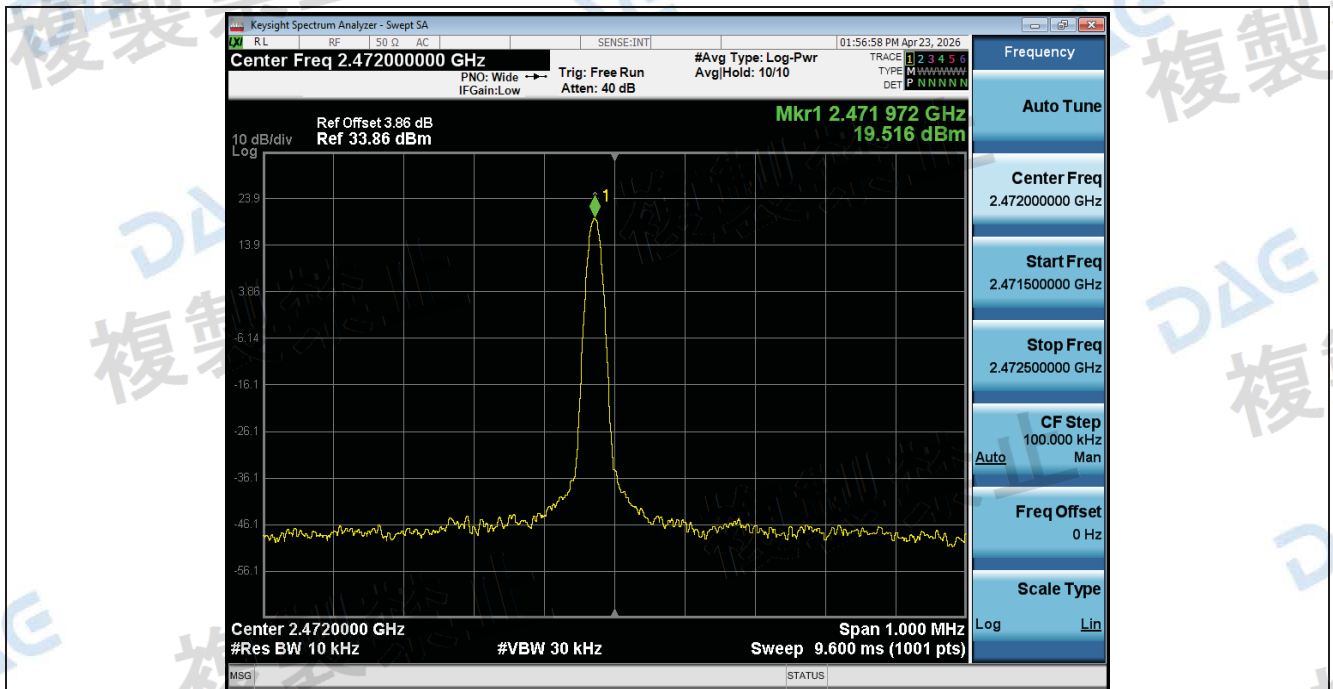
Frequency_Tolerance_NTHV_ANT1_802_11g_2472
