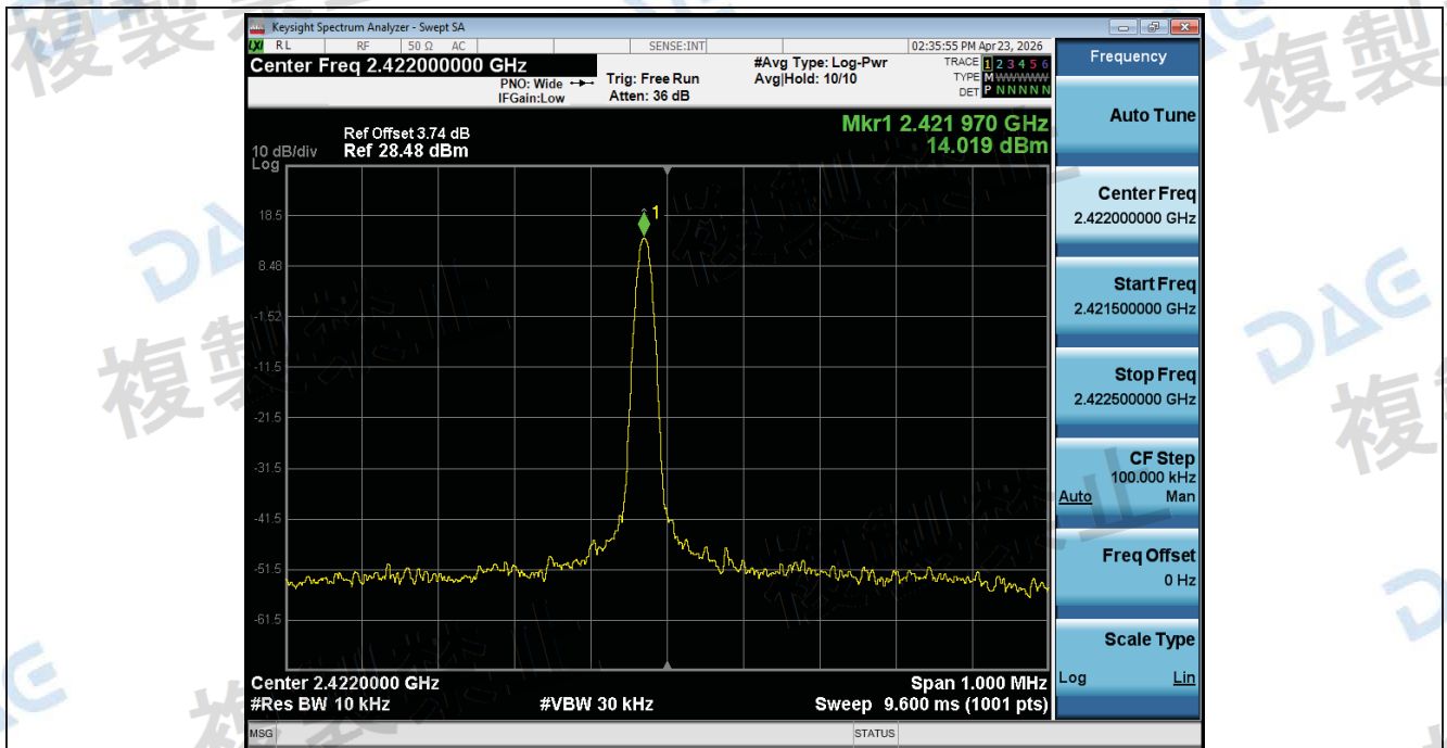
Frequency_Tolerance_NTHV_ANT1_802_11ax(HE40)_2422
