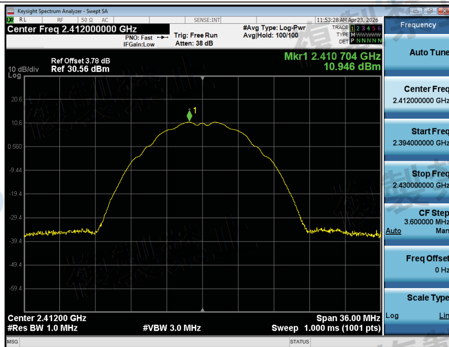
2_Antenna_Power_NVNT_ANT1_802_11b_2412
