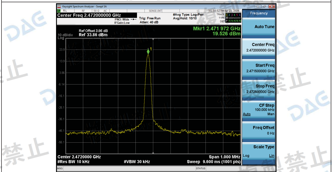
Frequency_Tolerance_NTLV_ANT1_802_11g_2472
