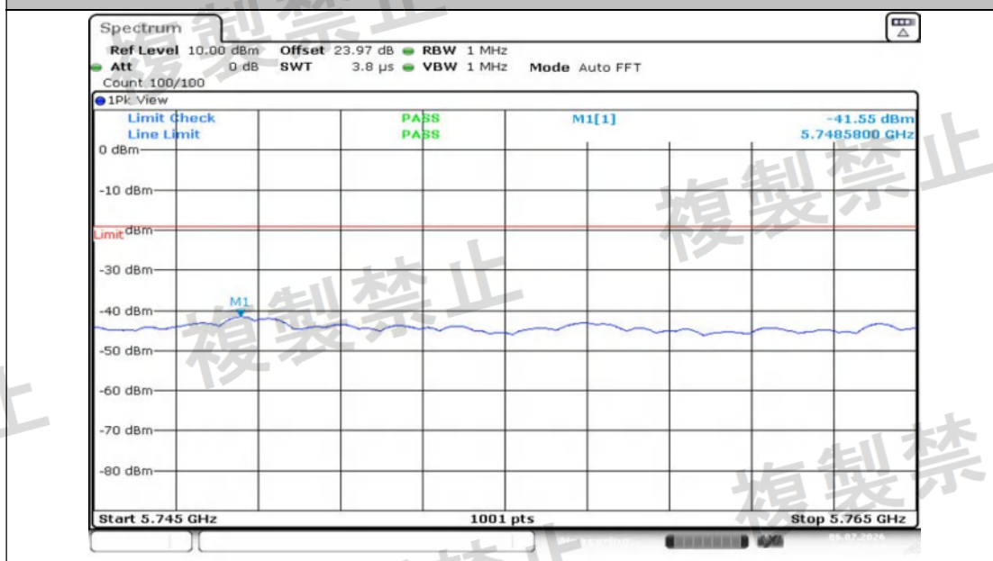
NTNV-11N20MIMO-Ant2-5700-5745~5765-PASS
