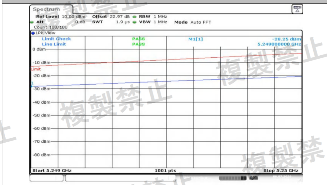
NTNV-11N40MIMO-Ant2-5270-5249~5250-PASS
