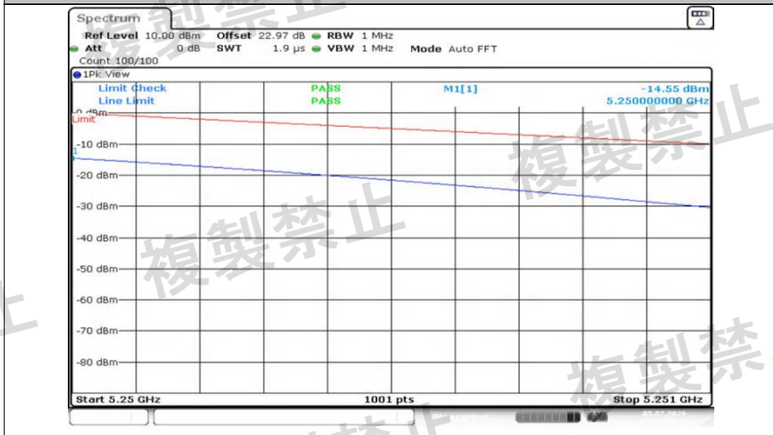
NTNV-11N20MIMO-Ant2-5240-5250~5251-PASS
