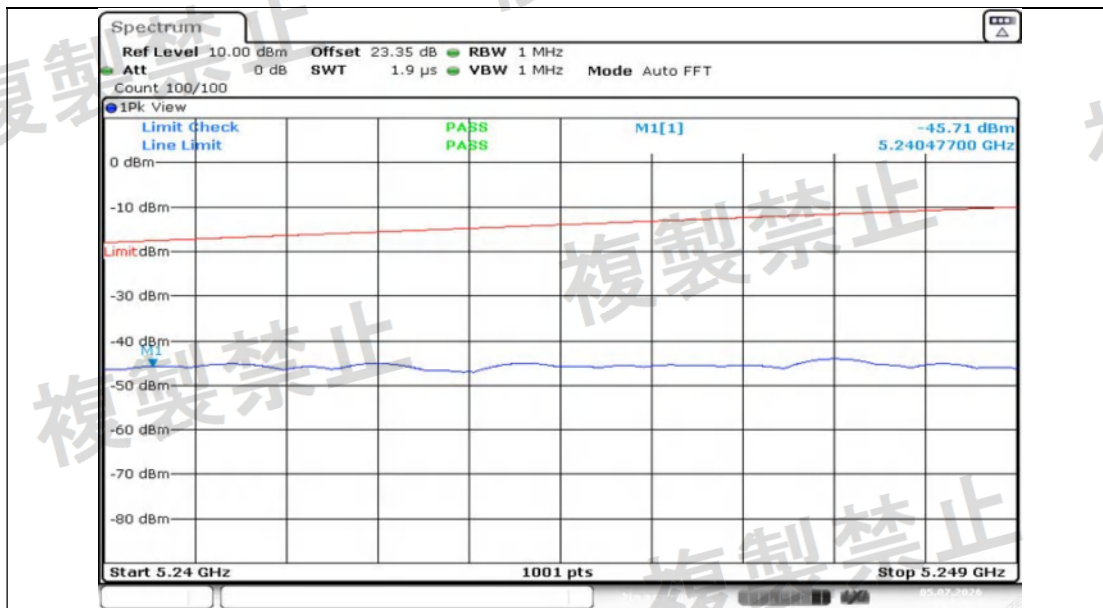
NTNV-11N20MIMO-Ant1-5320-5240~5249-PASS
