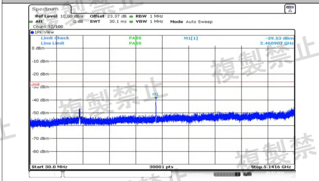
NTNV-11N40MIMO-Ant2-5190-30~5141.6-PASS
