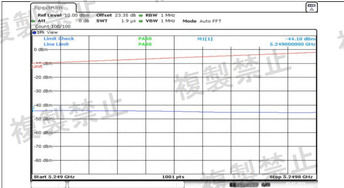
NTNV-11N20MIMO-Ant1-5280-5249~5249.8-PASS
