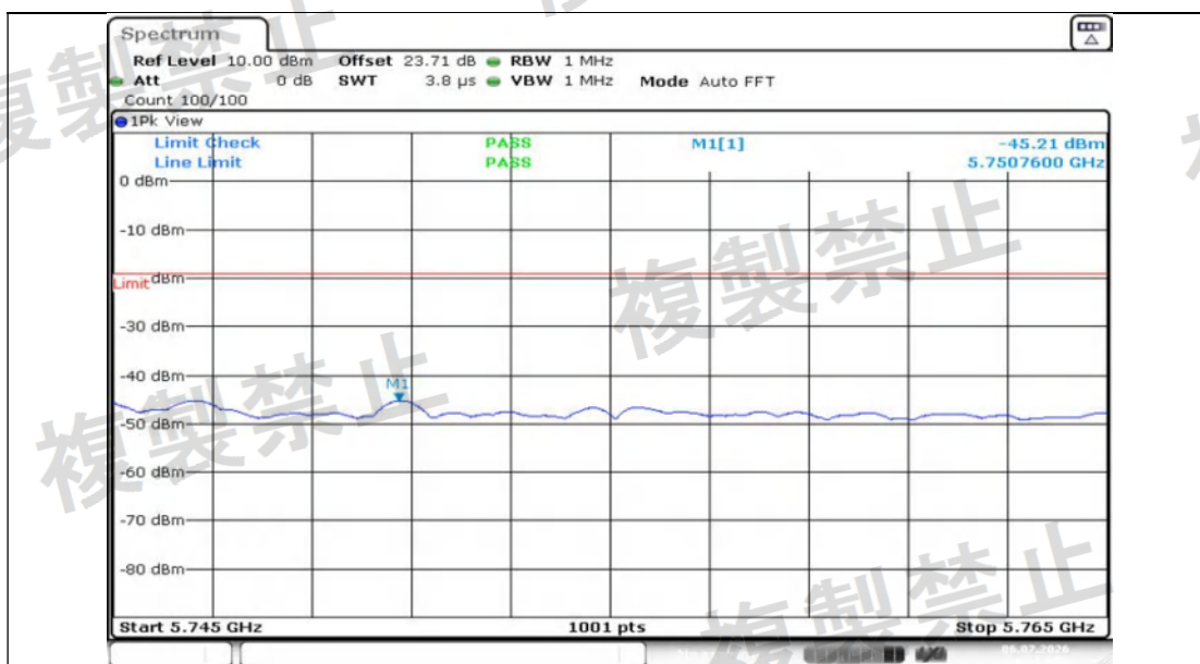
NTNV-11N20MIMO-Ant1-5700-5745~5765-PASS
