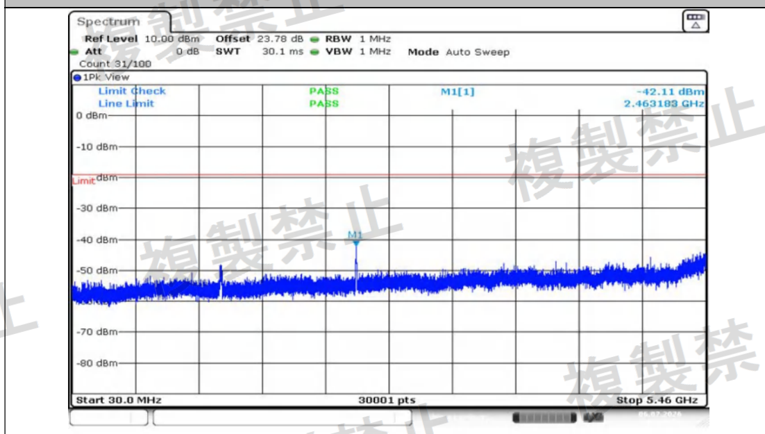
NTNV-11N40MIMO-Ant2-5510-30~5460-PASS
