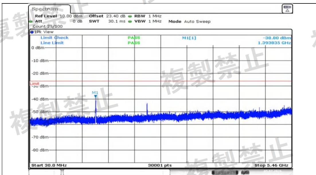
NTNV-11N20MIMO-Ant1-5600-30~5460-PASS
