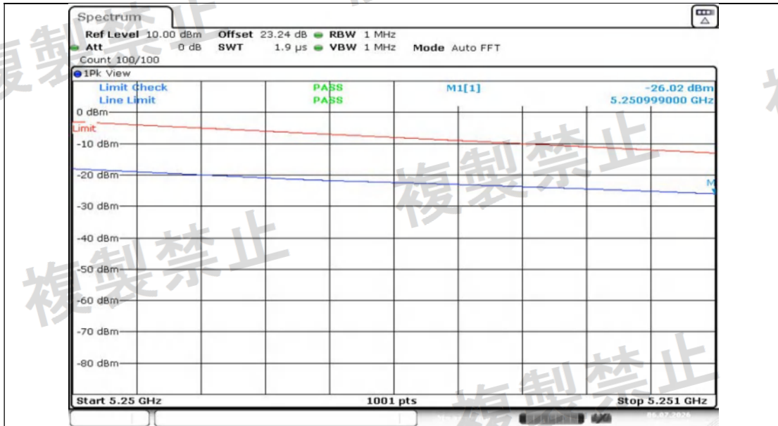
NTNV-11N40MIMO-Ant1-5230-5250-5251-PASS
