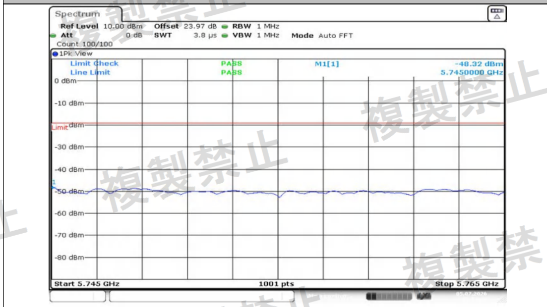
NTNV-11N20MIMO-Ant2-5500-5745~5765-PASS
