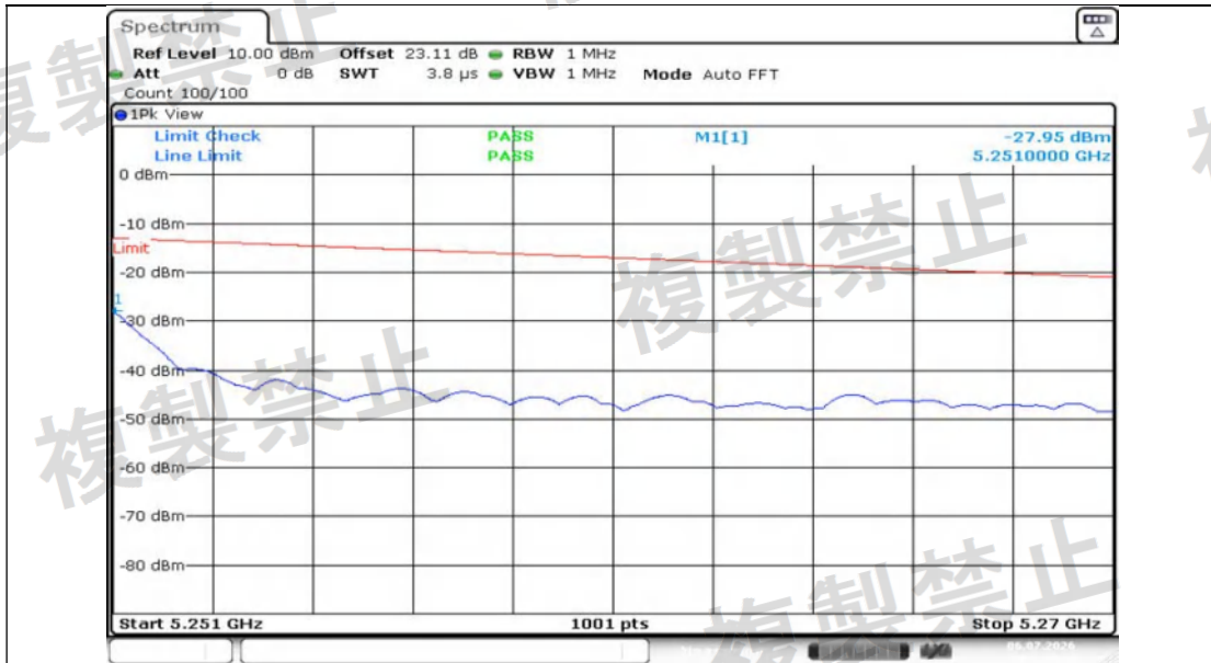
NTNV-11N40MIMO-Ant1-5230-5251~5270-PASS
