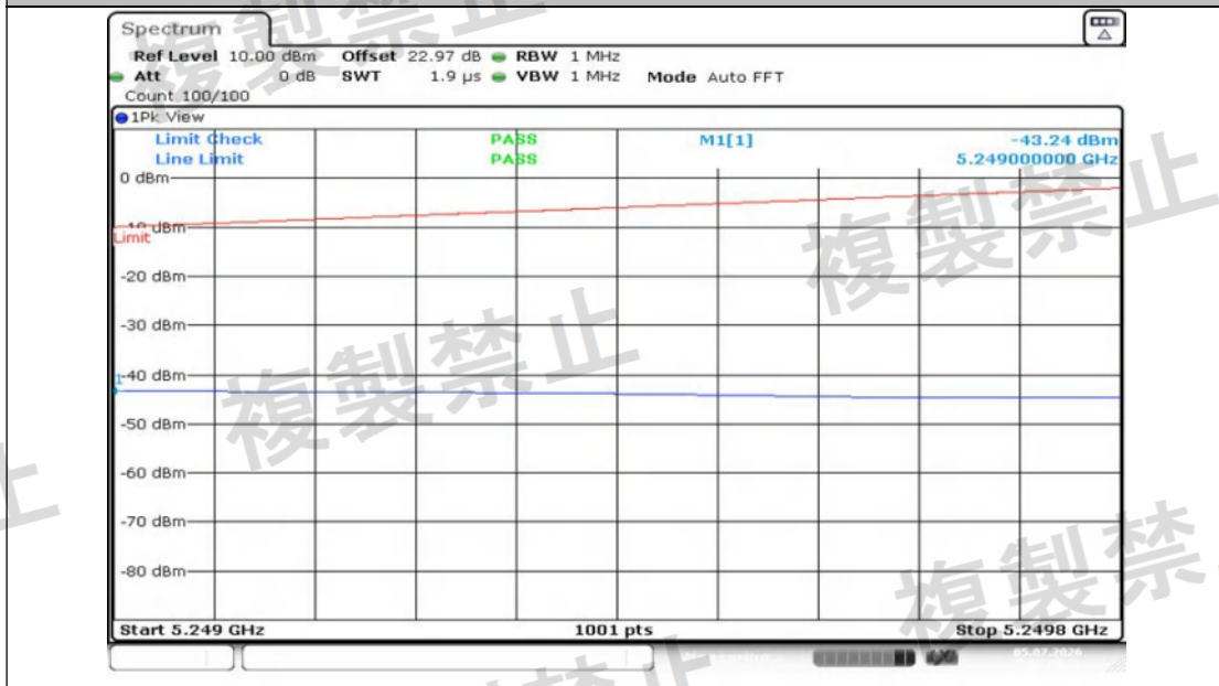
NTNV-11N20MIMO-Ant2-5320-5249~5249.8-PASS
