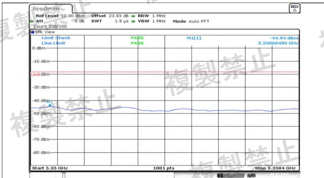
NTVN-11N40MIMO-Ant1-5310-5350~5358.4-PASS
