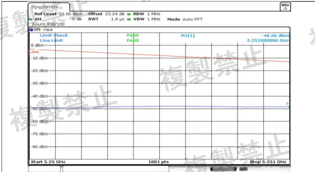
NTNV-11N40MIMO-Ant1-5190-5250~5251-PASS
