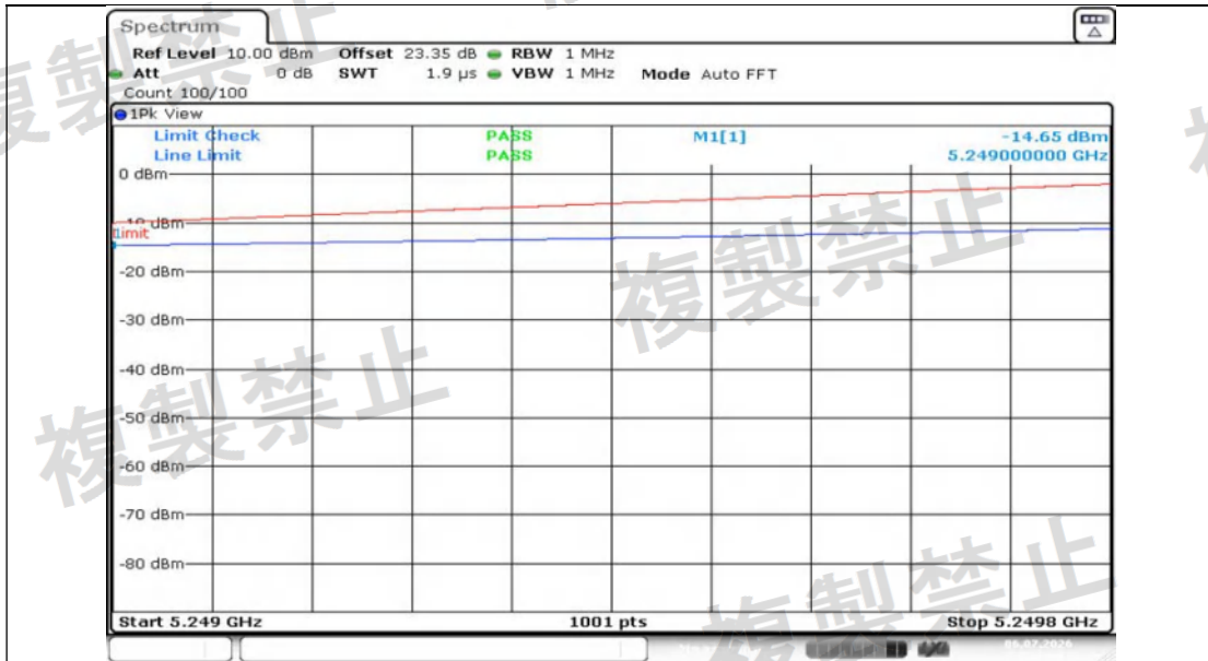
NTNV-11N20MIMO-Ant1-5260-5249~5249.8-PASS
