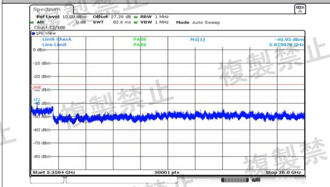
NTNV-11N40MIMO-Ant2-5310-5358.4~26000-PASS
