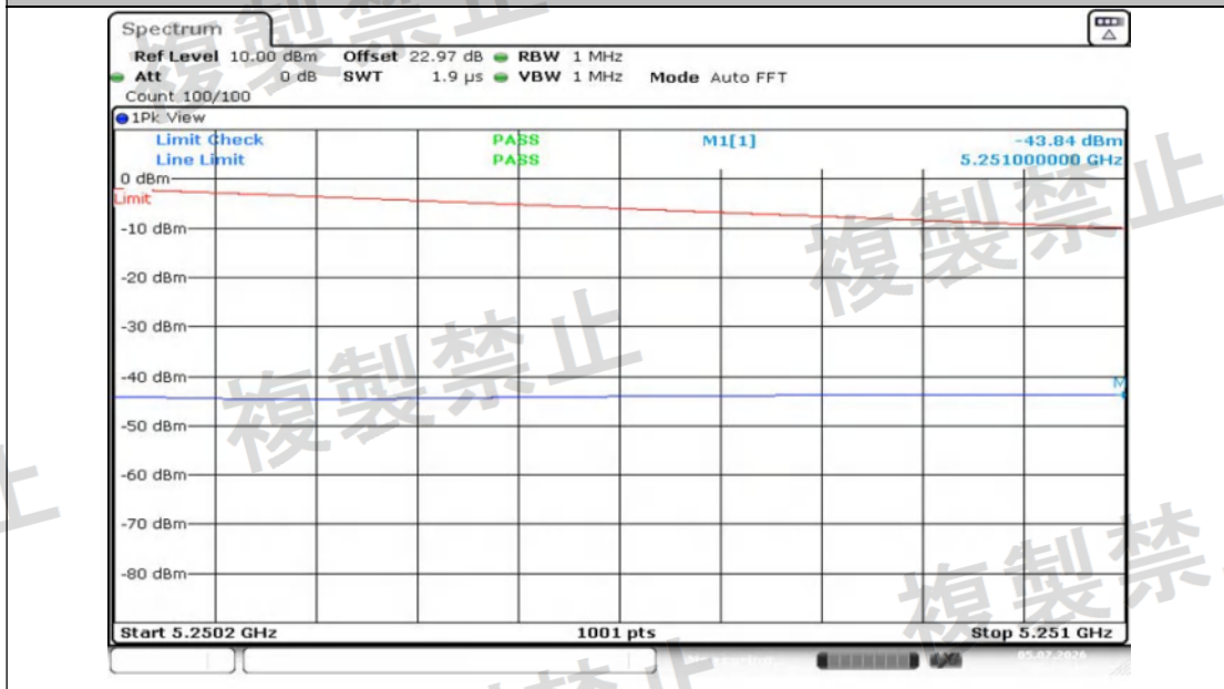
NTNV-11N20MIMO-Ant2-5200-5250.2~5251-PASS
