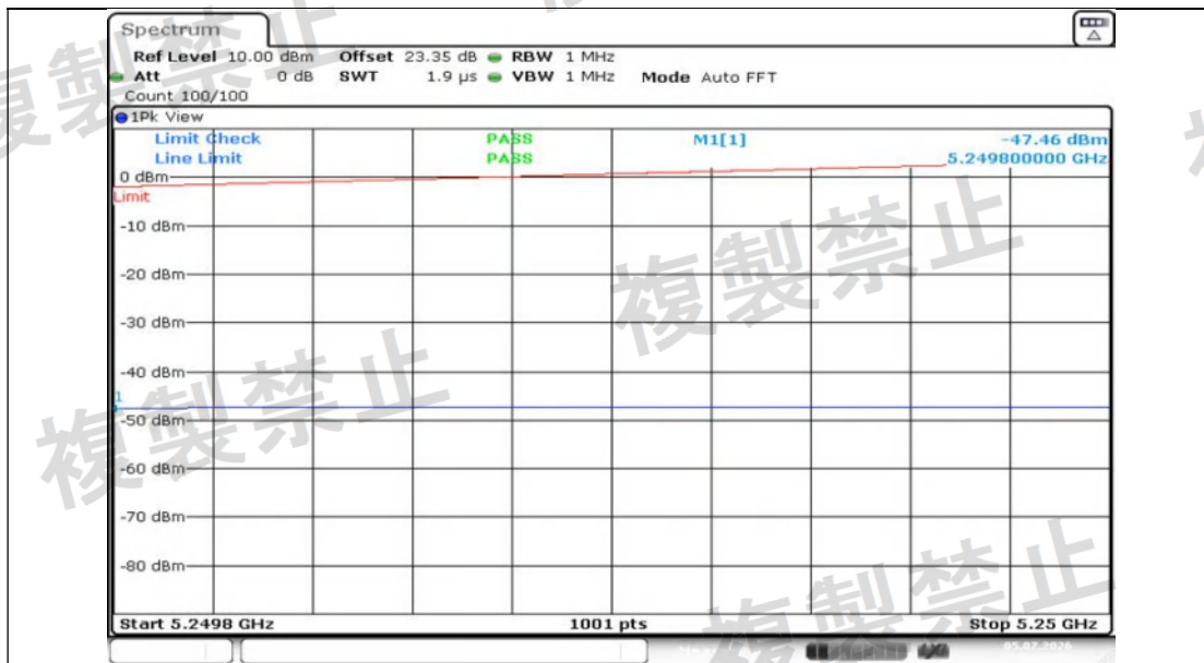
NTNV-11N20MIMO-Ant1-5320-5249.8~5250-PASS
