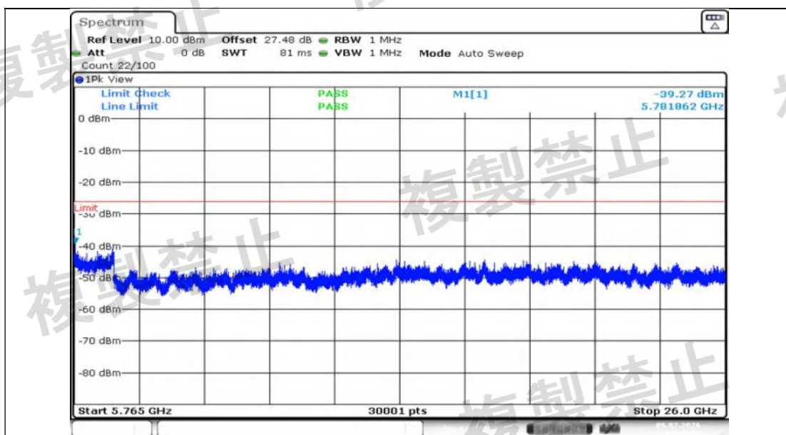
NTNV-11N20MIMO-Ant1-5700-5765~26000-PASS
