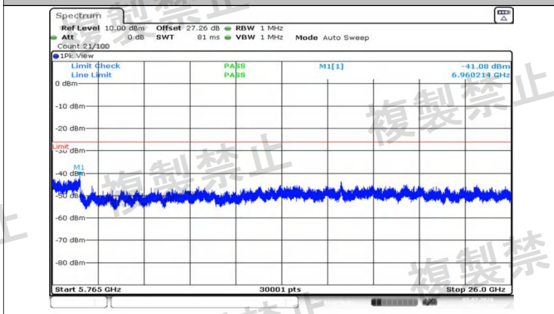
NTNV-11N20MIMO-Ant2-5600-5765~26000-PASS
