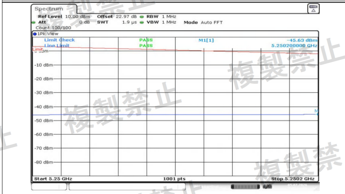
NTNV-11N20MIMO-Ant2-5200-5250~5250.2-PASS
