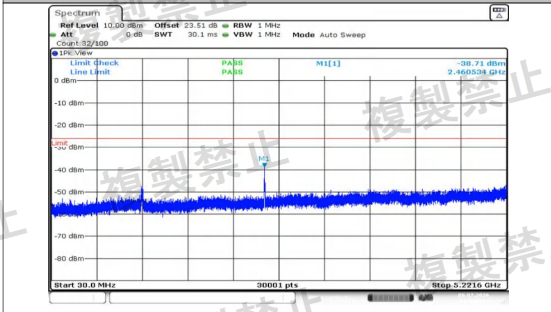
NTNV-11N40MIMO-Ant2-5270-30~5221.6-PASS
