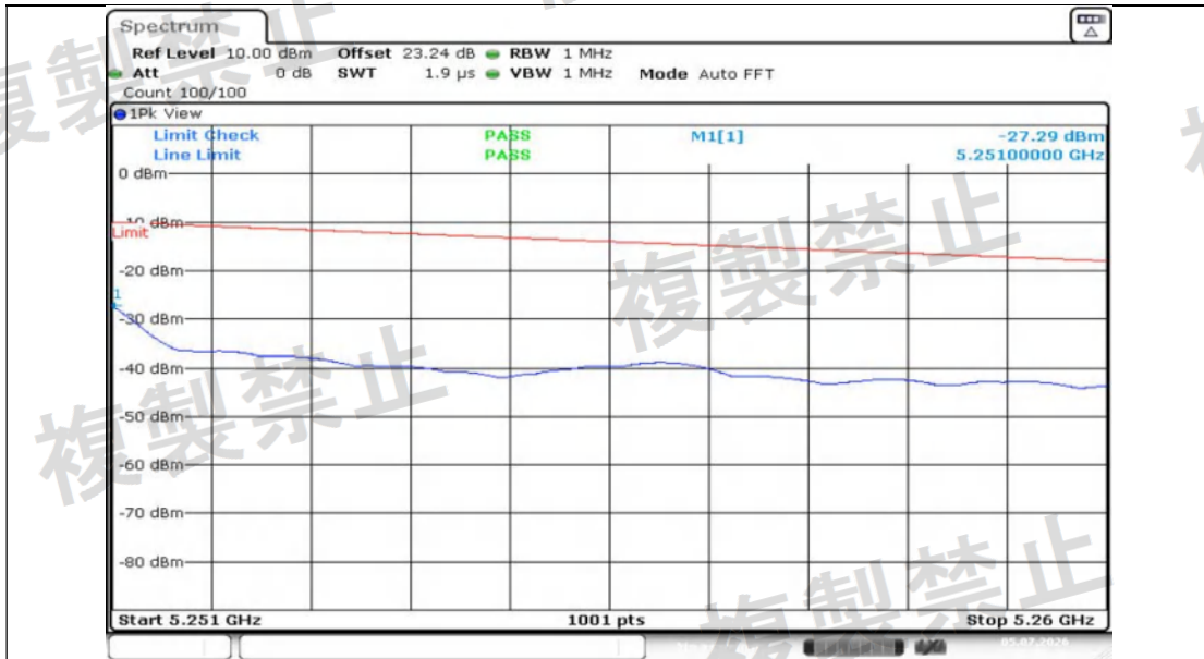
NTNV-11N20MIMO-Ant1-5240-5251~5260-PASS
