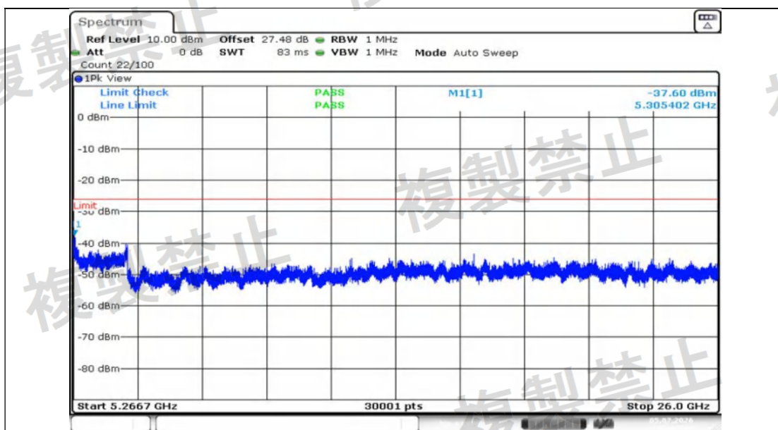
NTNV-11N20MIMO-Ant1-5240-5266.7~26000-PASS
