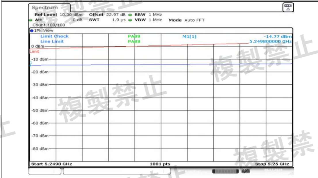
NTNV-11N20MIMO-Ant2-5260-5249.8~5250-PASS
