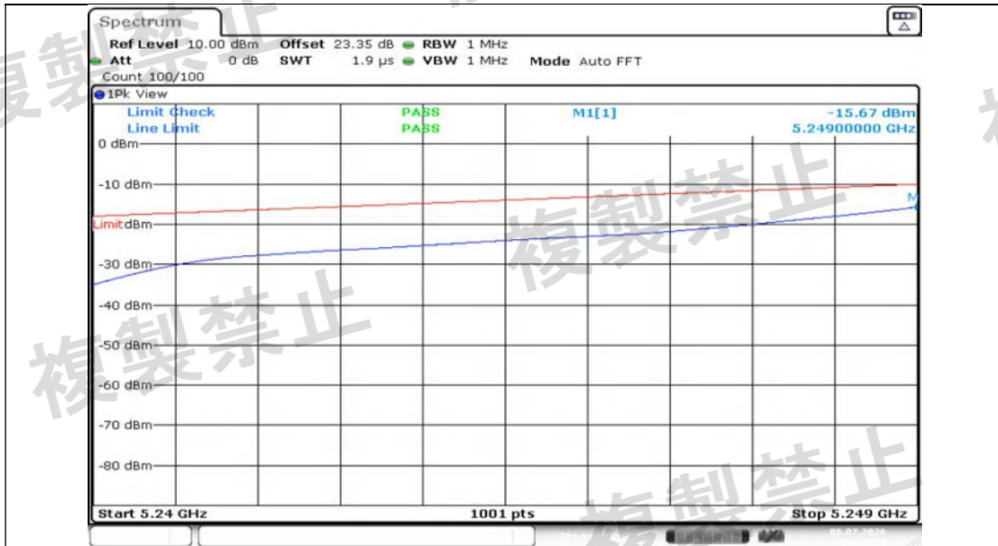
NTNV-11N20MIMO-Ant1-5260-5240~5249-PASS
