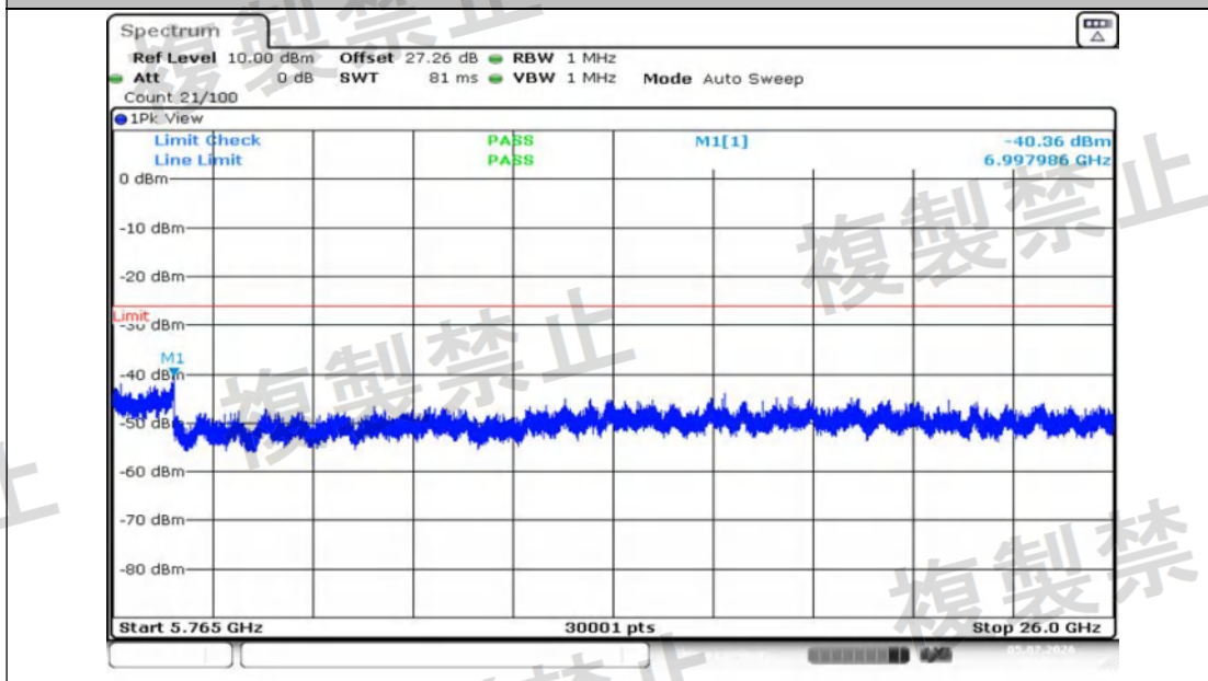
NTNV-11N20MIMO-Ant2-5500-5765~26000-PASS
