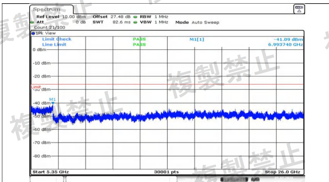
NTNV-11N20MIMO-Ant1-5280-5350~26000-PASS
