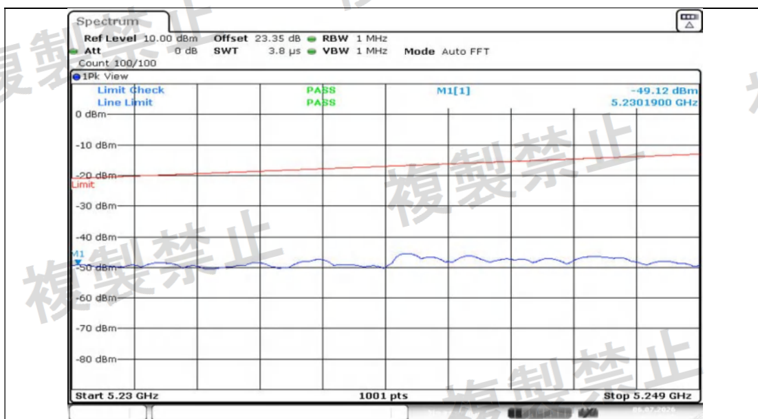
NTNV-11N40MIMO-Ant1-5310~5230~5249-PASS
