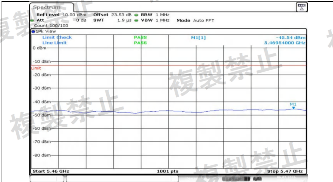
NTNV-11N40MIMO-Ant1-5510-5460~5470-PASS
