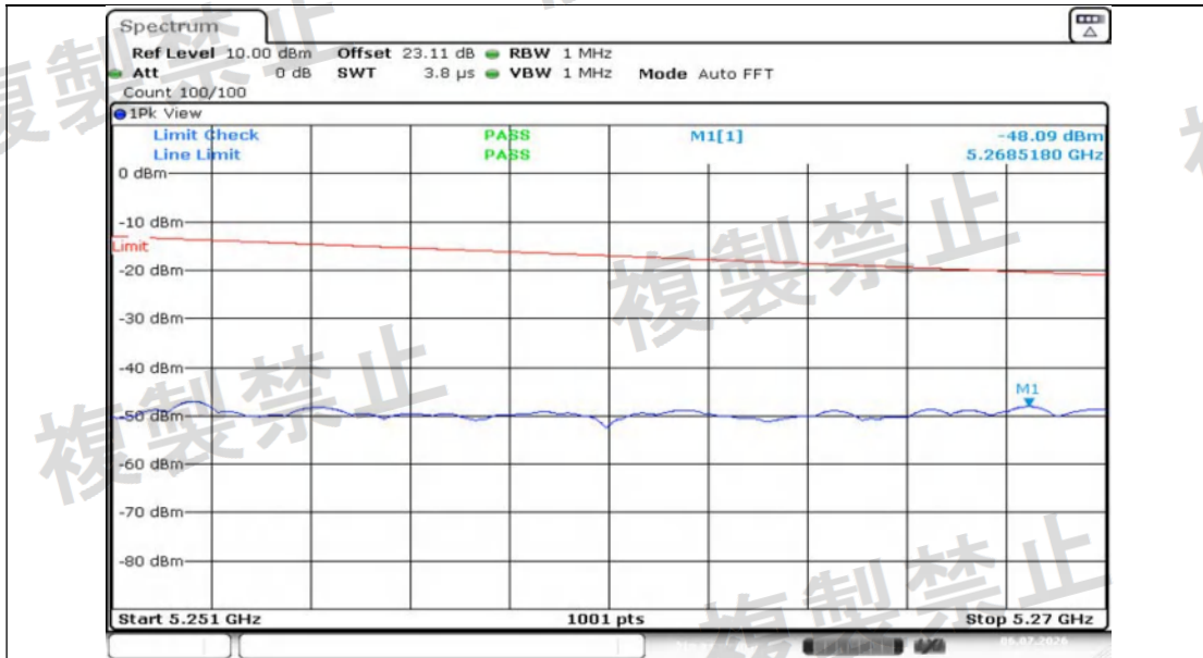
NTNV-11N40MIMO-Ant1-5190-5251~5270-PASS
