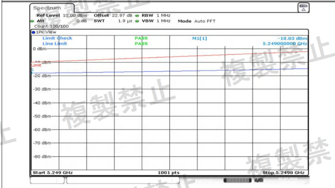
NTNV-11N20MIMO-Ant2-5260-5249~5249.8-PASS
