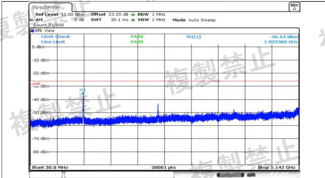
NTNV-11N20MIMO-Ant1-5240-30~5142-PASS
