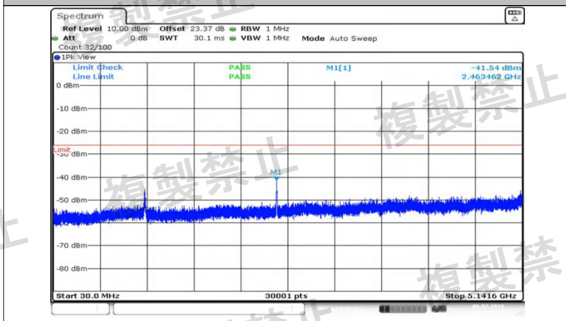
NTNV-11N40MIMO-Ant2-5230-30~5141.6-PASS
