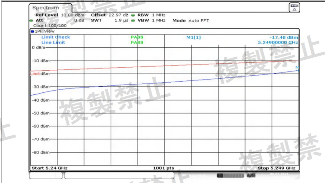
NTNV-11N20MIMO-Ant2-5260-5240~5249-PASS
