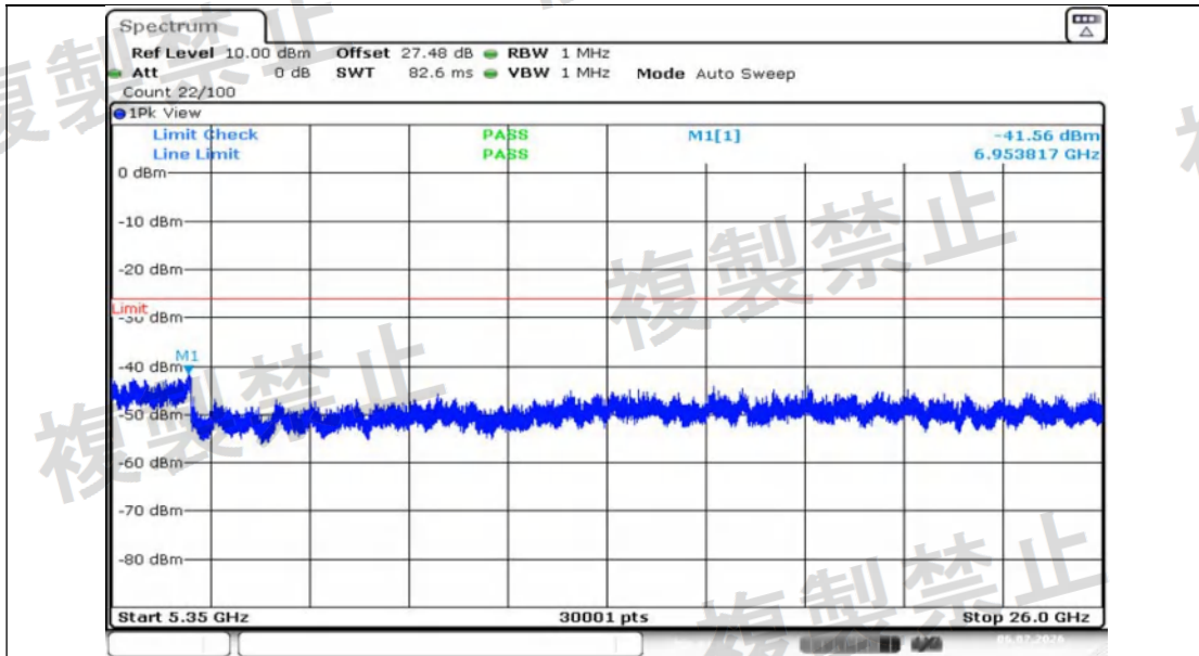
NTVN-11N20MIMO-Ant1-5260-5350~26000-PASS
