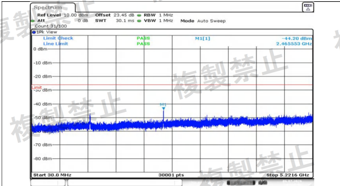
NTNV-11N40MIMO-Ant1-5310-30~5221.6-PASS
