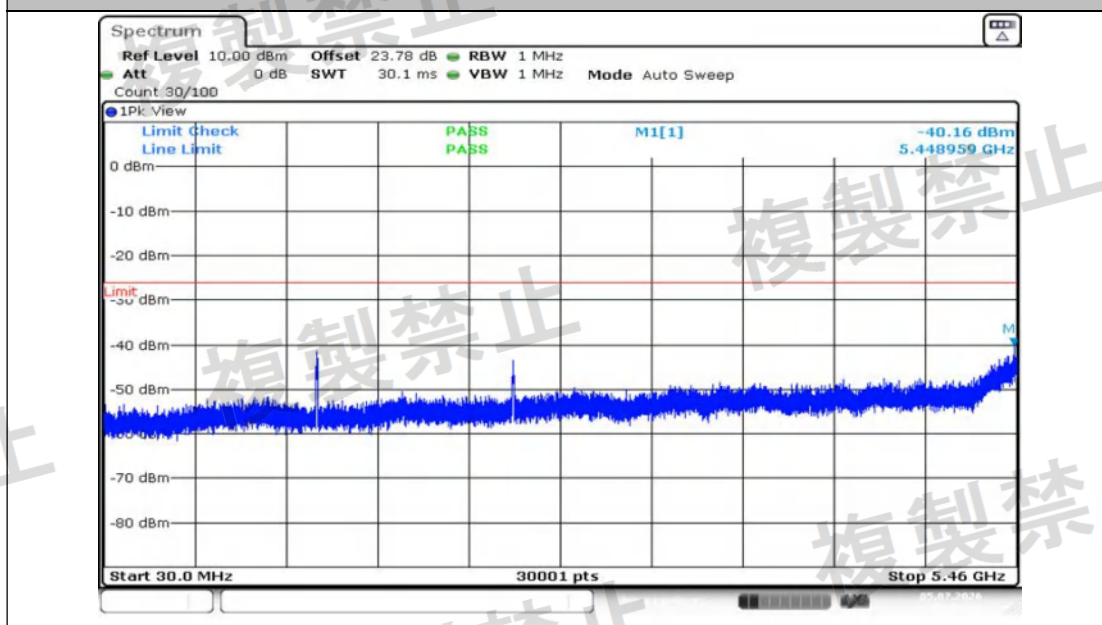
NTNV-11N20MIMO-Ant2-5500-30~5460-PASS
