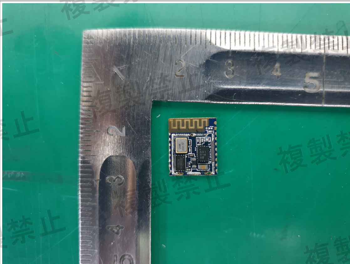
Bluetooth Module(BLE)_Shield Can Removal (Top)
