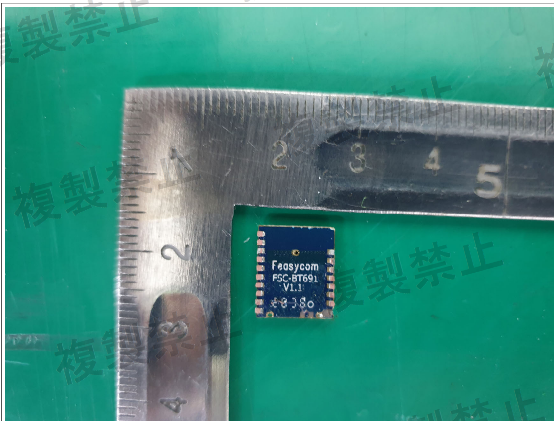
Bluetooth Module(BLE)_Shield Can Removal (Bottom)
