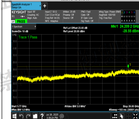
NTNV-11AX20MIMO-Ant10-5720-30~5460-PASS
