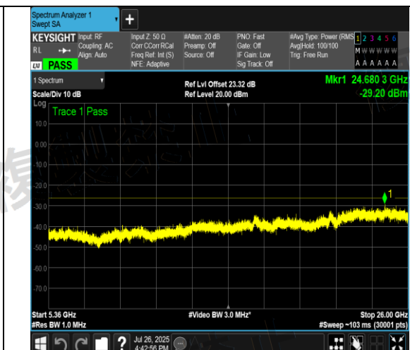
NTNV-11AX40MIMO-Ant7-5310-30~5221.6-PASS
