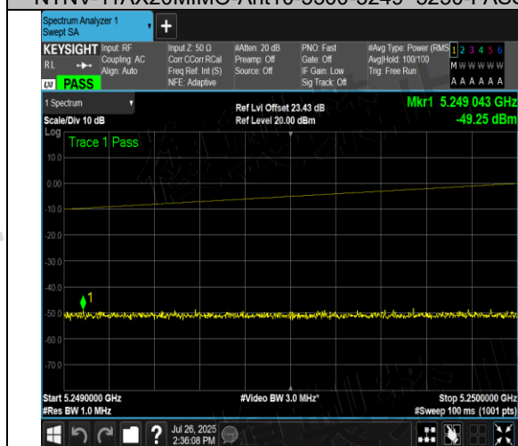
NTNV-11AX20MIMO-Ant10-5300-5249~5250-PASS
