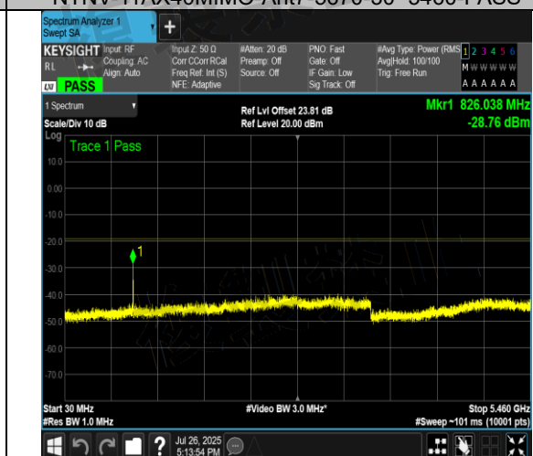
NTNV-11AX40MIMO-Ant7-5670-5460~5470-PASS
