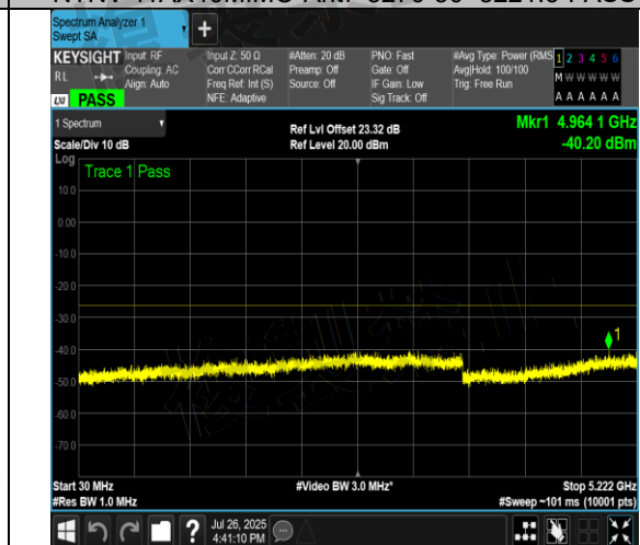
NTNV-11AX40MIMO-Ant7-5270-5221.6~5230-PASS
