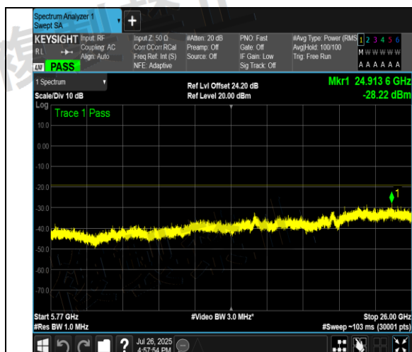
NTNV-11AX40MIMO-Ant10-5550-30~5460-PASS
