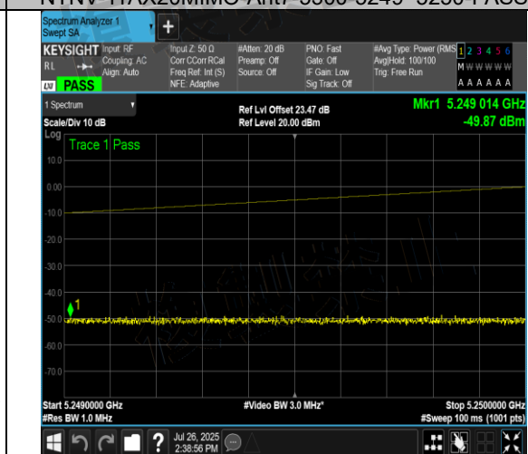
NTNV-11AX20MIMO-Ant7-5300-5249~5250-PASS
