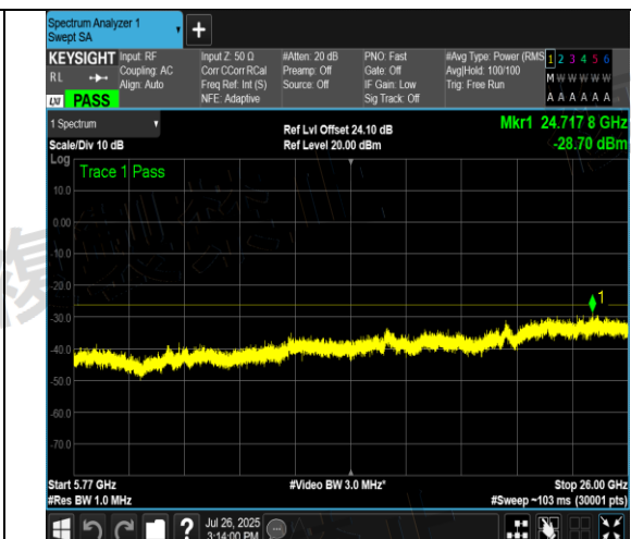
NTNV-11AX20MIMO-Ant7-5600-30~5460-PASS
