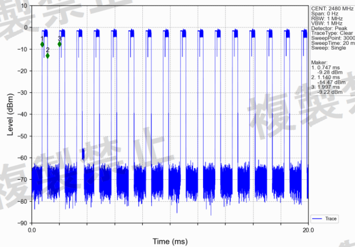
8DPSK_3DH1_2480MHz_Ant1_NTNV
