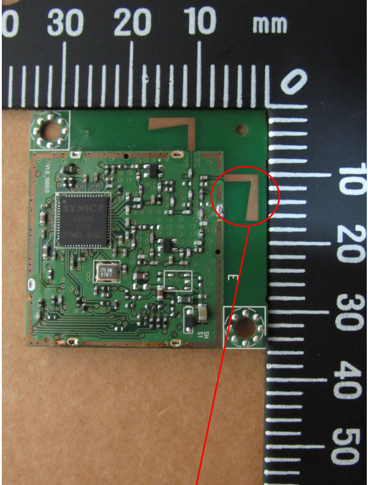
PCB Printed Antenna / Gain: 2.17 dBi
