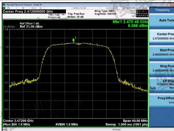
NTNV-11N20SISO-Ant1-2472-PASS
