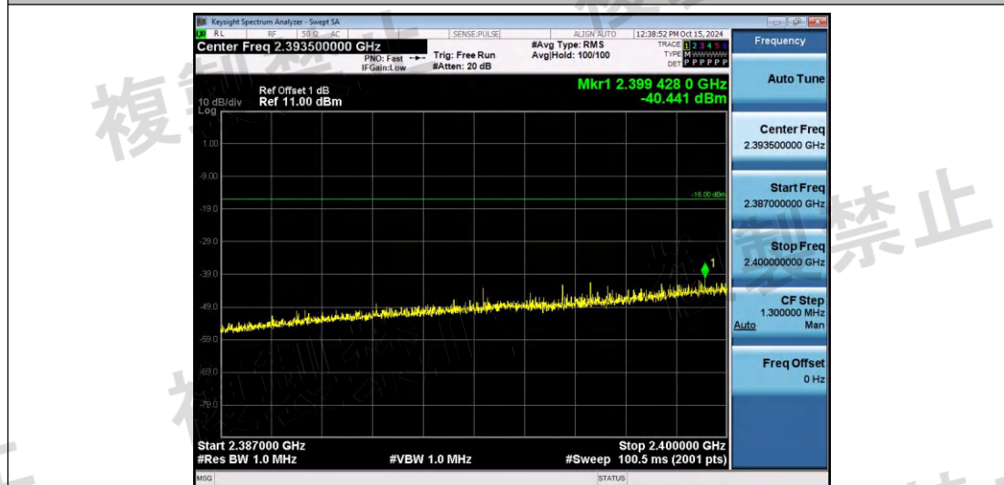
NTVN-11N40SISO-Ant1-2442-2387~2400-PASS
