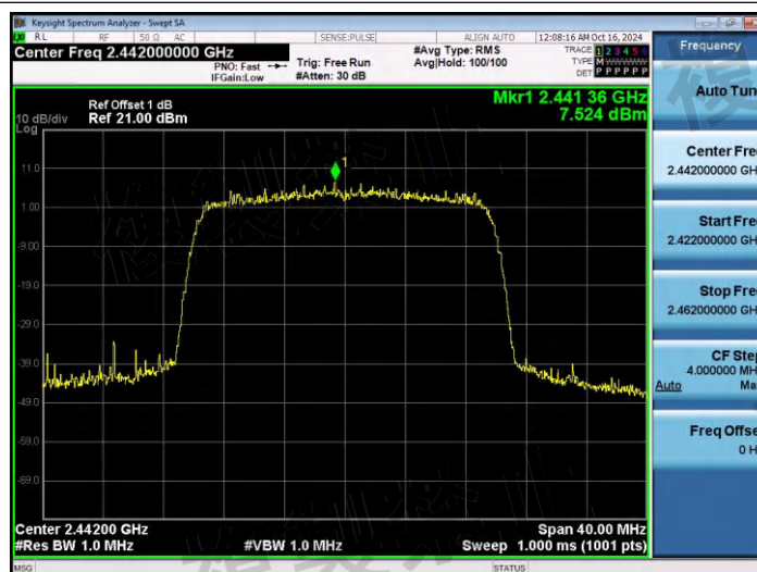
NTNV-11AX20SISO-Ant1-2442-PASS
