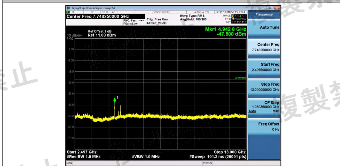
NTNV-11G-Ant1-2472-2496.5~13000-PASS
