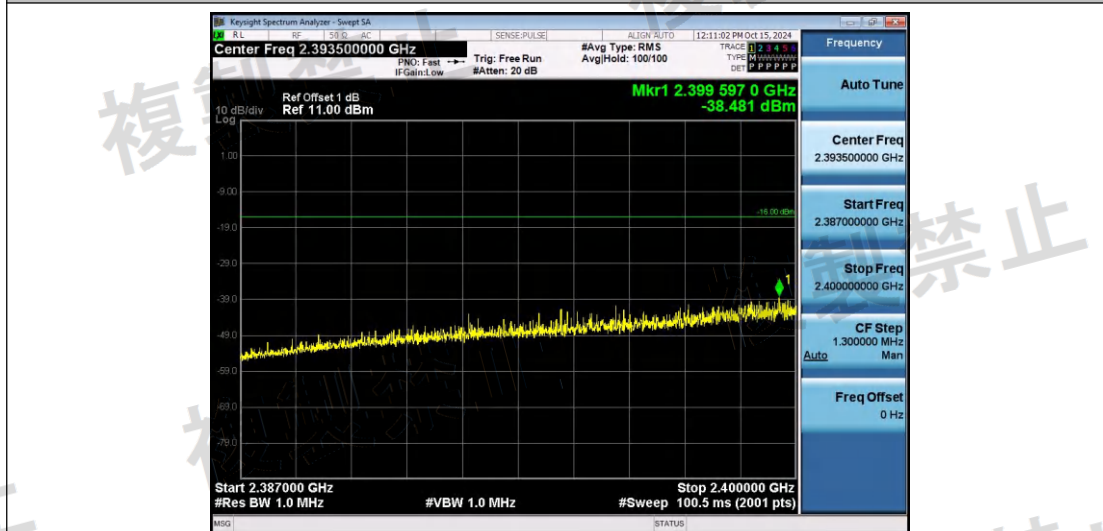
NTNV-11AX40SISO-Ant1-2442-2387~2400-PASS
