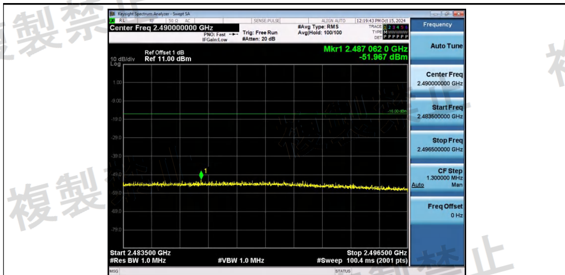
NTNV-11B-Ant1-2412-2483.5~2496.5-PASS
