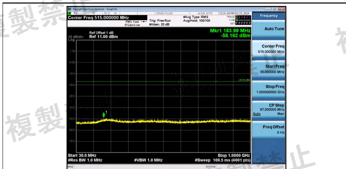
NTNV-11N20SISO-Ant1-2412-30~1000-PASS
