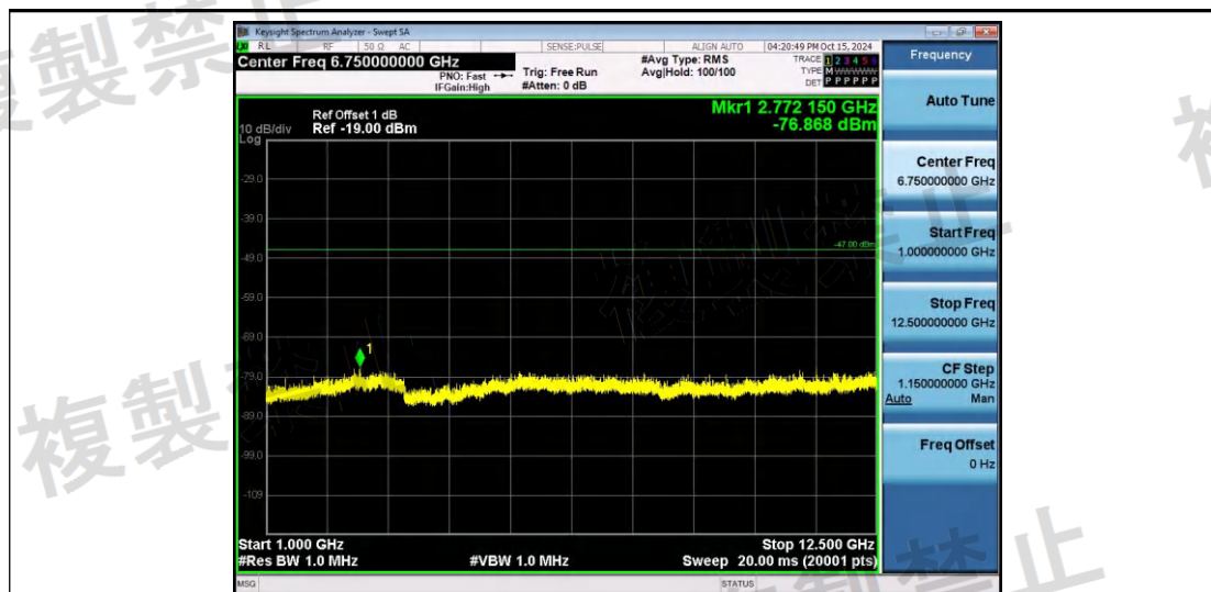
NTNV-11AX40SISO-Ant1-2442-1000~12500-PASS
