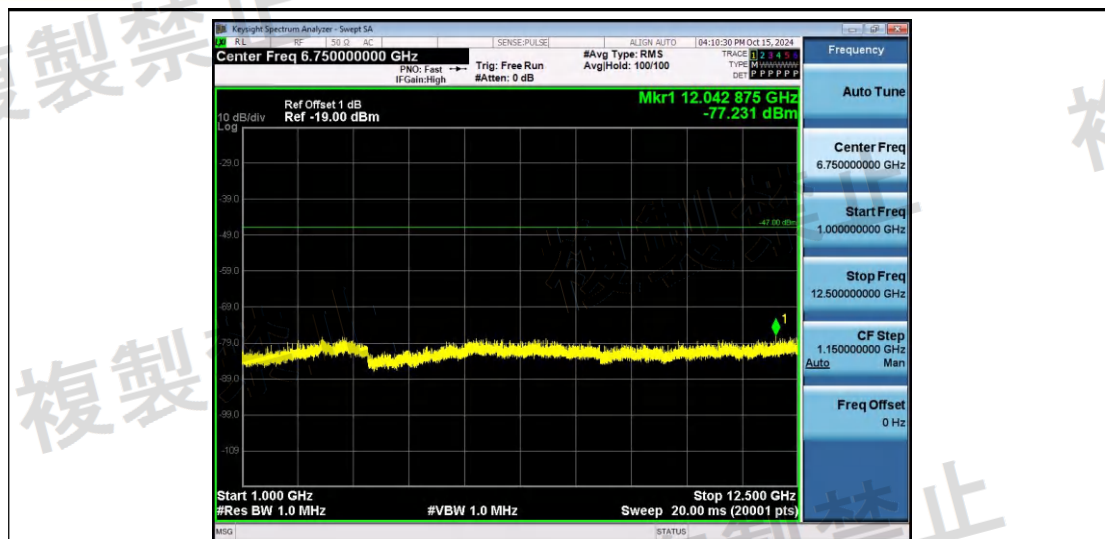
NTNV-11B-Ant1-2442-1000~12500-PASS
