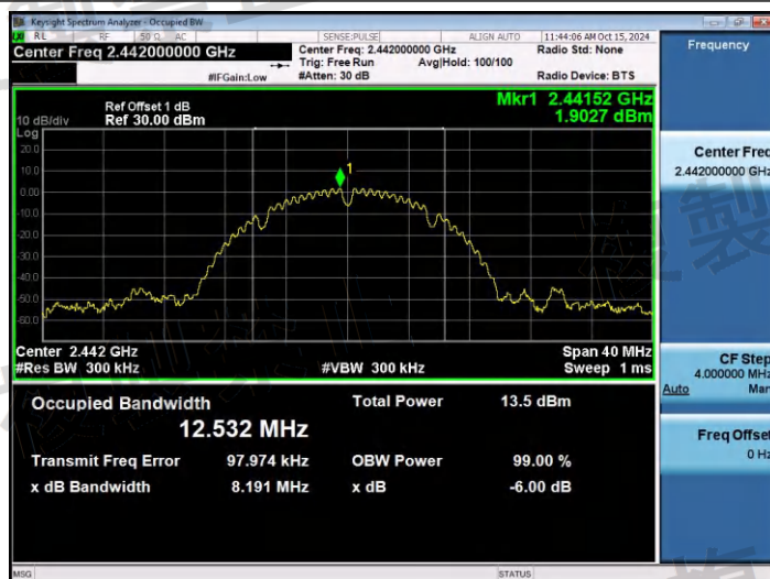
NTNV-11B-Ant1-2442-PASS
