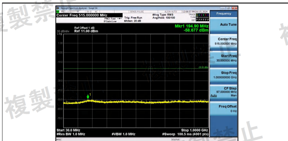
NTNV-11AX40SISO-Ant1-2422-30~1000-PASS
