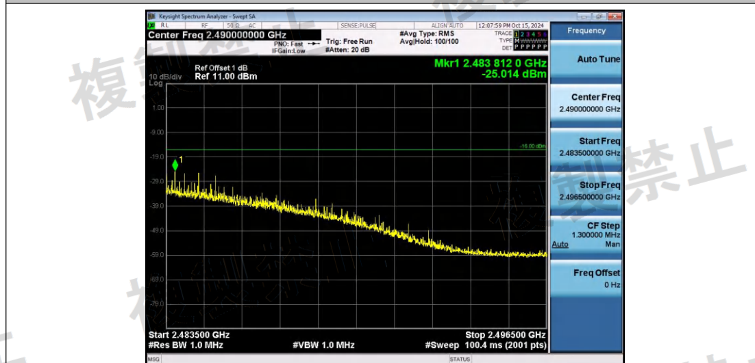
NTNV-11AX20SISO-Ant1-2472-2483.5~2496.5-PASS
