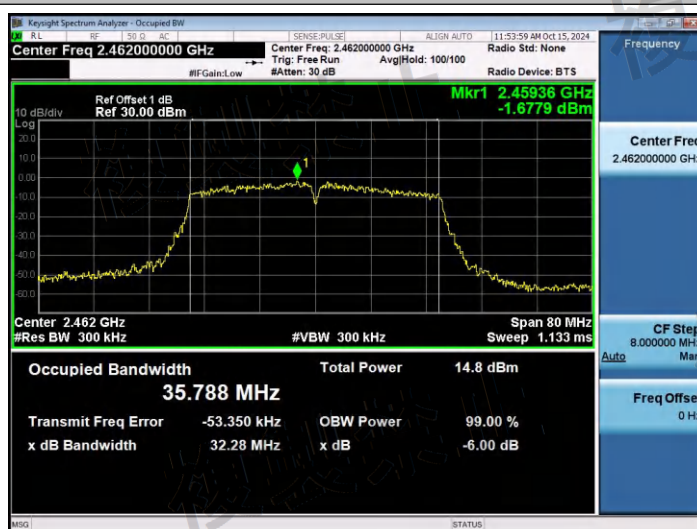
NTNV-11N40SISO-Ant1-2462-PASS
