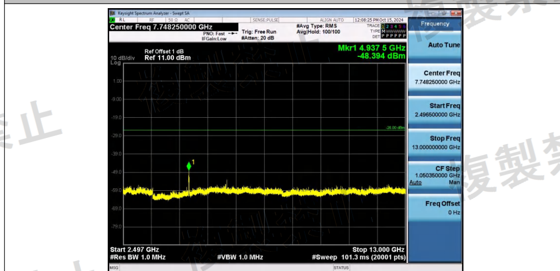
NTNV-11AX20SISO-Ant1-2472-2496.5~13000-PASS
