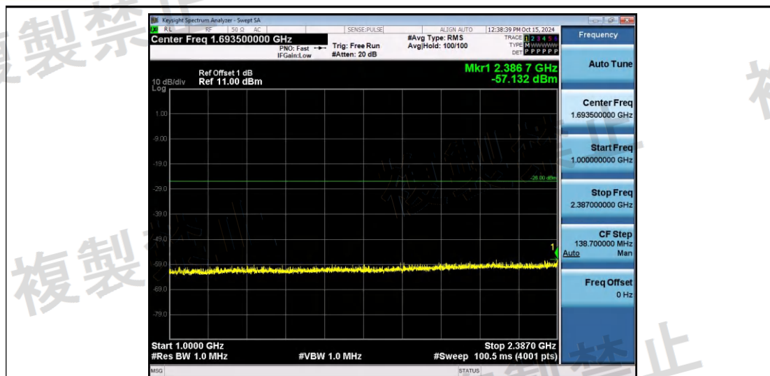
NTVN-11N40SISO-Ant1-2442-1000~2387-PASS
