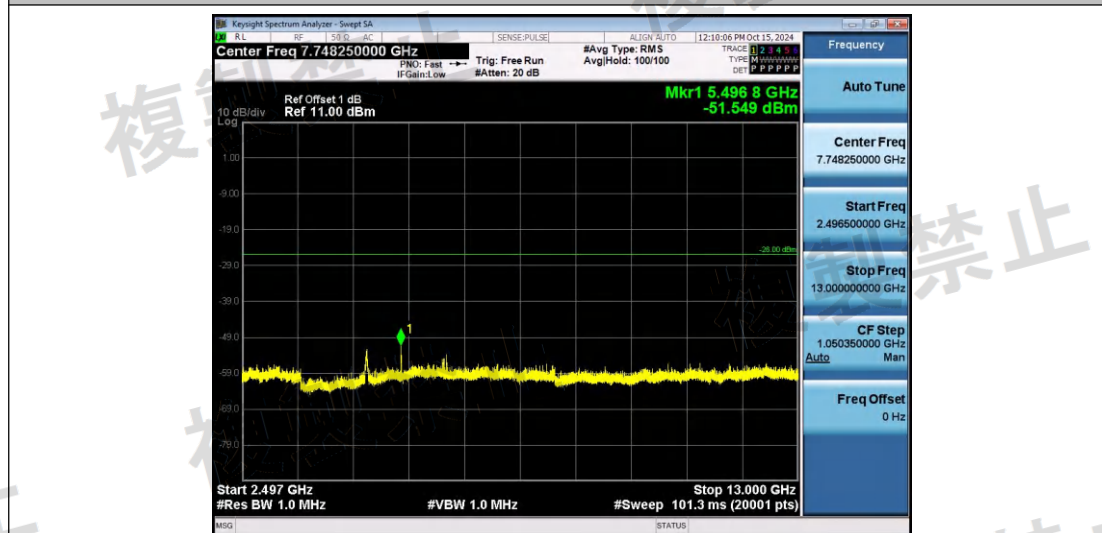
NTNV-11AX40SISO-Ant1-2422-2496.5~13000-PASS
