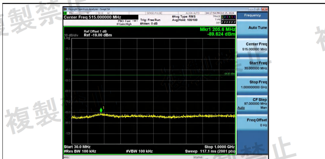
NTNV-11AX20SISO-Ant1-2412-30~1000-PASS
