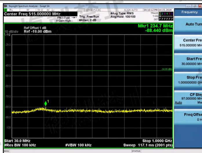
NTNV-11B-Ant1-2442-30~1000-PASS
