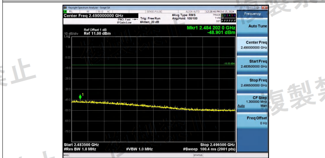
NTNV-11G-Ant1-2442-2483.5~2496.5-PASS
