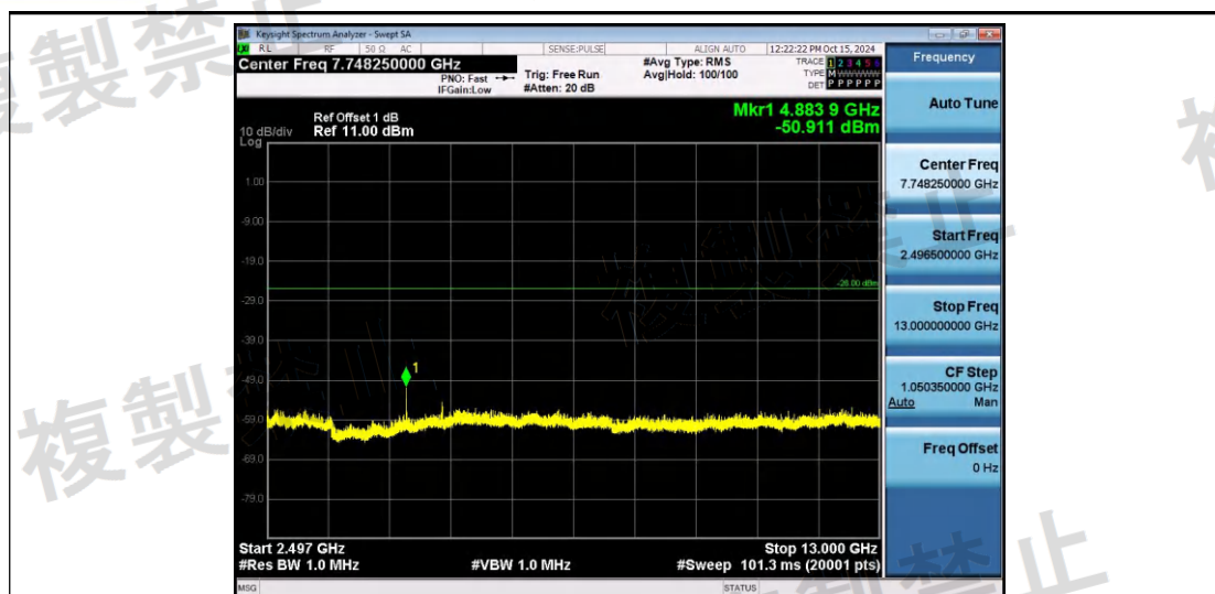
NTNV-11B-Ant1-2442-2496.5~13000-PASS
