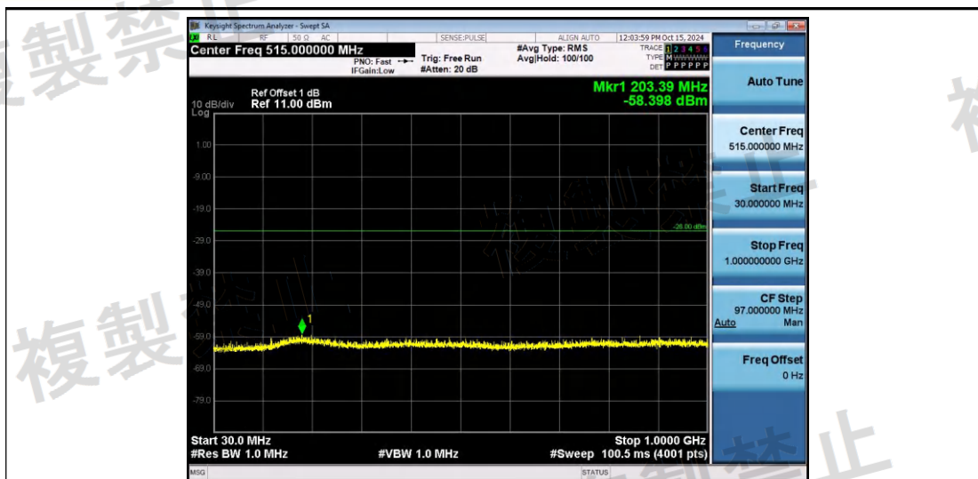
NTNV-11AX20SISO-Ant1-2412-30~1000-PASS
