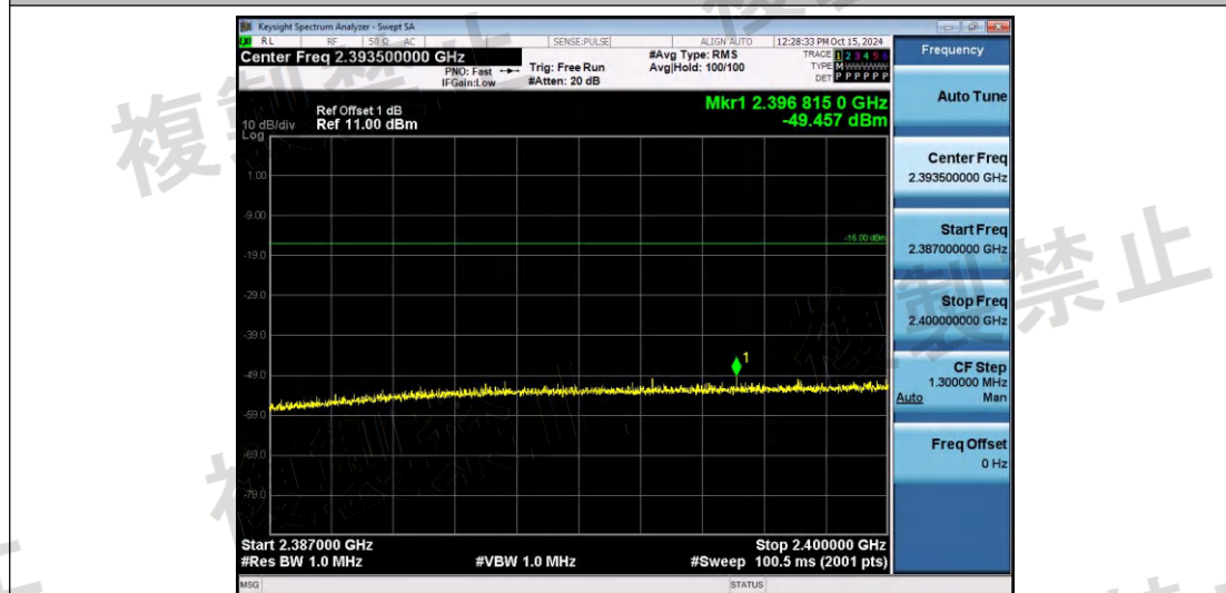
NTNV-11G-Ant1-2442-2387~2400-PASS
