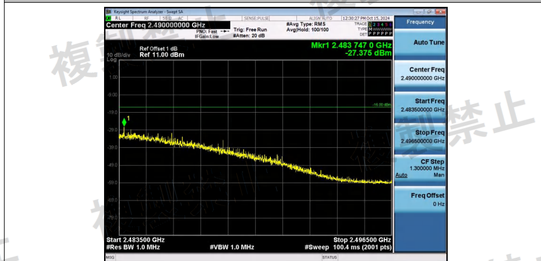
NTNV-11G-Ant1-2472-2483.5~2496.5-PASS
