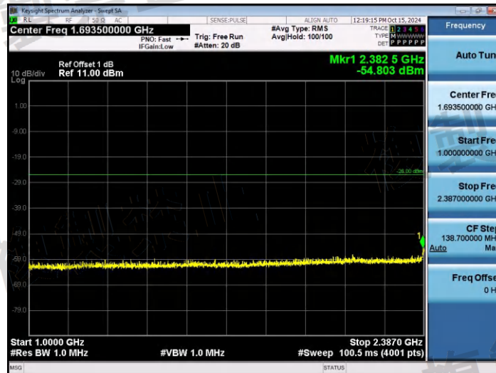
NTNV-11B-Ant1-2412-1000~2387-PASS
