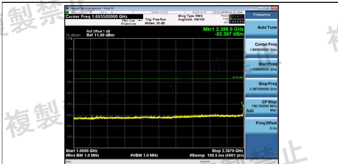
NTNV-11B-Ant1-2442-1000~2387-PASS
