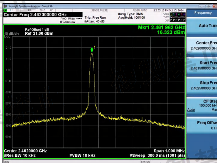
NTVN-CW-Ant1-2462-PASS
