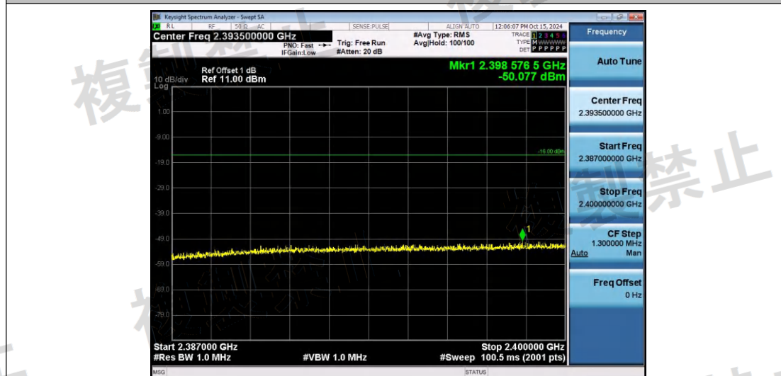
NTNV-11AX20SISO-Ant1-2442-2387~2400-PASS
