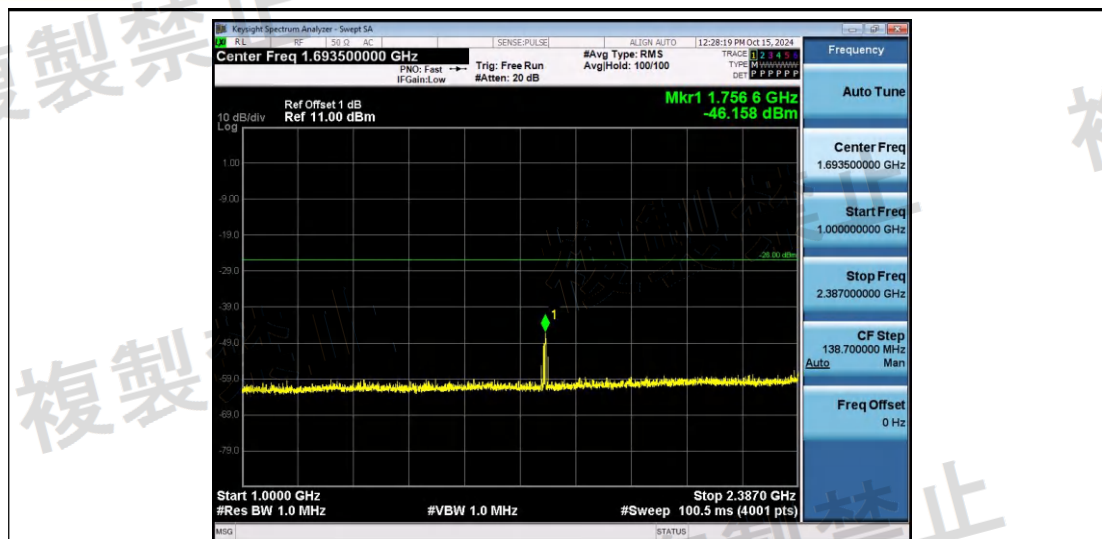
NTNV-11G-Ant1-2442-1000~2387-PASS
