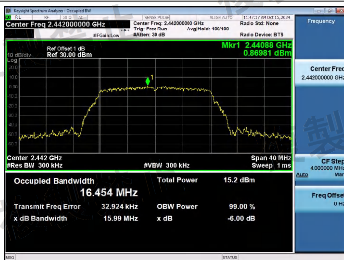
NTNV-11G-Ant1-2442-PASS
