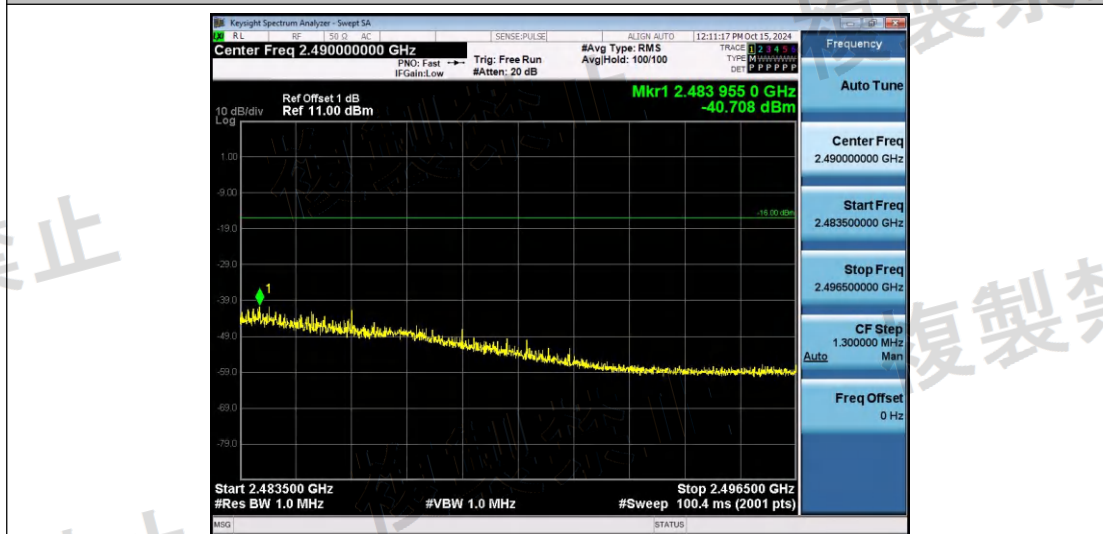
NTNV-11AX40SISO-Ant1-2442-2483.5~2496.5-PASS
