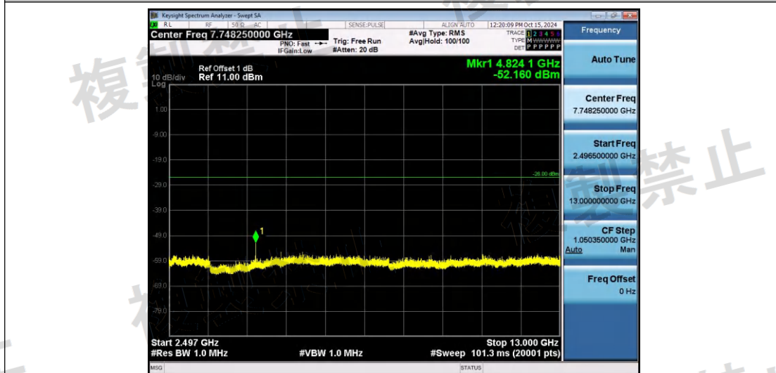
NTNV-11B-Ant1-2412-2496.5~13000-PASS
