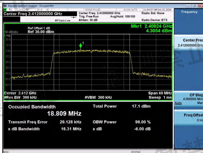
NTNV-11AX20SISO-Ant1-2412-PASS
