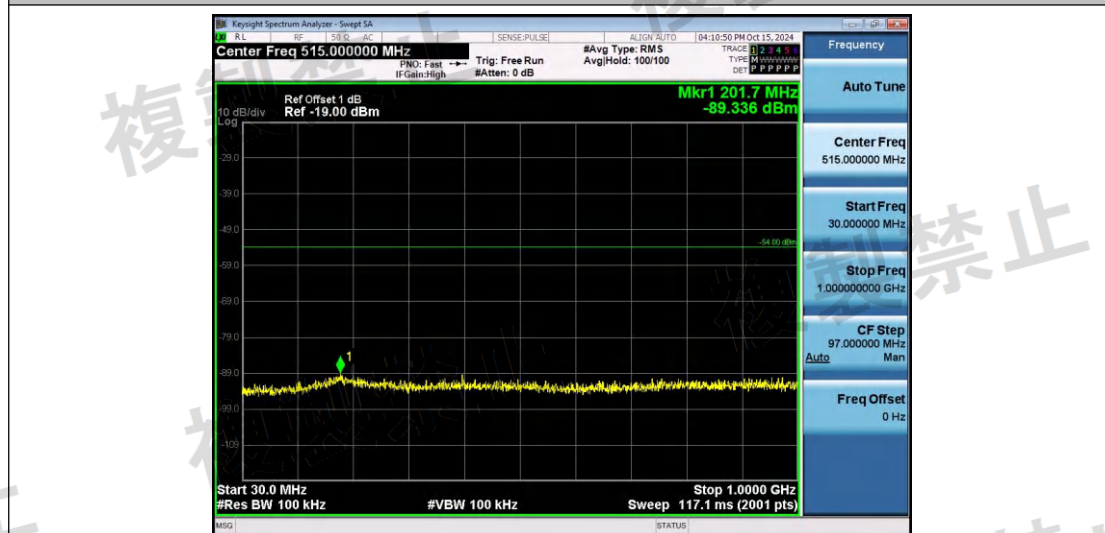
NTNV-11B-Ant1-2472-30~1000-PASS
