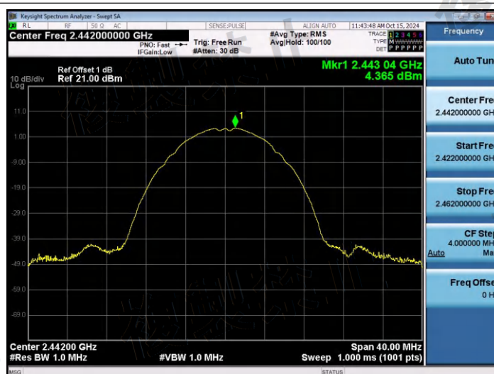
NTNV-11B-Ant1-2442-PASS
