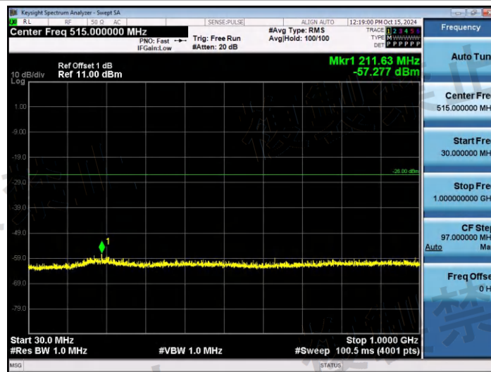
NTNV-11B-Ant1-2412-30~1000-PASS
