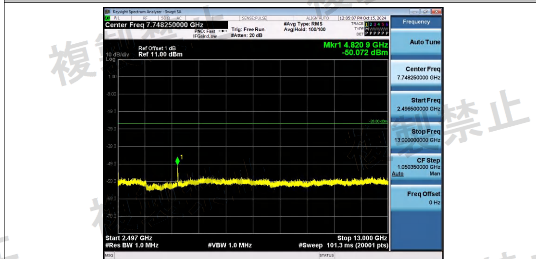
NTNV-11AX20SISO-Ant1-2412-2496.5~13000-PASS
