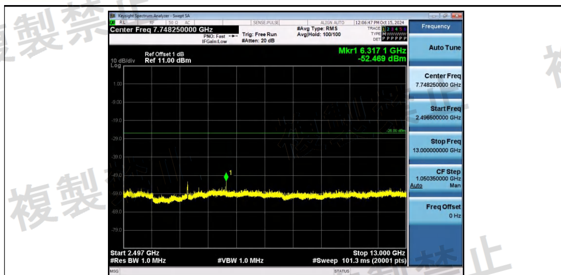
NTNV-11AX20SISO-Ant1-2442-2496.5~13000-PASS
