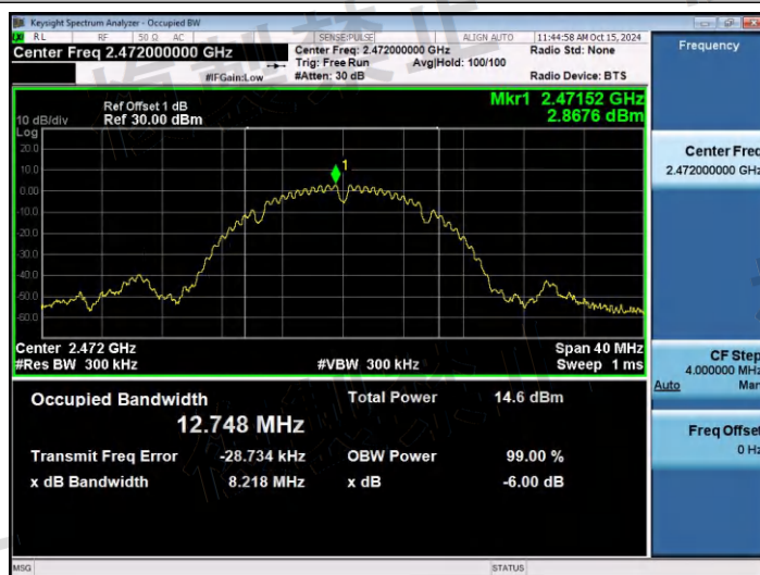
NTNV-11B-Ant1-2472-PASS
