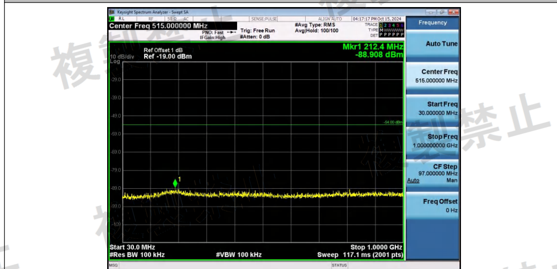
NTNV-11N40SISO-Ant1-2462-30~1000-PASS
