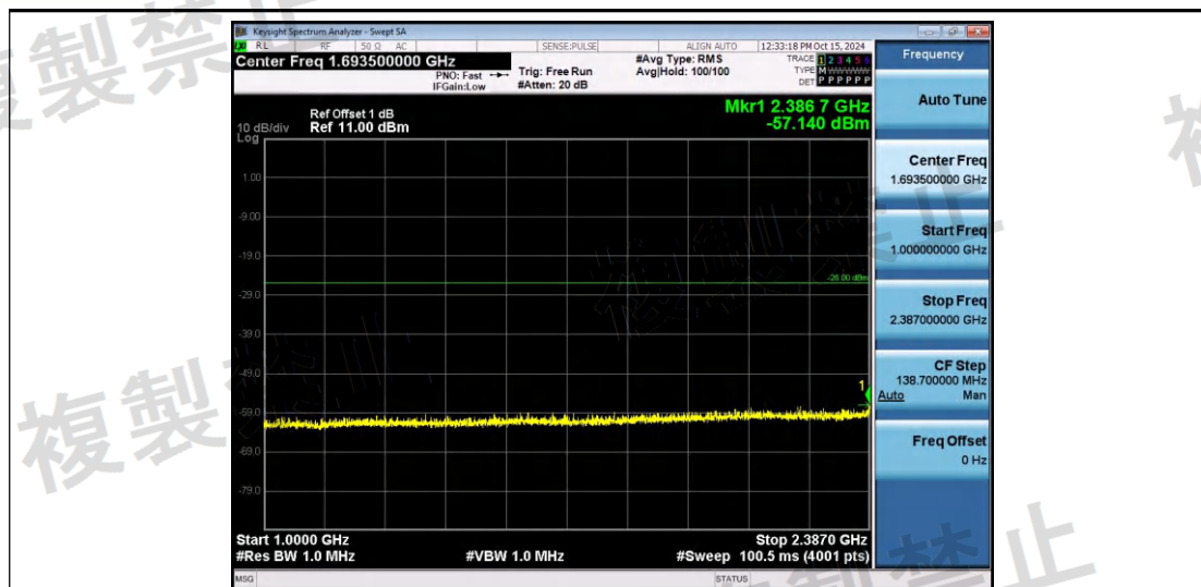
NTVN-11N20SISO-Ant1-2442-1000~2387-PASS
