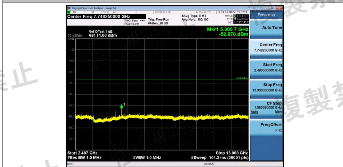
NTNV-11B-Ant1-2472-2496.5~13000-PASS
