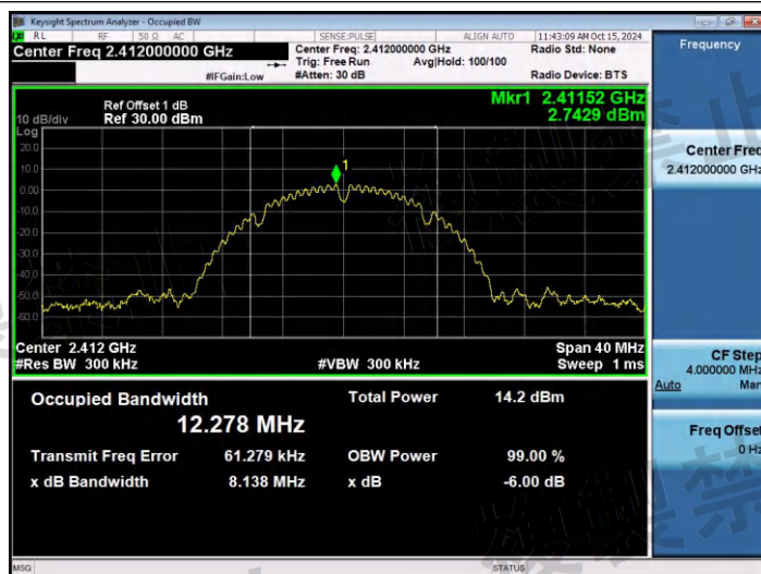
NTNV-11B-Ant1-2412-PASS
