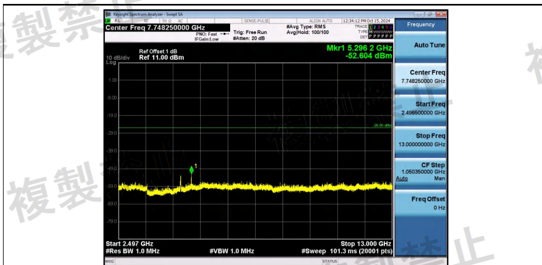
NTNV-11N20SISO-Ant1-2442-2496.5~13000-PASS
