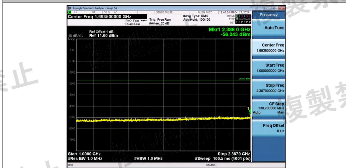
NTNV-11N40SISO-Ant1-2462-1000~2387-PASS
