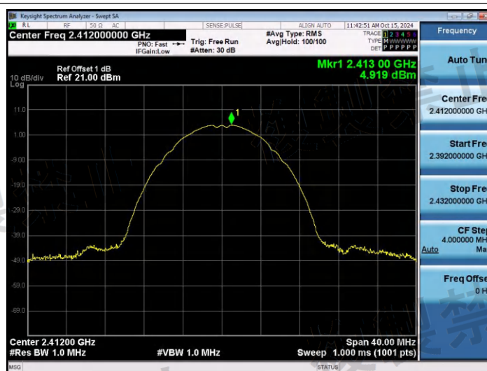
NTNV-11B-Ant1-2412-PASS
