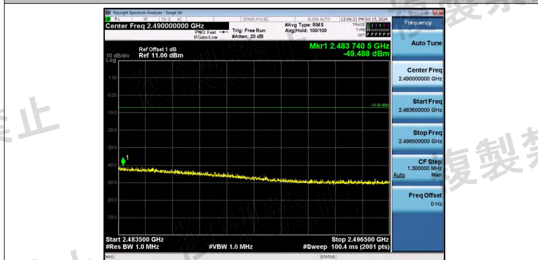
NTNV-11AX20SISO-Ant1-2442-2483.5~2496.5-PASS
