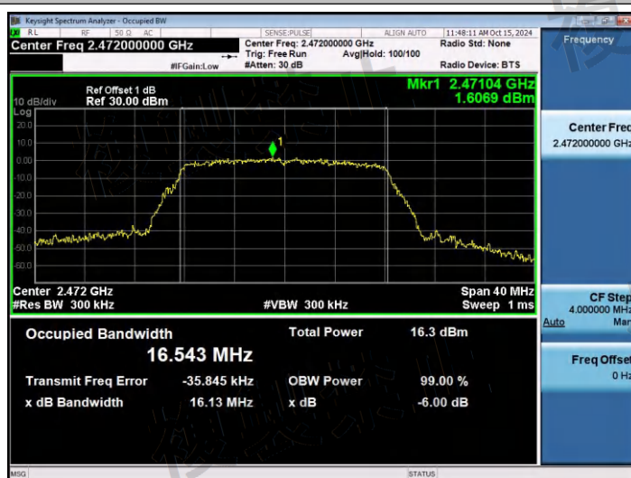
NTNV-11G-Ant1-2472-PASS
