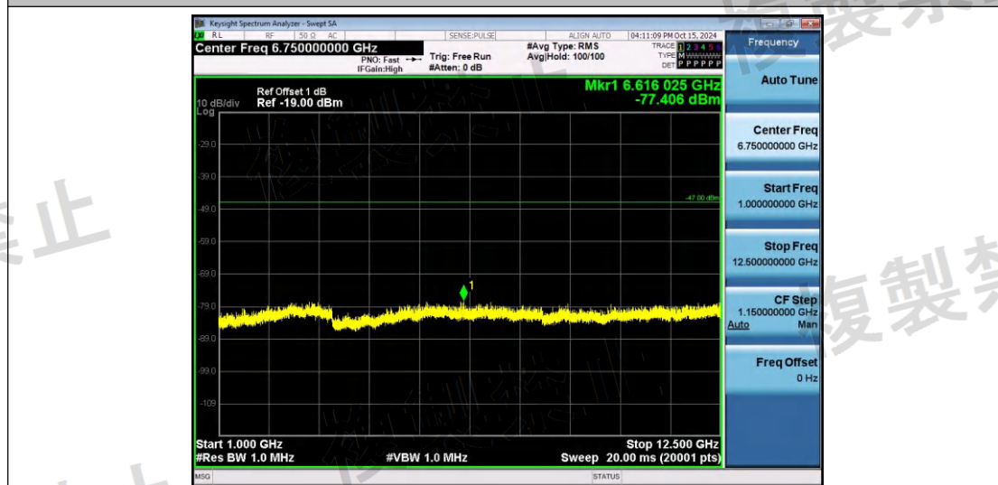
NTNV-11B-Ant1-2472-1000~12500-PASS
