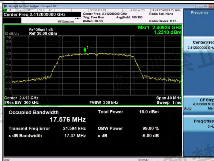
NTNV-11N20SISO-Ant1-2412-PASS
