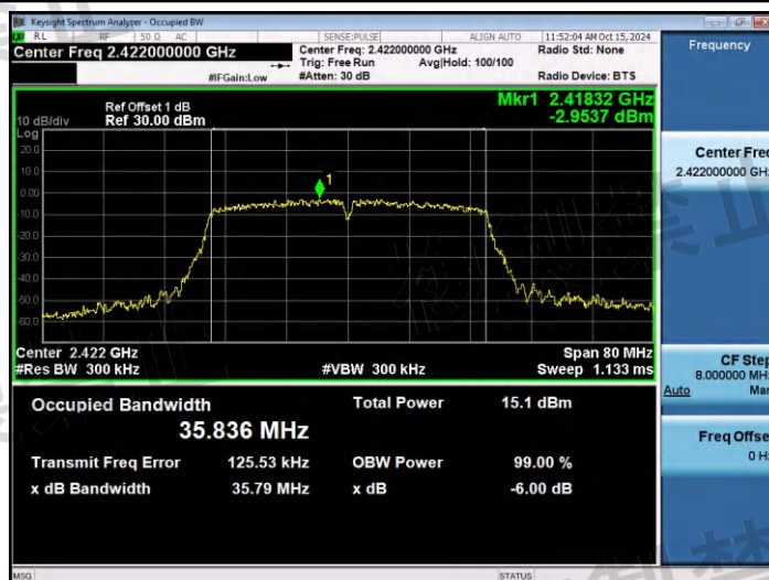
NTNV-11N40SISO-Ant1-2422-PASS
