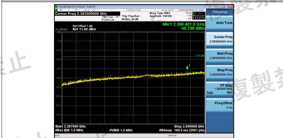
NTNV-11AX20SISO-Ant1-2412-2387~2400-PASS
