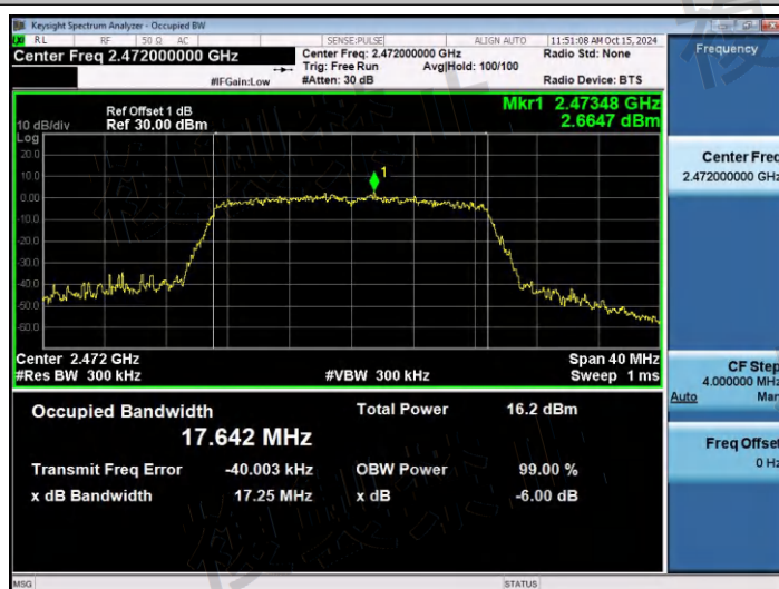
NTNV-11N20SISO-Ant1-2472-PASS
