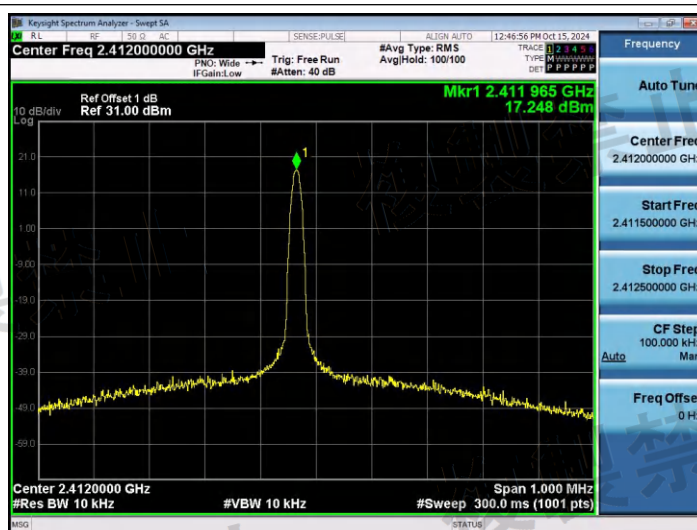
NTNV-CW-Ant1-2412-PASS
