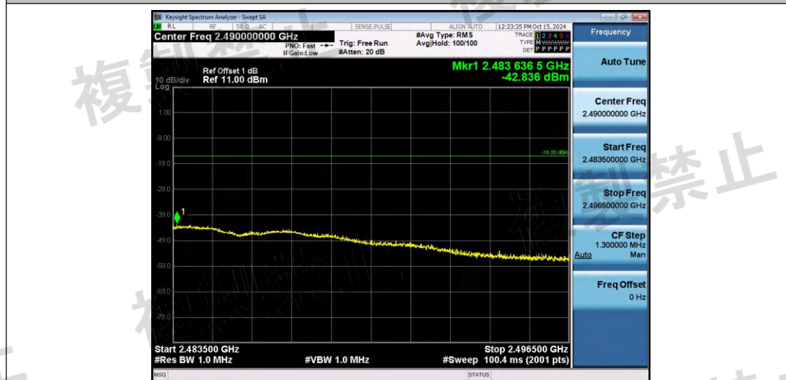
NTNV-11B-Ant1-2472-2483.5~2496.5-PASS
