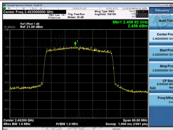
NTNV-11AX40SISO-Ant1-2462-PASS
