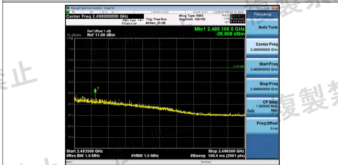
NTVN-11N40SISO-Ant1-2442-2483.5~2496.5-PASS
