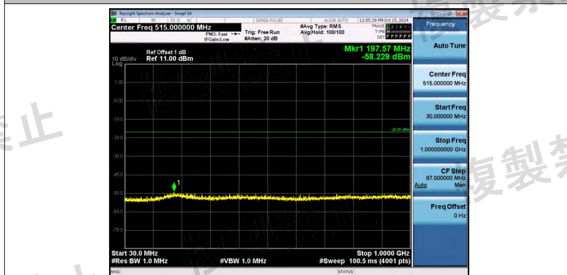
NTNV-11AX20SISO-Ant1-2442-30~1000-PASS
