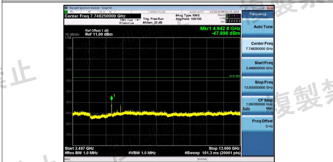
NTNV-11N20SISO-Ant1-2472-2496.5~13000-PASS
