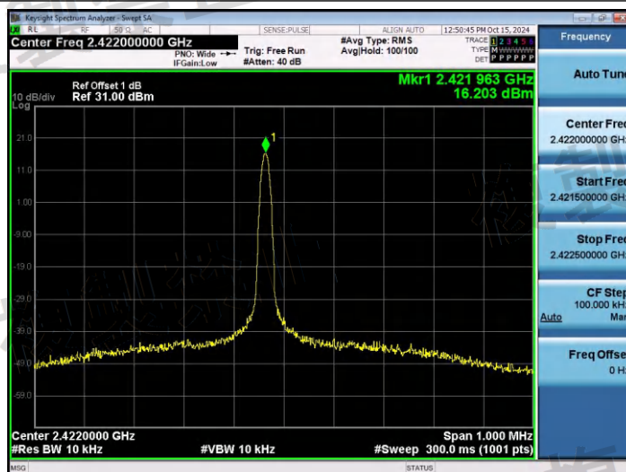
NTNV-CW-Ant1-2422-PASS
