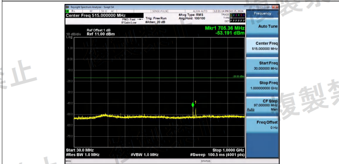
NTNV-11B-Ant1-2442-30~1000-PASS
