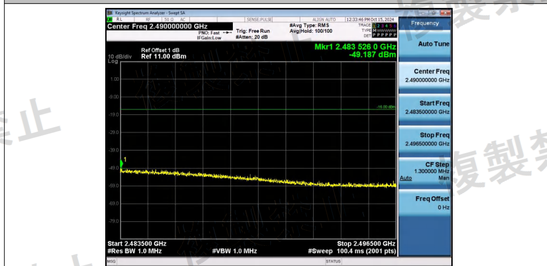
NTVN-11N20SISO-Ant1-2442-2483.5~2496.5-PASS
