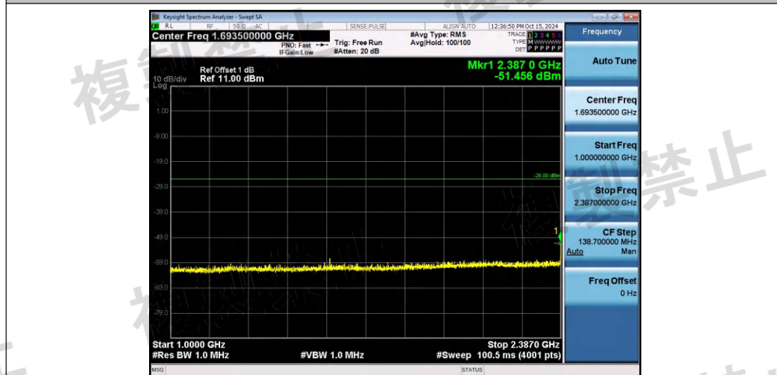
NTNV-11N40SISO-Ant1-2422-1000~2387-PASS
