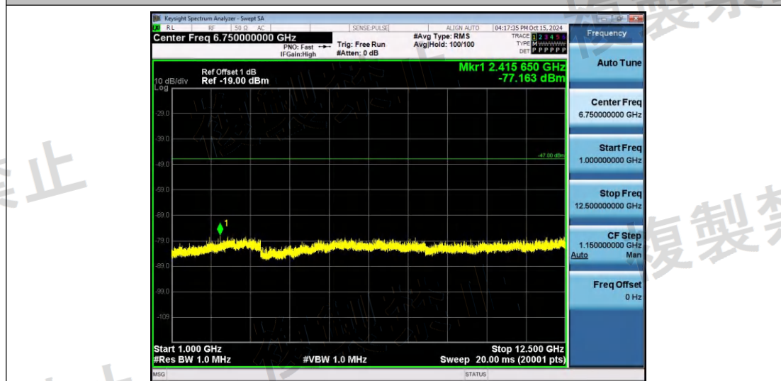
NTNV-11N40SISO-Ant1-2462-1000~12500-PASS
