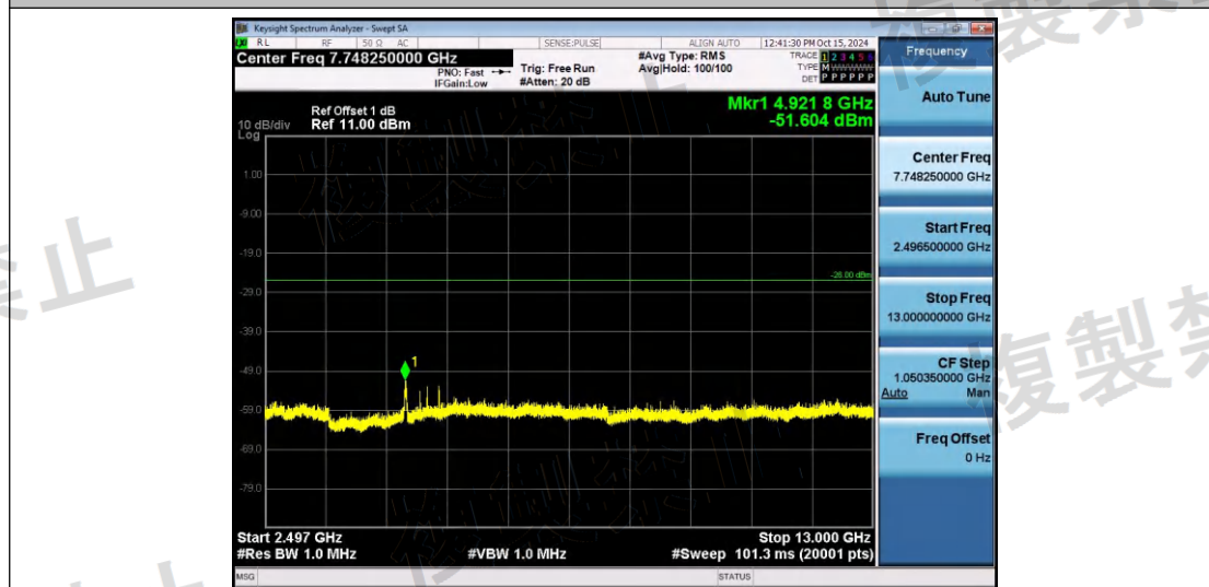
NTNV-11N40SISO-Ant1-2462-2496.5~13000-PASS
