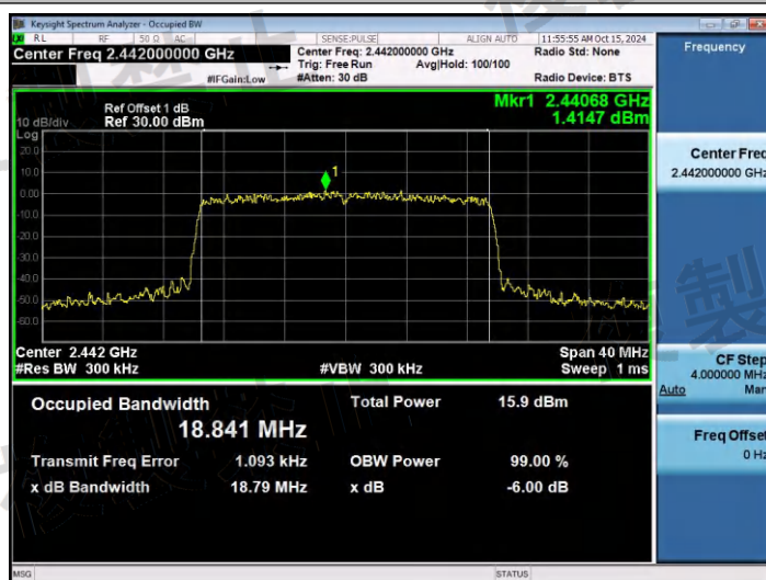
NTNV-11AX20SISO-Ant1-2442-PASS
