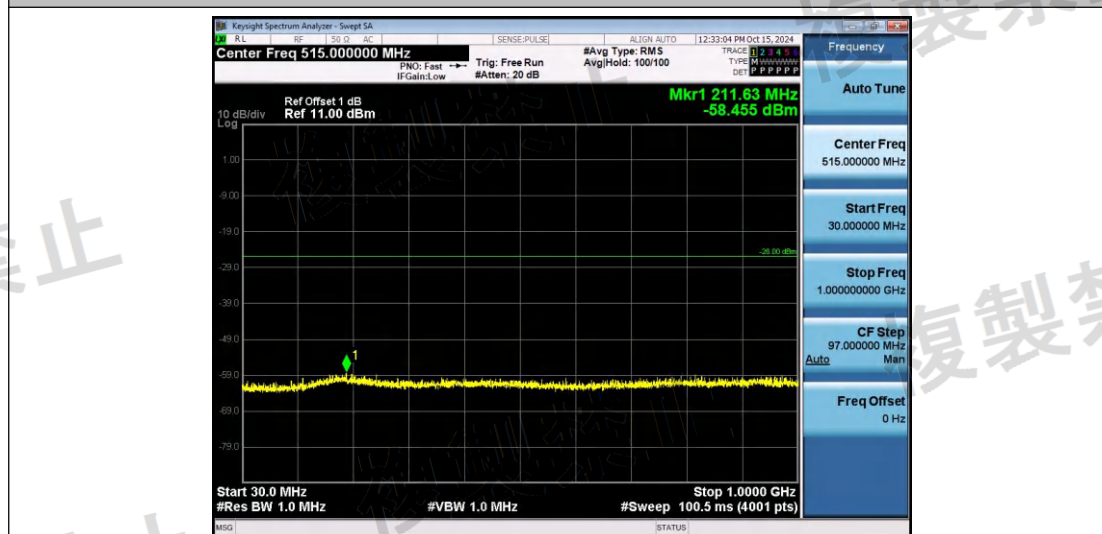
NTNV-11N20SISO-Ant1-2442-30~1000-PASS
