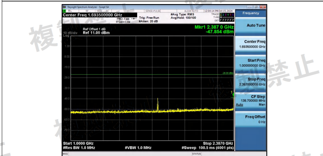
NTNV-11AX20SISO-Ant1-2412-1000~2387-PASS
