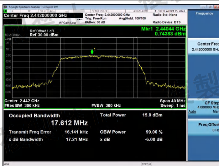
NTNV-11N20SISO-Ant1-2442-PASS
