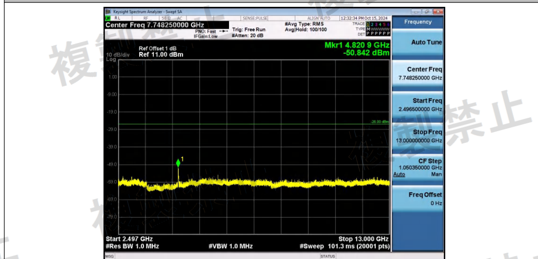
NTNV-11N20SISO-Ant1-2412-2496.5~13000-PASS
