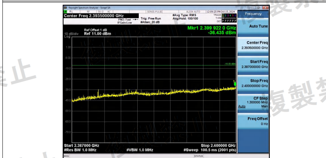
NTNV-11AX40SISO-Ant1-2422-2387~2400-PASS
