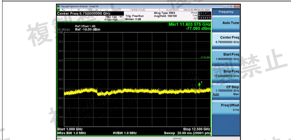
NTNV-11G-Ant1-2412-1000~12500-PASS
