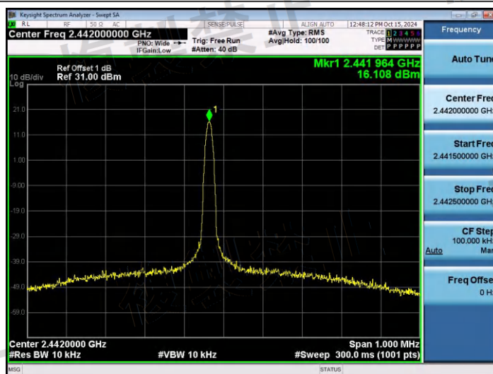
NTNV-CW-Ant1-2442-PASS
