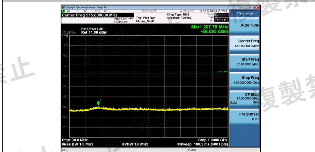
NTNV-11N40SISO-Ant1-2442-30~1000-PASS
