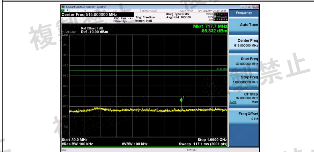
NTNV-11AX20SISO-Ant1-2472-30~1000-PASS
