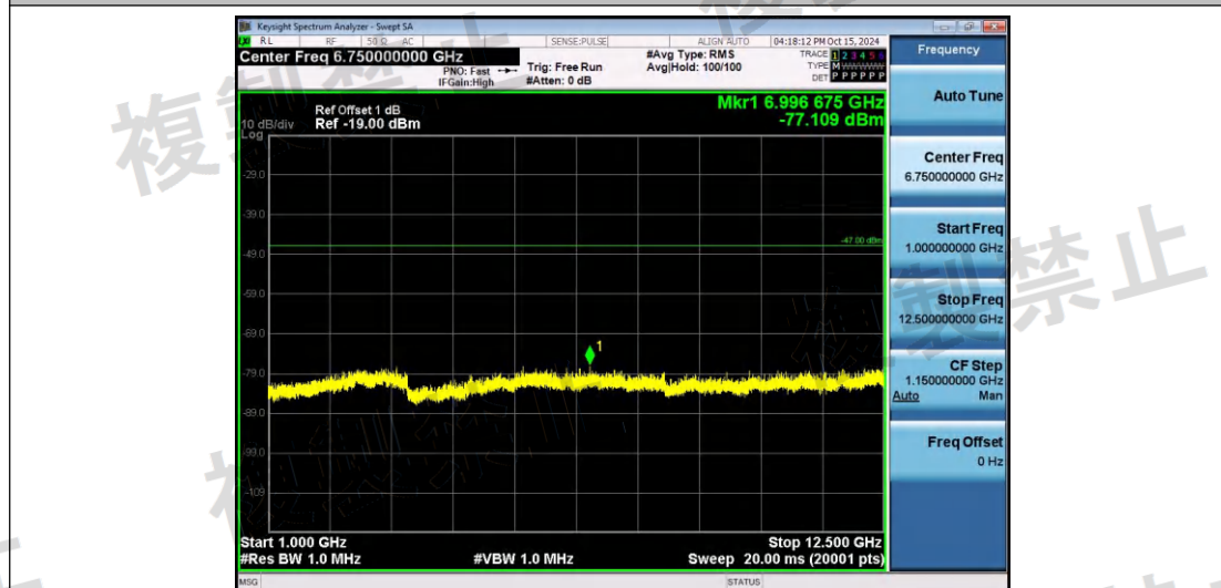
NTNV-11AX20SISO-Ant1-2412-1000~12500-PASS
