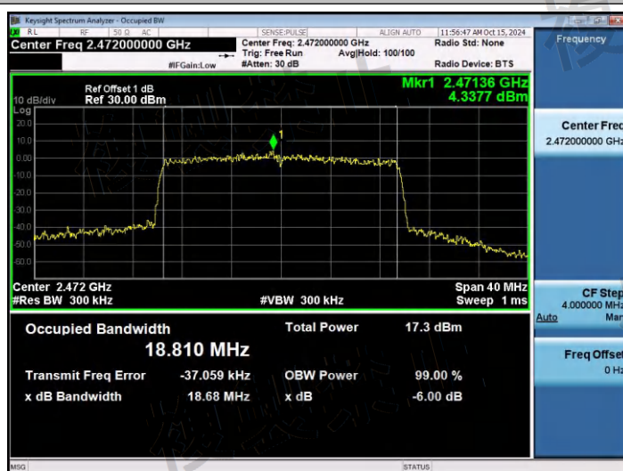
NTNV-11AX20SISO-Ant1-2472-PASS
