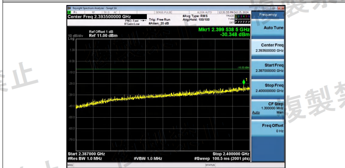
NTNV-11N20SISO-Ant1-2412-2387~2400-PASS
