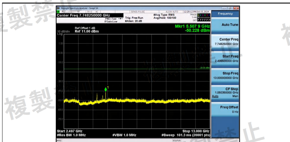
NTNV-11G-Ant1-2442-2496.5~13000-PASS
