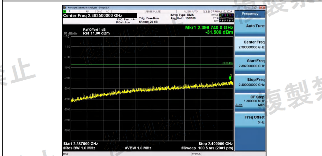
NTNV-11G-Ant1-2412-2387~2400-PASS
