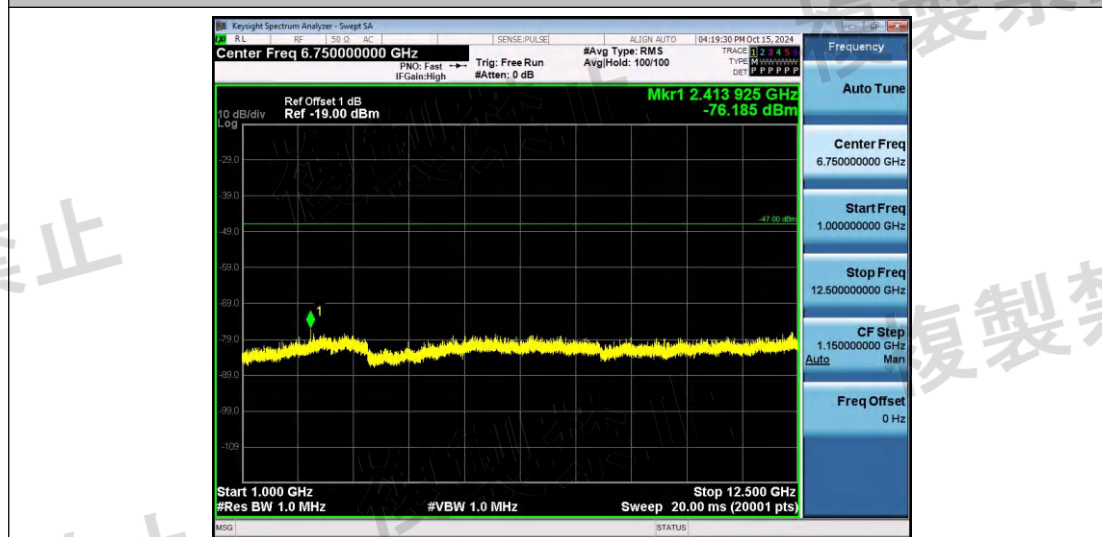
NTNV-11AX20SISO-Ant1-2472-1000~12500-PASS
