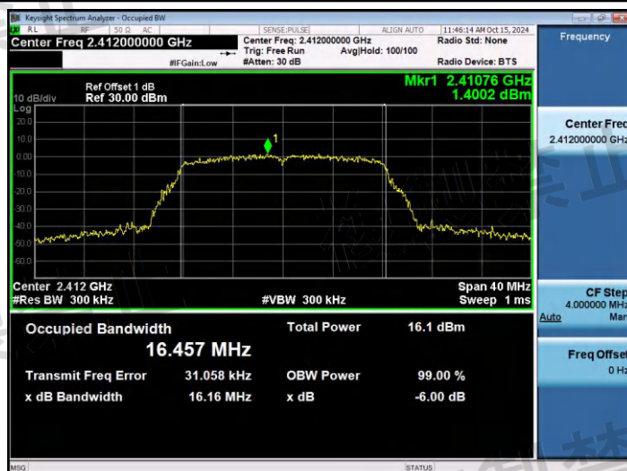
NTNV-11G-Ant1-2412-PASS
