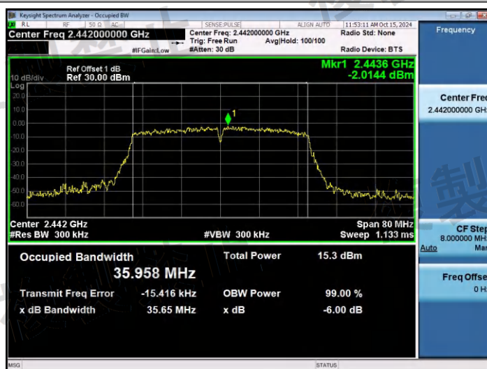
NTNV-11N40SISO-Ant1-2442-PASS
