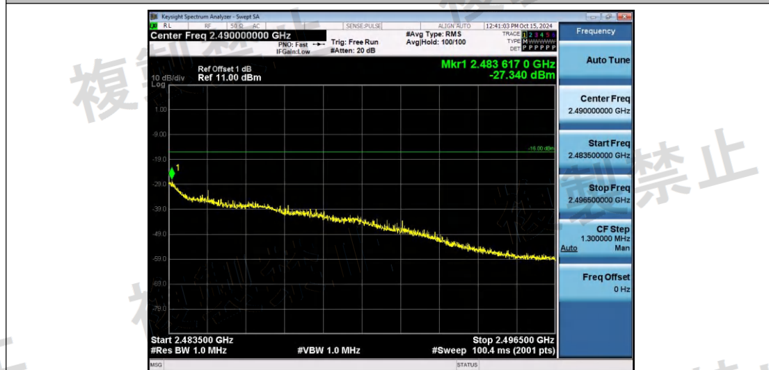
NTNV-11N40SISO-Ant1-2462-2483.5~2496.5-PASS
