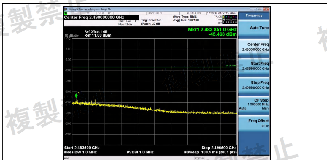
NTNV-11AX40SISO-Ant1-2422-2483.5~2496.5-PASS
