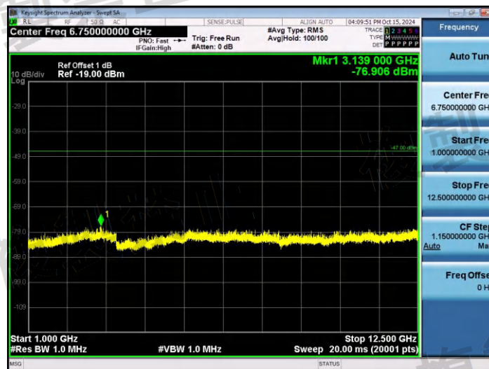
NTNV-11B-Ant1-2412-1000~12500-PASS
