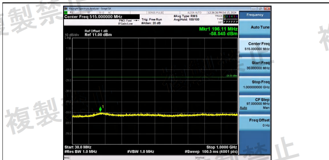
NTNV-11N40SISO-Ant1-2422-30~1000-PASS
