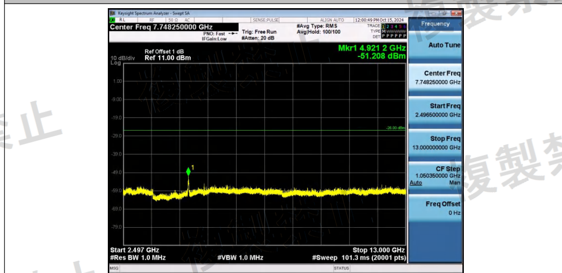
NTNV-11AX40SISO-Ant1-2462-2496.5~13000-PASS
