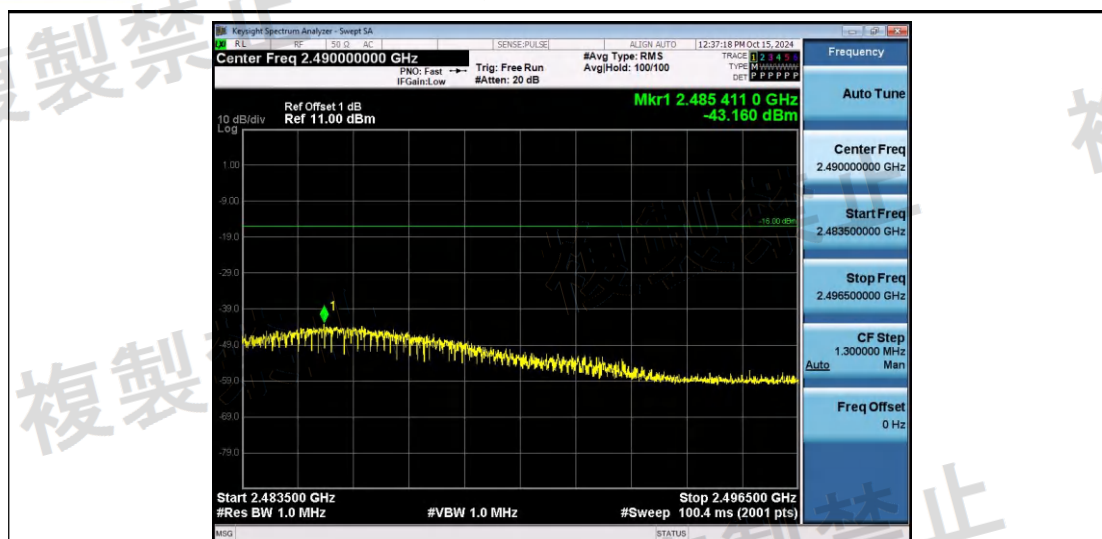
NTNV-11N40SISO-Ant1-2422-2483.5~2496.5-PASS
