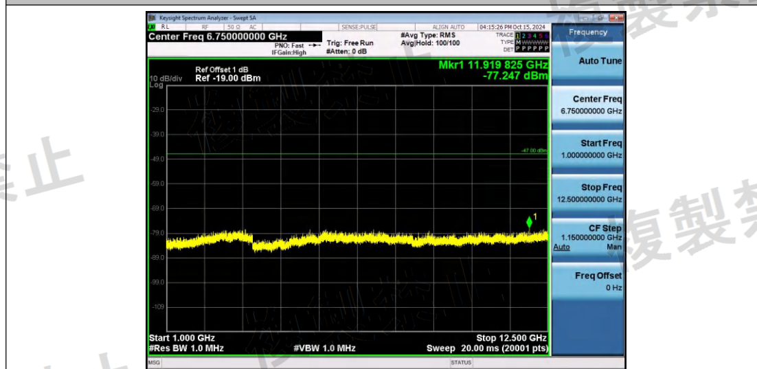
NTNV-11N20SISO-Ant1-2472-1000~12500-PASS
