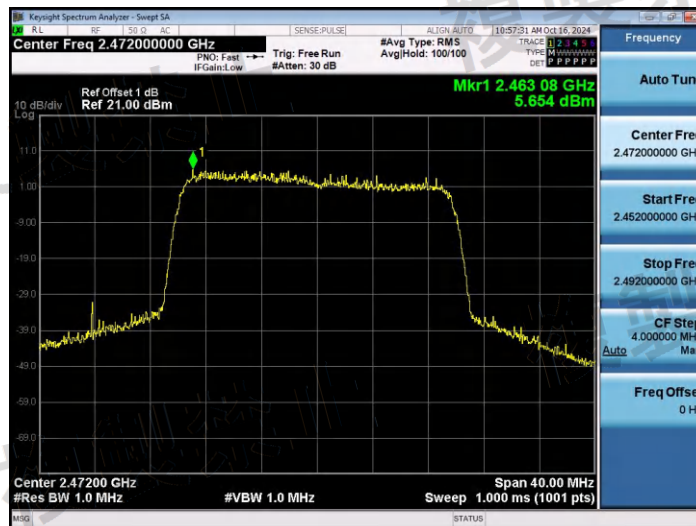
NTNV-11AX20SISO-Ant1-2472-PASS
