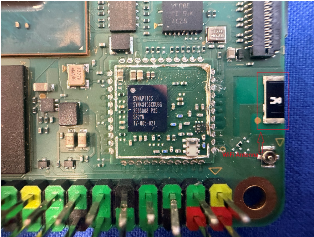
Photo 7: Internal View for WiFi Antenna
