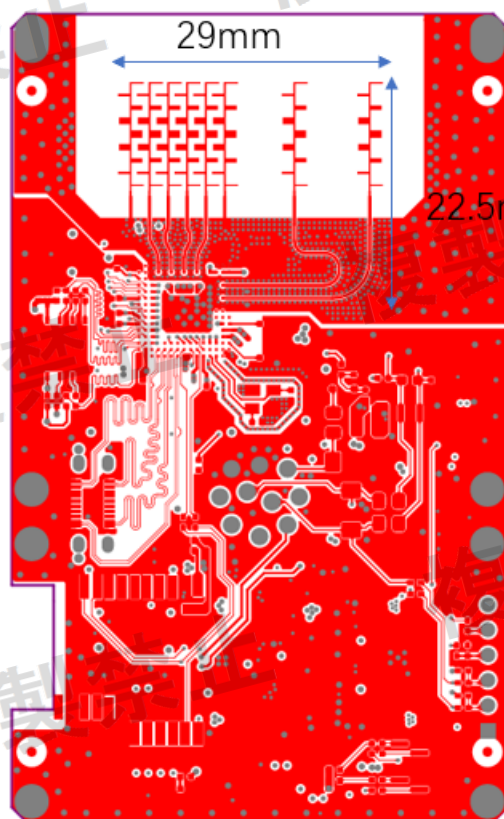
Antenna Size
