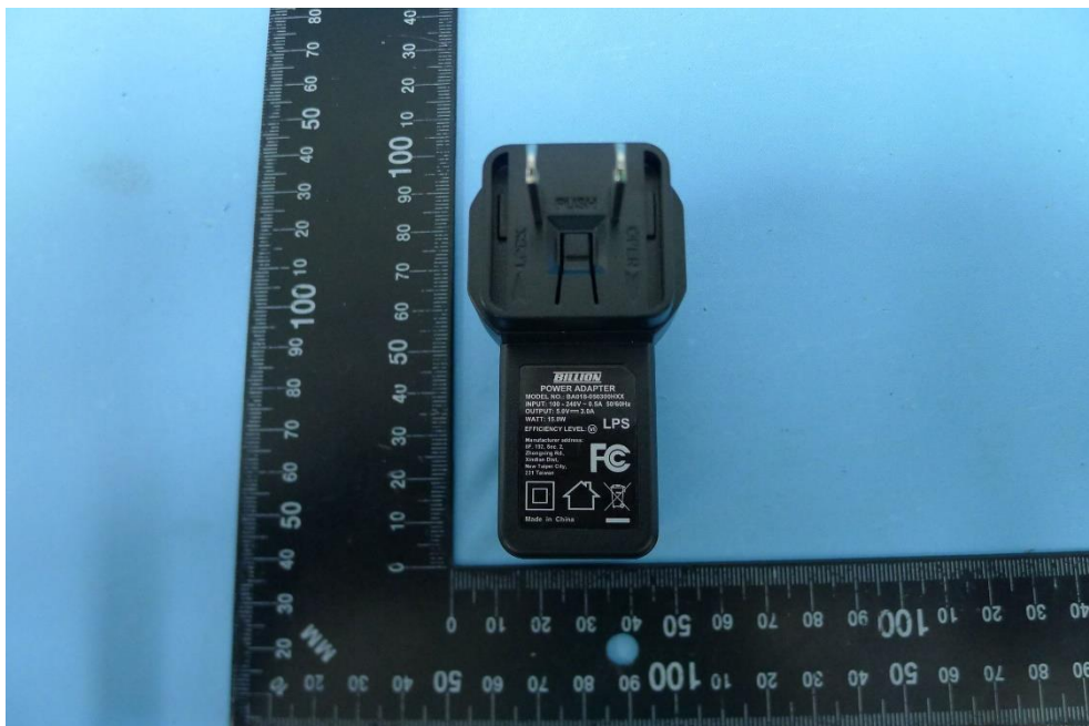
(16) Adapter Photo
