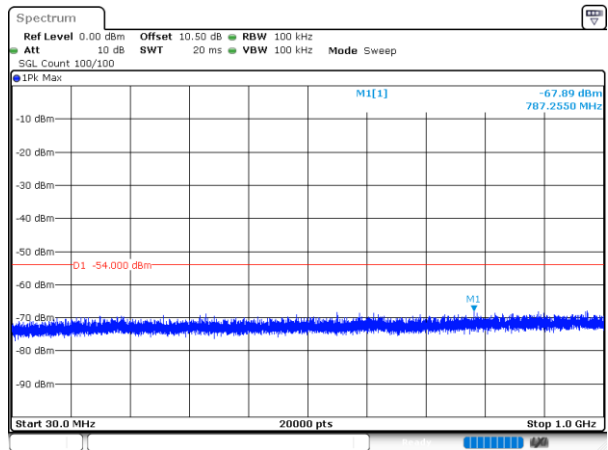
BLE 1M_High Channel(30MHz~1GHz)
