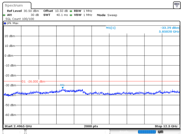
BLE 1M_Low Channel(2.4965GHz~12.5GHz)
