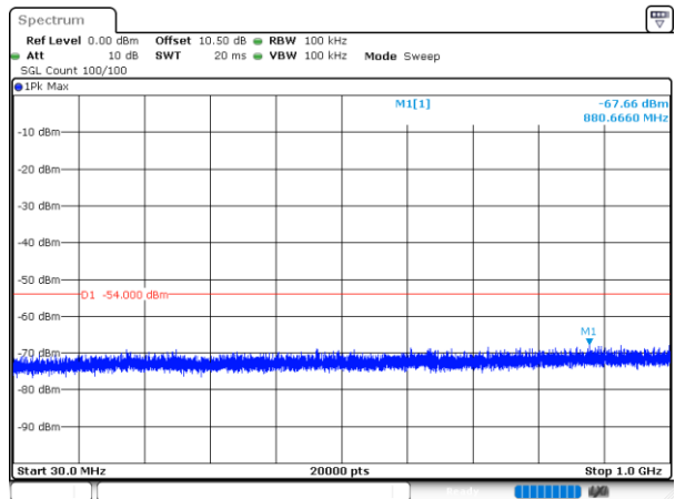
BLE 1M_Middle Channel(30MHz~1GHz)
