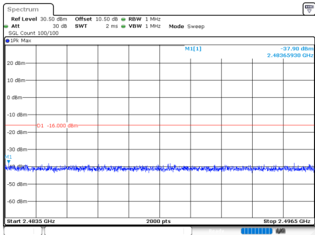
BLE 1M_High Channel(2.4835GHz~2.4965GHz)
